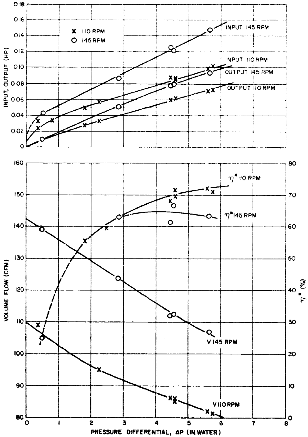
FIG. 13. BLOWER PERFORMANCE WITH SURGETANK
