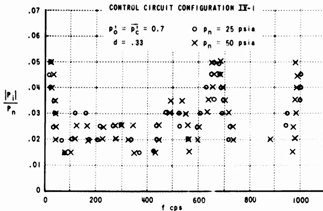
Figure 24 SWITCHING PERFORMANCE DATA AT DIFFERENT POWER NOZZLE SUPPLY PRESSURES INDICATING SUITABILITY OF METHOD CHOSEN TO NONDIMENSIONALIZE PRESSURE PARAMETERS.
