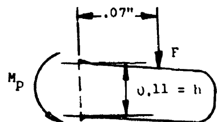
Figure 9. Track-Channel Free Body.
