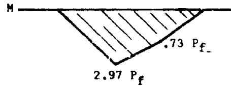
Figure 19. Bending Shear and Load Diagrams for Aft Legs.
