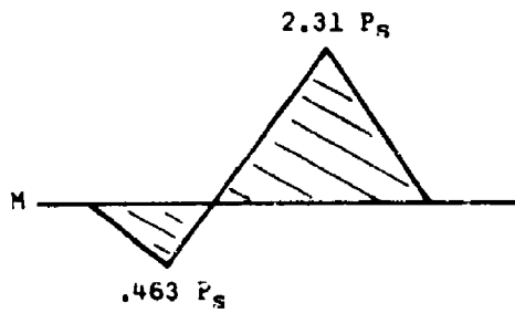
Figure 19. Bending Shear and Load Diagrams for Aft Legs.
