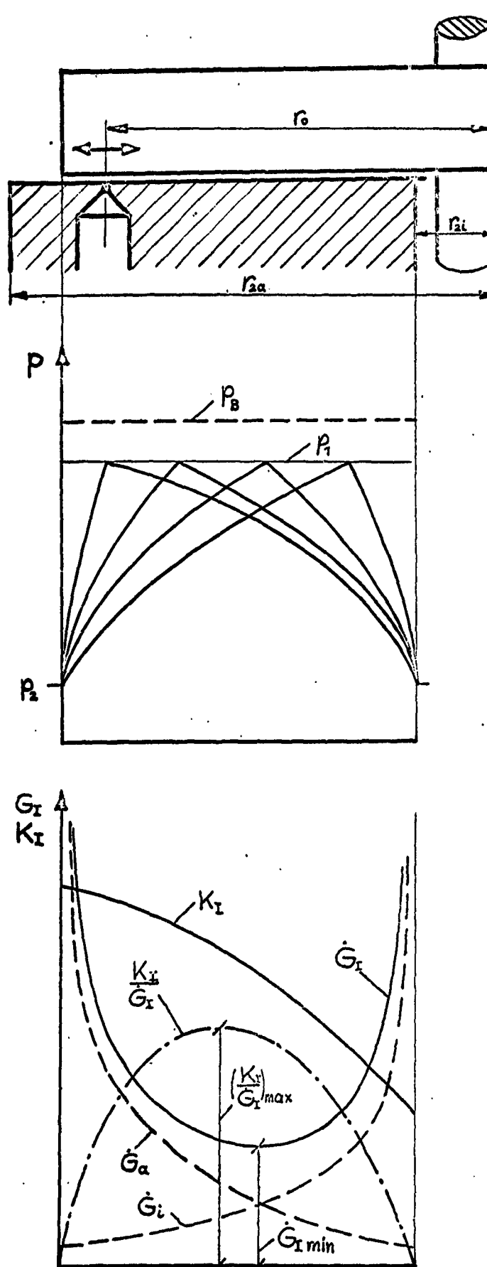
Gas consumption and load capacity as function of the gas inlet radius r_0
