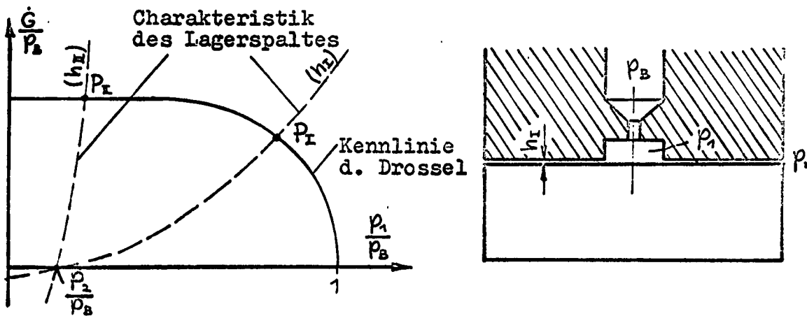
(top) characteristic of the bearing clearance - (bottom) characteristic of the throttle
