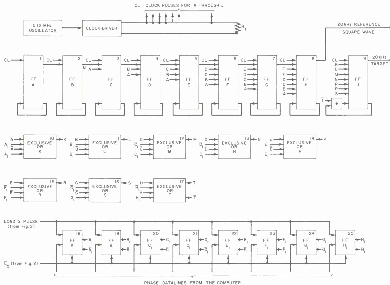
Fig. 10. Phaseshift generator digital circuits.
