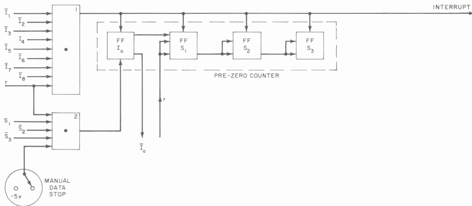
Fig. 7. Interrupt generation.
