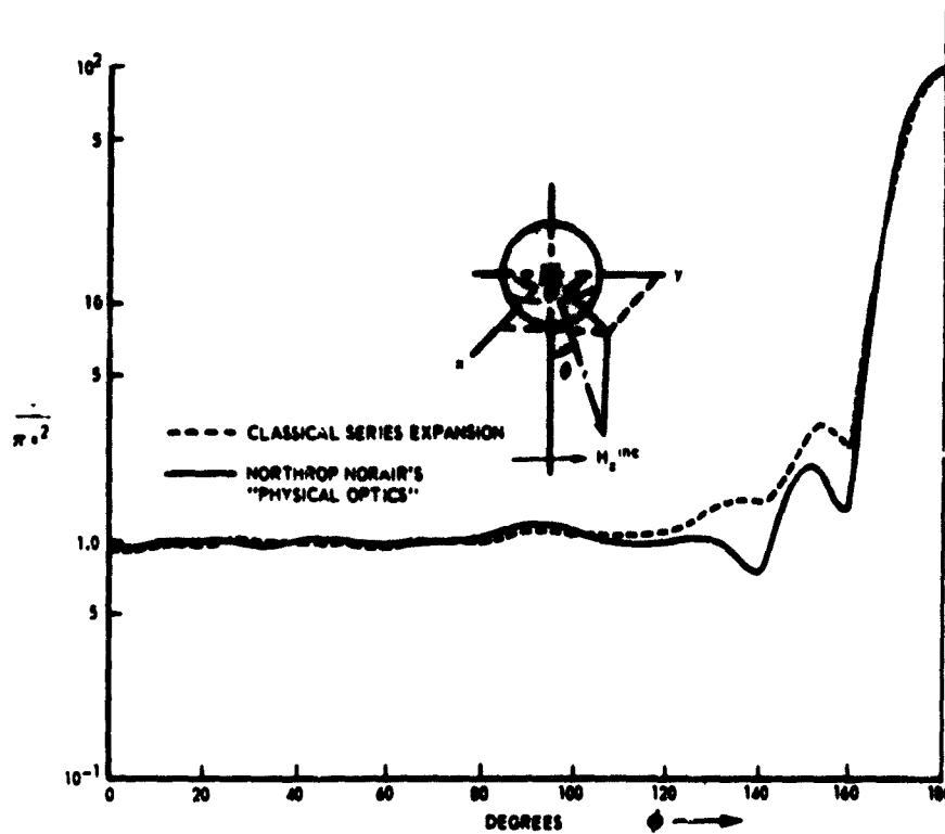
FIGURE 19 BISTATIC CROSS-SECTION FOR PERFECTLY CONDUCTING SPHERE ( ka = 10 ) H-PLANE
