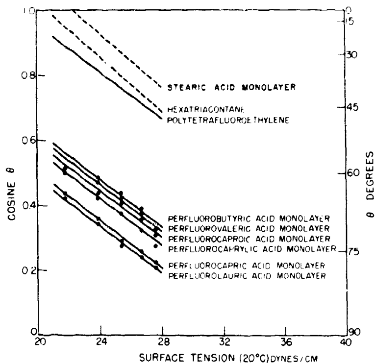
Fig. 6 - Comparison of \gamma_{LV} vs \cos \theta relationships for a series of n-alkanes on several different low energy surfaces
