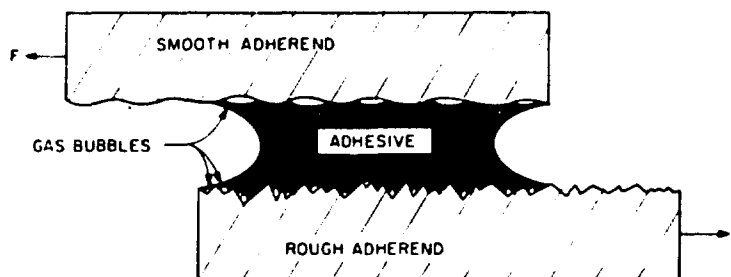
Fig. 22 - Effect of surface roughness on coplanarity of gas bubbles
