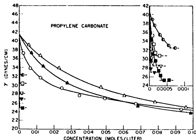
Fig. 18 - Surface tensions of partially fluorinated compounds in propylene carbonate: \Delta , 1H,1H-pentadecafluorooctyl alcohol; \blacktriangle , 1H,1H-pentadecafluorooctyl ethanesulfonate; \nabla , bis-(1H,1H-pentadecafluorooctoxy)-bis-( t -butoxy)silane; \blacktriangledown , tris (1H,1H-pentadecafluorooctoxy)- t -butoxysilane; \square , bis-(1H,1H-pentadecafluorooctyl) tetrachlorophthalate; \circ , tris-(1H,1H-heptafluorobutyl) tricarballylate; \bullet , tris-(1H,1H-pentadecafluorooctyl) tricarballylate; \blacksquare , bis-(1H,1H-pentadecafluorooctyl) dodecenyl succinate; \circ , bis-(1H,1H-pentadecafluorooctyl) toluene dicarbamate; \times , hexyl perfluorobutyrate; \langle \times \rangle , 1,2,3-trimethylolpropane tris(perfluorobutyrate); \blacktriangle , bis-(1H,1H-undecafluorohexyl)-3-methylglutarate; \blacktriangledown , bis-(1H,1H-pentadecafluorooctyl) 3-methylglutarate
