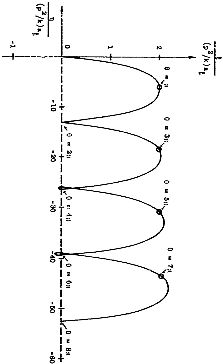
FIG. 3. ACCELERATION CONSTANT IN ROTATING REFERENCE FRAME a_\xi \neq 0 ; a_\eta = 0 ; \omega = 0.01
