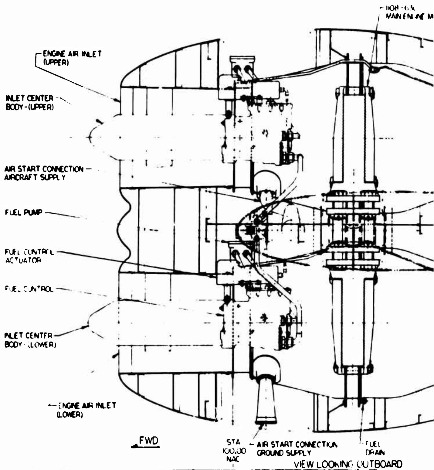
Figure 19. Engine Installation
