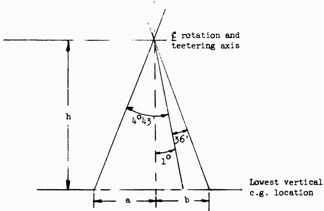
Figure 5. Center-of-Gravity Range.
