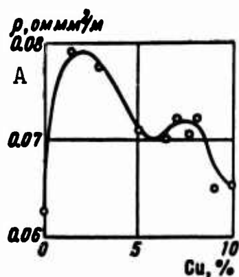
Fig. 1. Resistivity of Mo-Cu alloys as a function of copper content. A) \rho , \text{ohms}\cdot\text{mm}^2/\text{m} .
