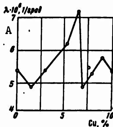
Fig. 2. Linear expansion coefficient of Mo-Cu alloys as a function of copper content. A) \lambda \cdot 10^6 , \text{deg}^{-1} .
