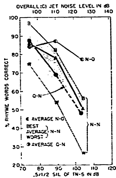
FIG. 2. Speech intelligibility (percent/rhyme words correct) vs jet-noise level for SPP equipments. When both the talker and the listeners are in the noise levels listed on the abscissa (N-N), B refers to developmental equipment, W to operational equipment, and A to an average of about 8 equipments (mostly developmental). For the N-Q and Q-N conditions, only the average results are shown. N-Q means talker in noise, listeners in quiet (noise level of leftmost data point). Q-N is the reverse: talker in "quiet," listeners in noise. The noise levels are as in Fig. 1: over-all (C) level of jet noise (top); and 0.5, 1, 2 SIL of a -6-dB oct noise that is equivalent to the jet noise in its speech-interfering properties.
