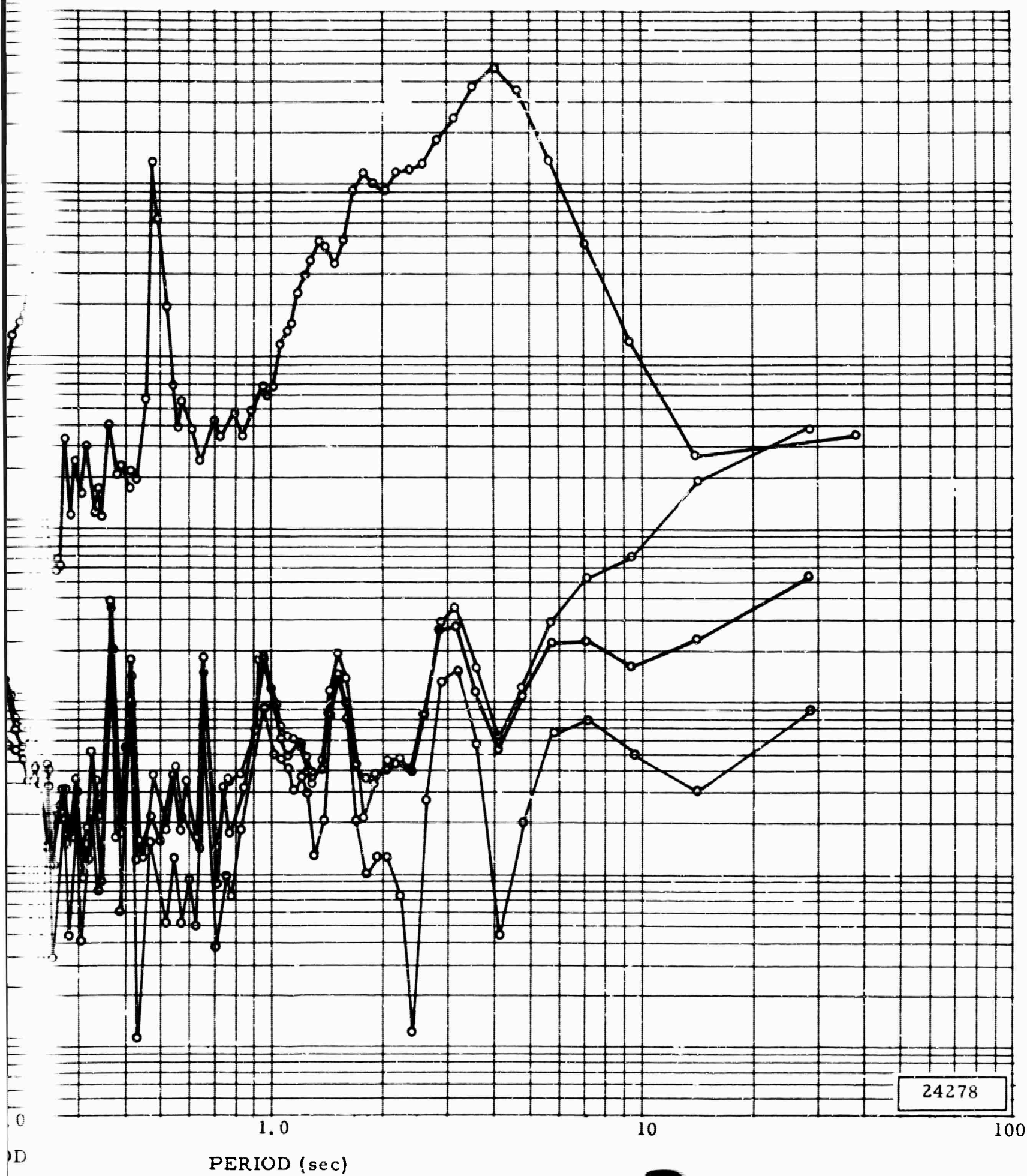
cr density spectra of microseismic and system noise pg 6 short-period seismograph at WMSO
