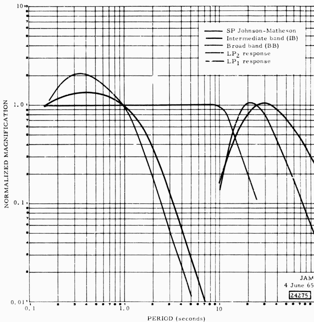
Figure 1. Present normalized frequency responses of seismographs at WMSO
