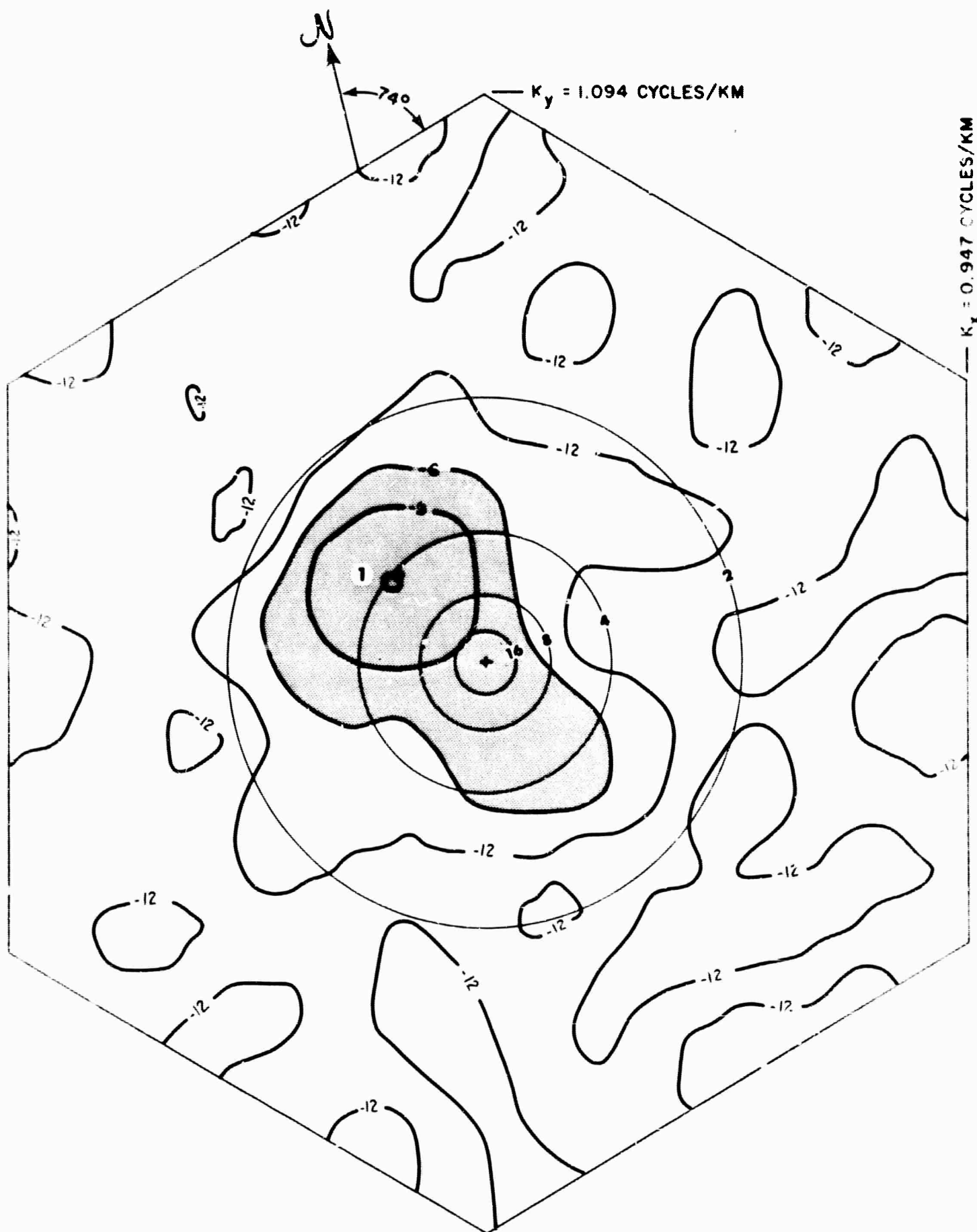
Figure III-5. CPSO Ambient Noise Frequency-Wavenumber Spectrum, May 1965. f = 1.00 \text{ CPS}
