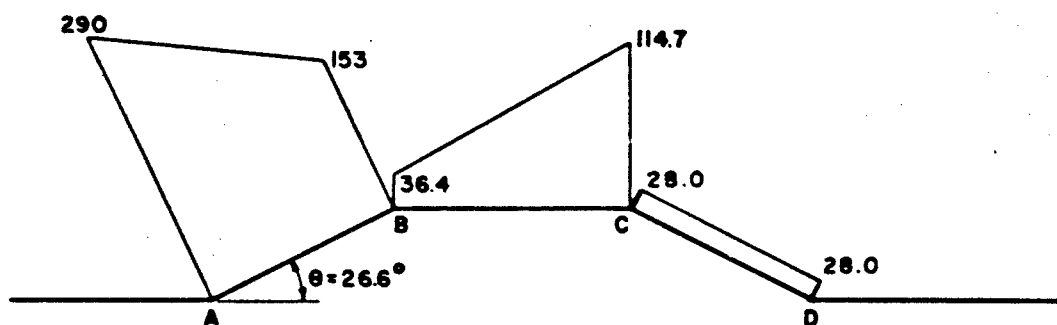
PRESSURES, PSI ABSOLUTE, FOR 100PSIG SHOCK WAVE
