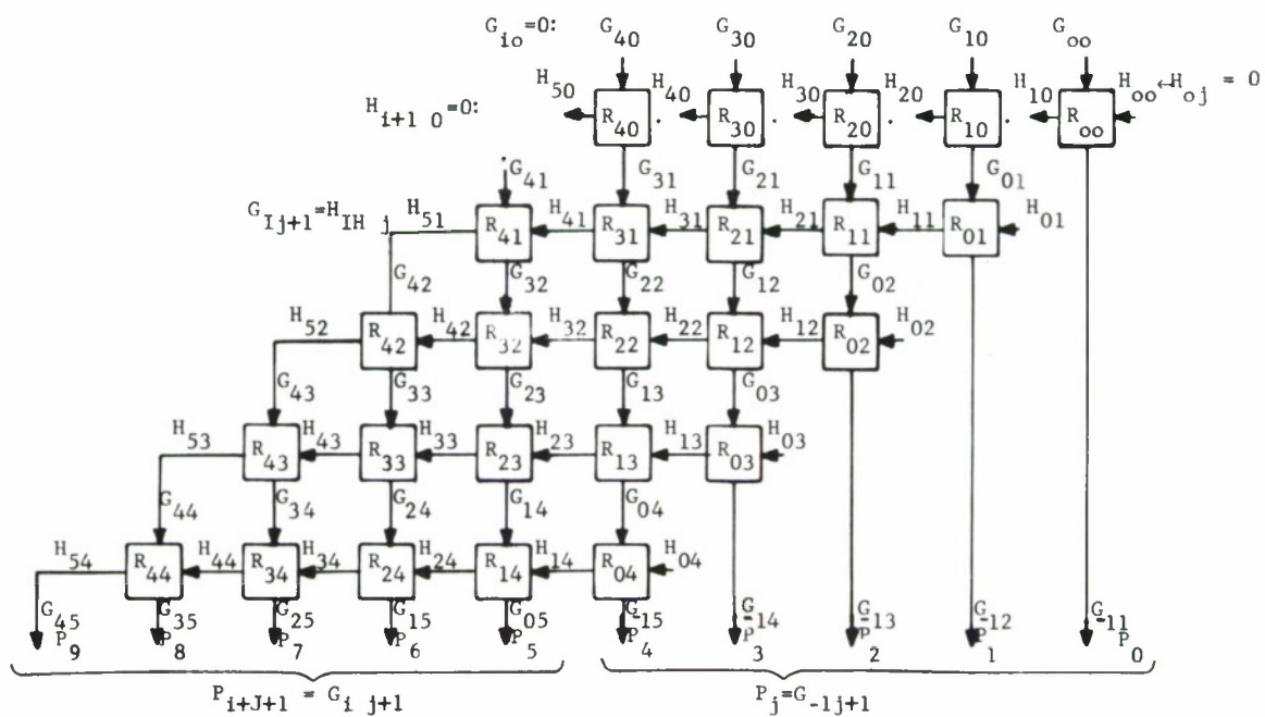
Figure 12 Circuit Construction
