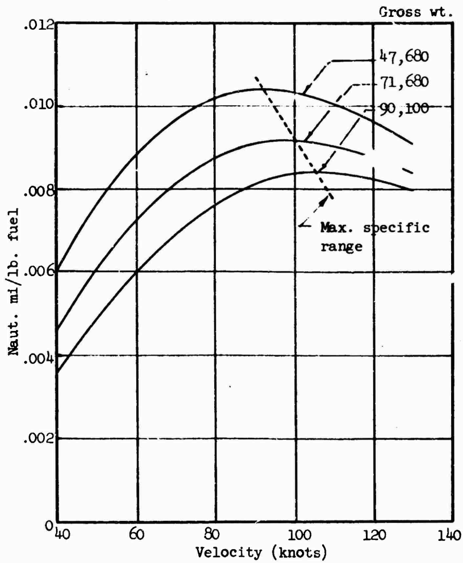
Figure 22. Specific Range Versus Forward Velocity at Sea Level, Standard Day.
