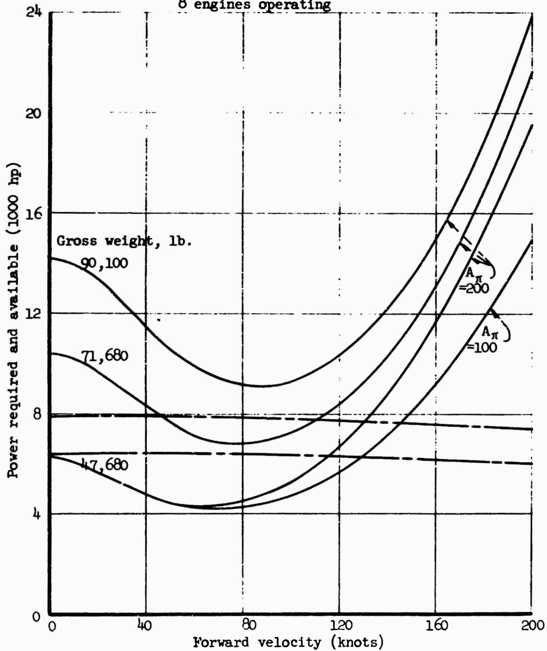
Figure 10a. Power Required and Available Versus Forward Velocity - 20,000 Ft. Altitude.
