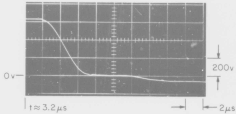
b) Discharge Waveform
