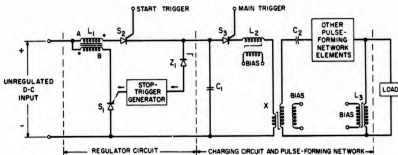
Fig. 1.3 Basic Circuit of the Semiconductor-Magnetic Pulse Generator
