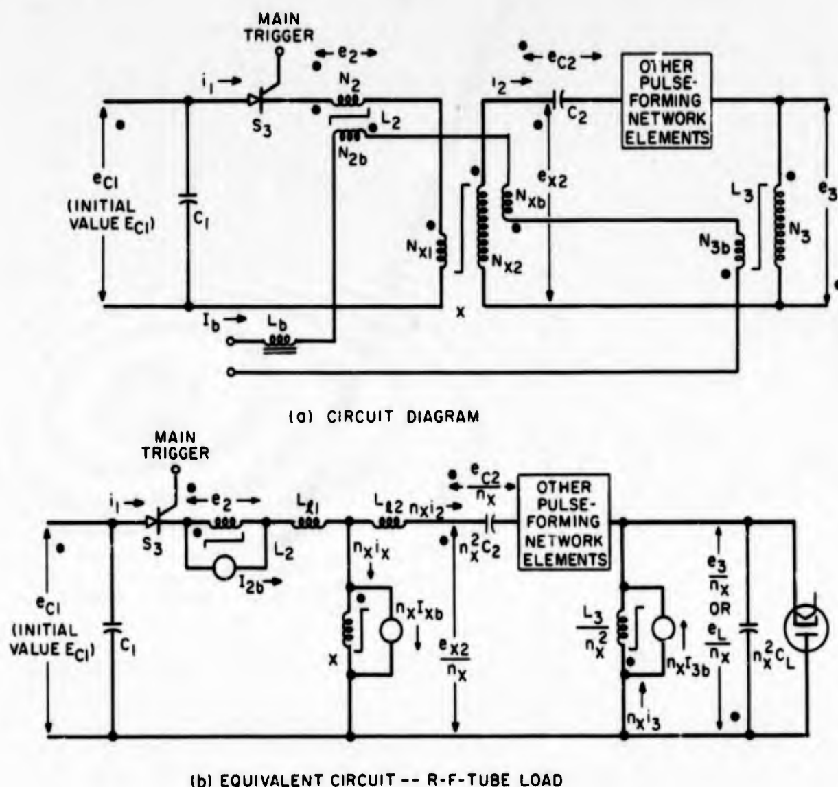
Fig. 3.4 Charging Circuit
