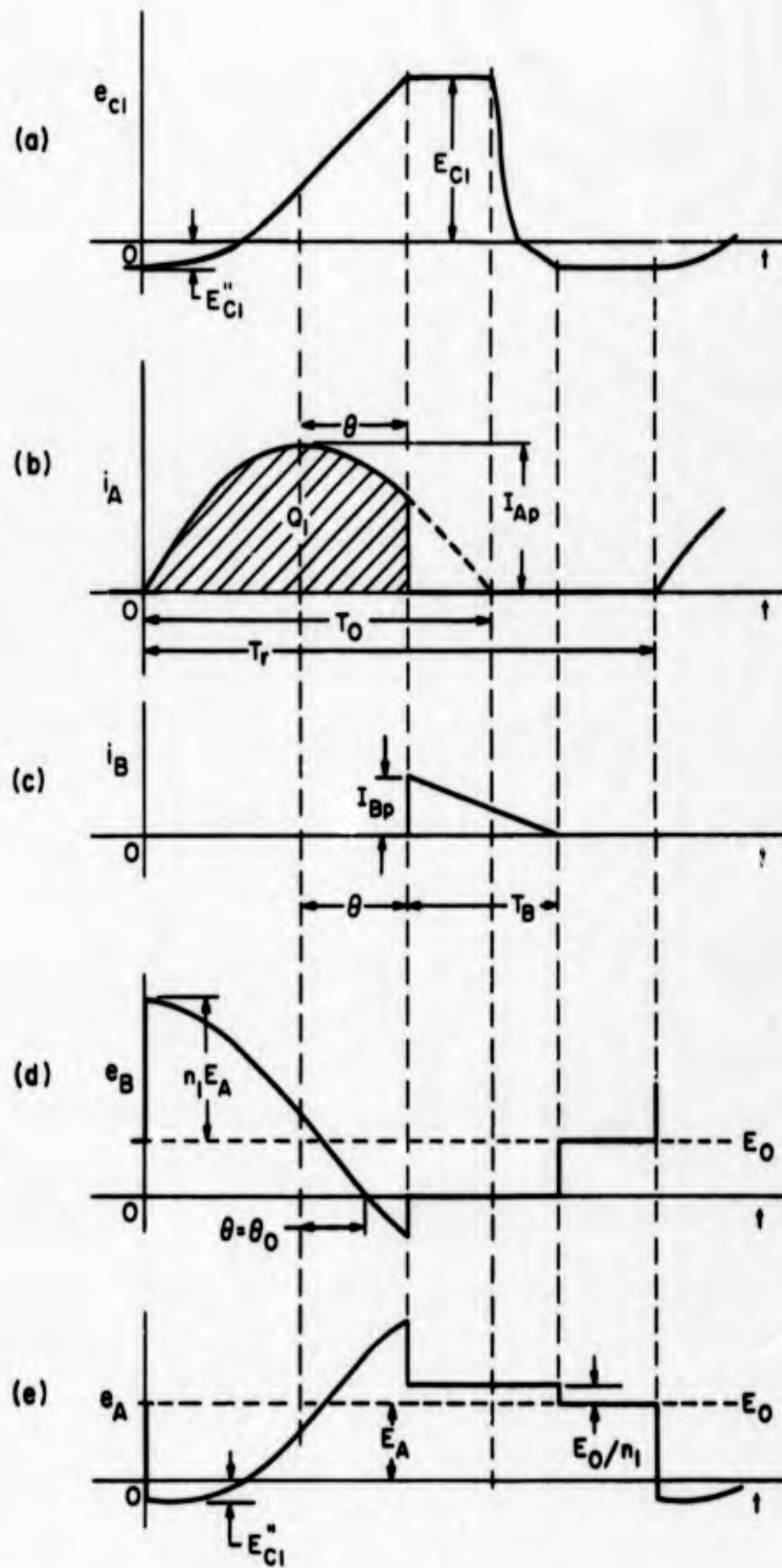
Fig. 3.7 Voltage-Regulator Waveforms
