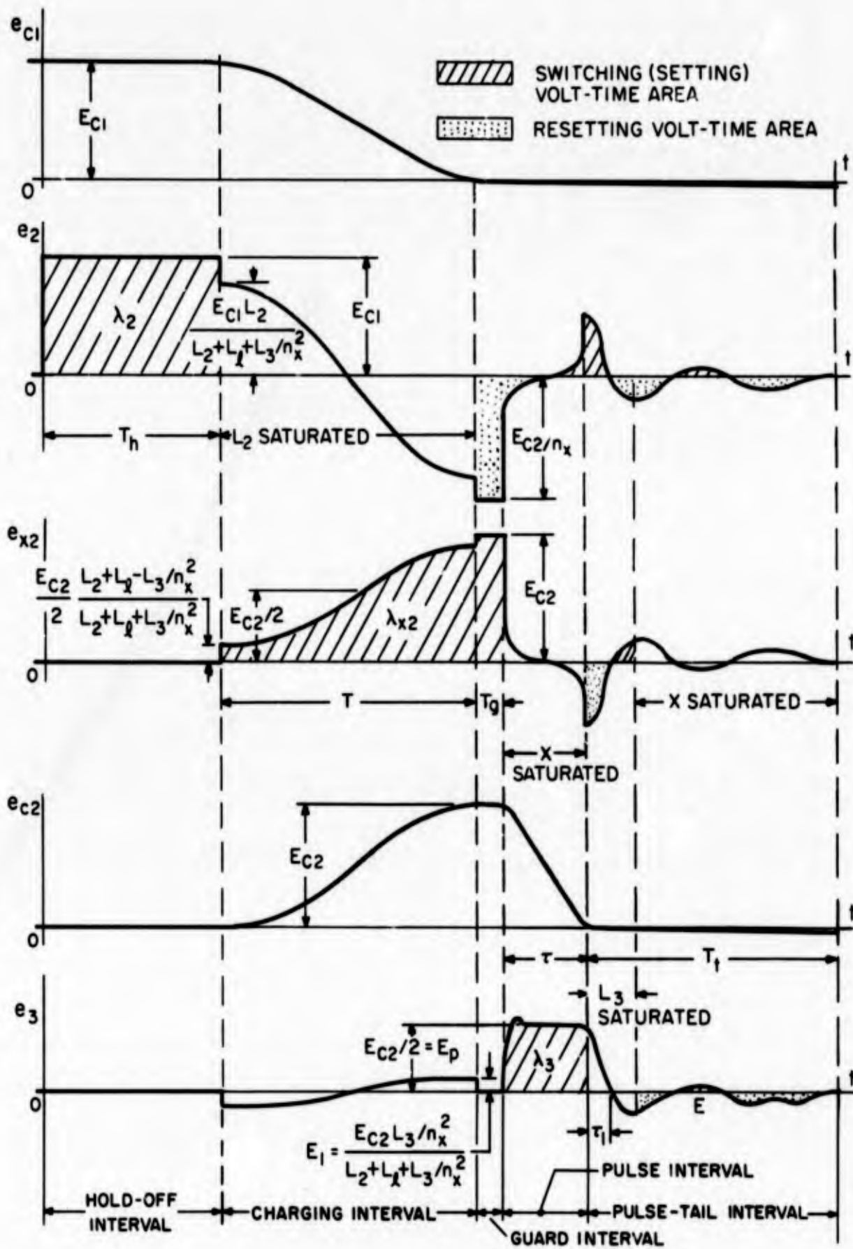
Fig. 3.5 Charging-Circuit Waveforms--R-F-Tube
