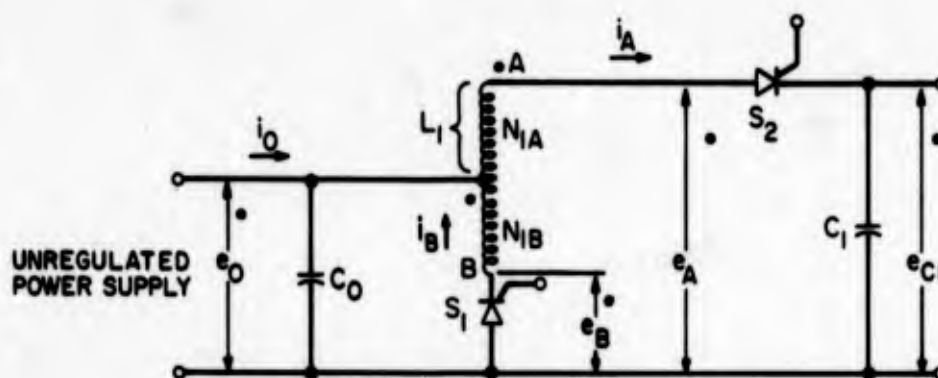
Fig. 3.6 Basic Voltage-Regulator Circuit
