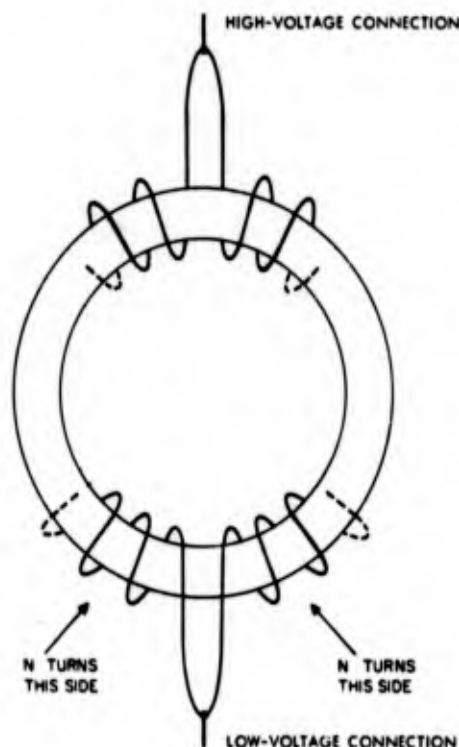
Fig. 4.2 Winding Configuration of N-Turn Toroidal Inductor
