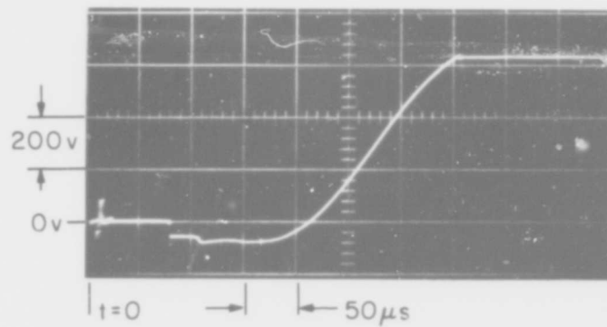
Fig. 5.6 Voltage e_s across S_{3C}
