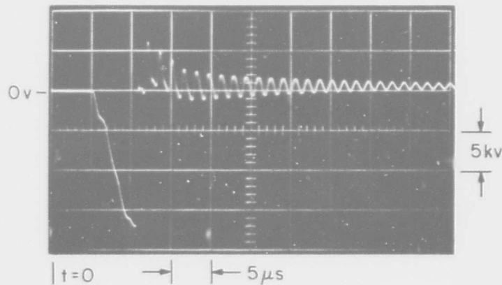
Fig. 5.4 Voltage e_X (Across Transformer High-Voltage Winding)
