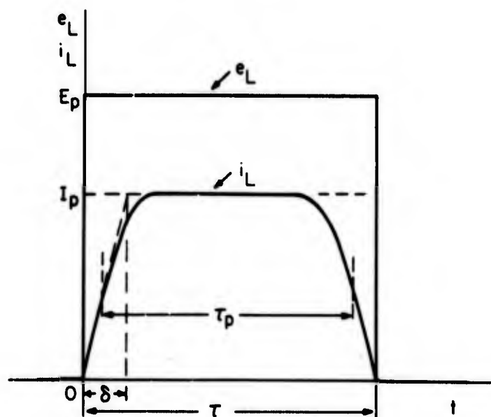
Fig. 3.2 Nominal Pulse Shapes
