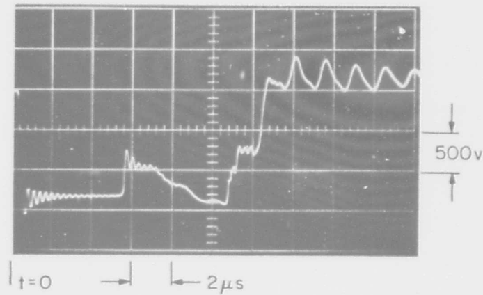
Fig. 5.10 Bias inductor L_b Voltage e_b
