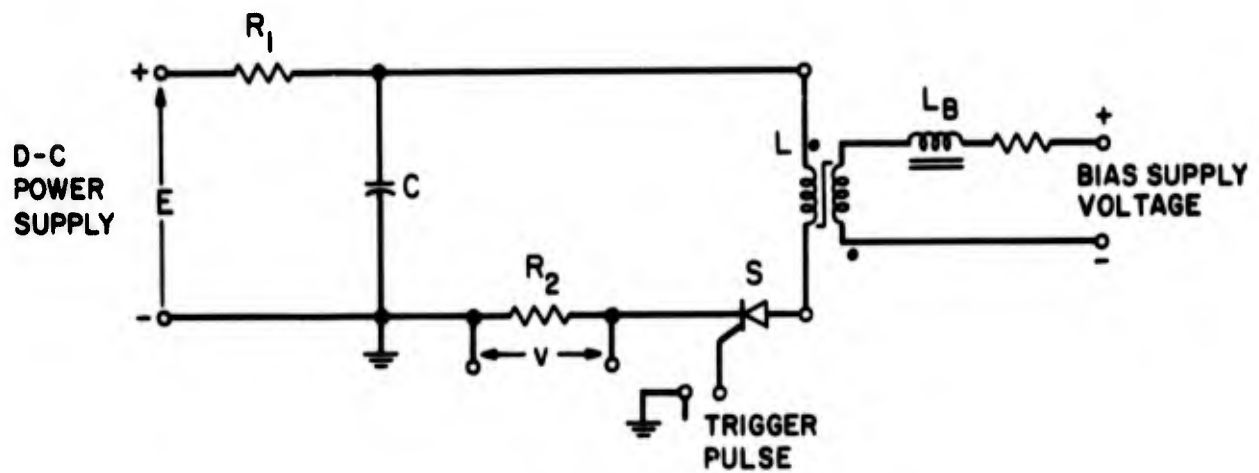
Fig. B.1 Saturable-Inductor Test Circuit
