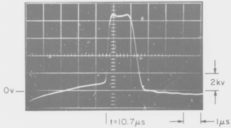
b) Output Pulse Shape
