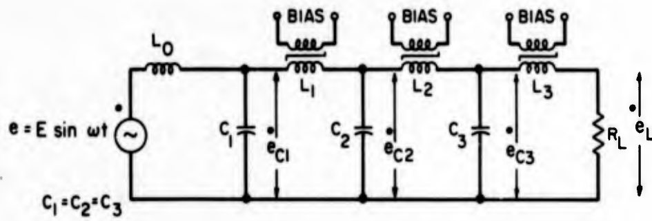
Fig. 1.1 All-Magnetic Pulse Generator
