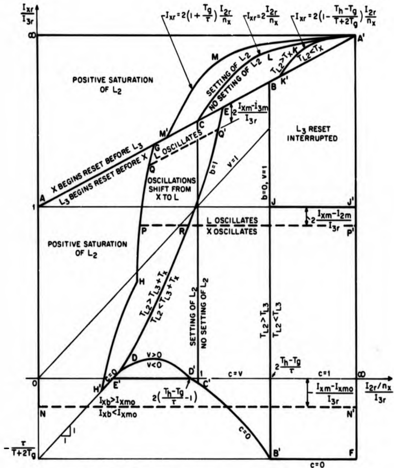
Fig. A.2 Mode Diagram for R-F Tube Load and Zero Residual Voltages
