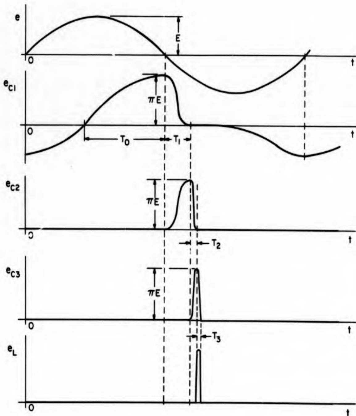
Fig. 1.2 Waveforms for Circuit of Fig. 1.1
