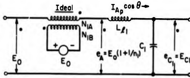
Fig. 3.8 Equivalent Circuit Showing Effect of L_{11}
