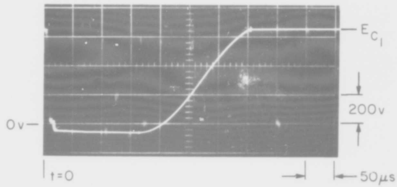
a) Discharge and Charging Waveform
