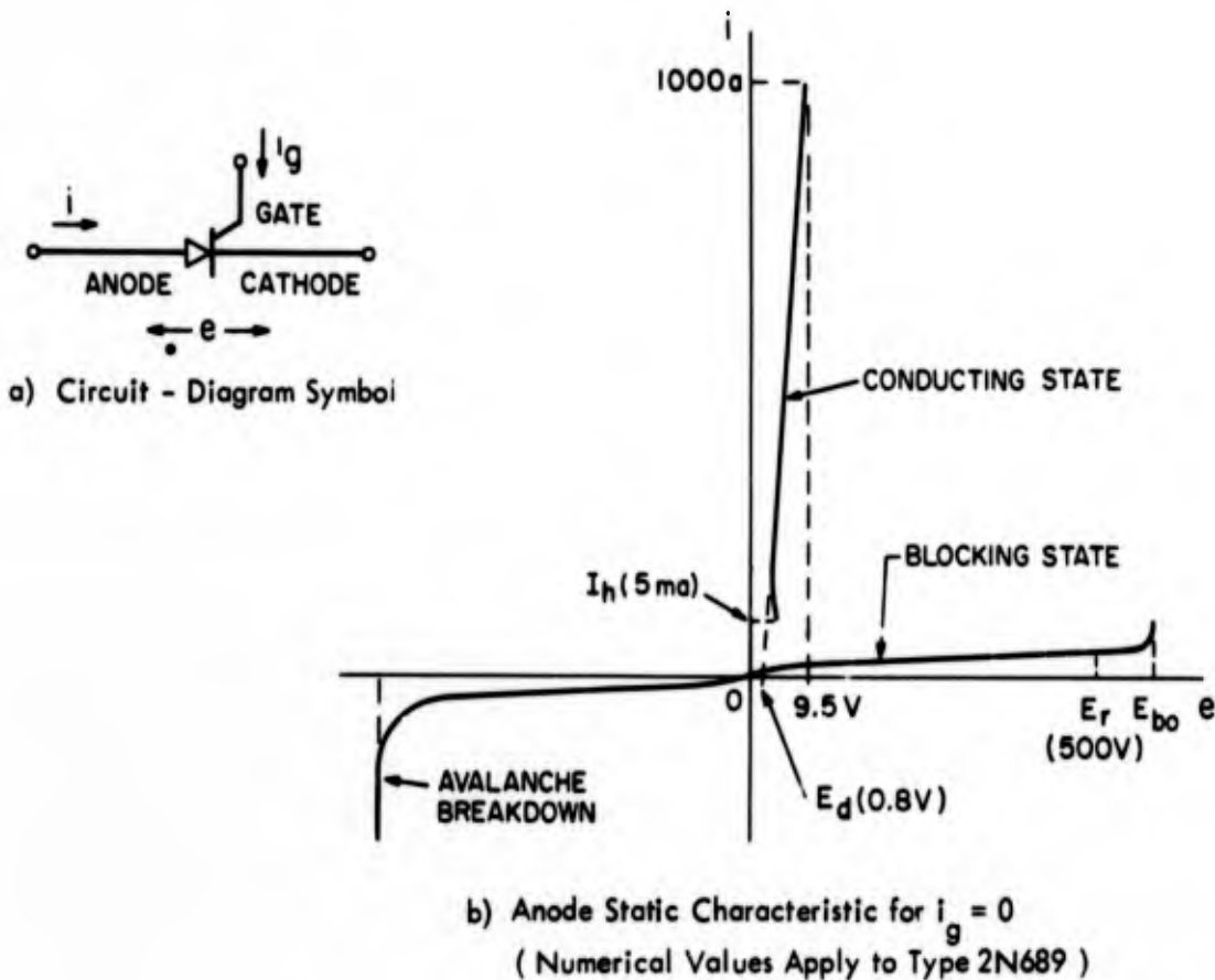
Fig. 2.3 Static Characteristic of Controlled Rectifier
