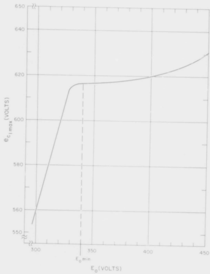
Fig. 5.8 Measured Regulation for E_{C1} = 612.5 V
