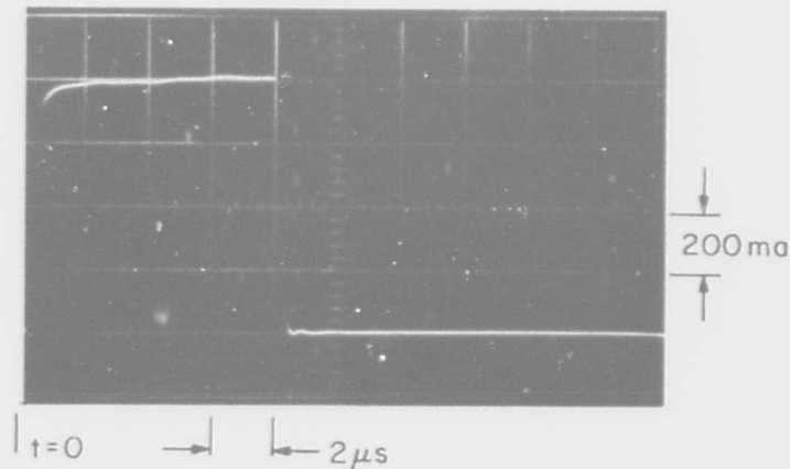
Fig. 5.11 Gate-Current Pulse for S_{3a}
