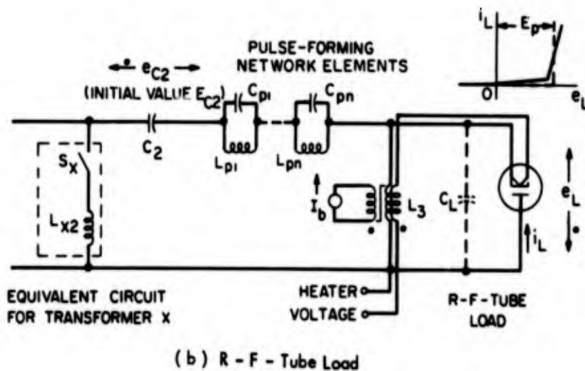
Fig. 3.1 Pulse-Forming Network and Load
