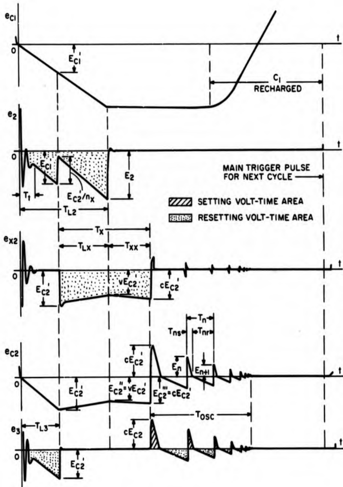
Fig. A.1 Waveforms for a Particular Resetting Mode
