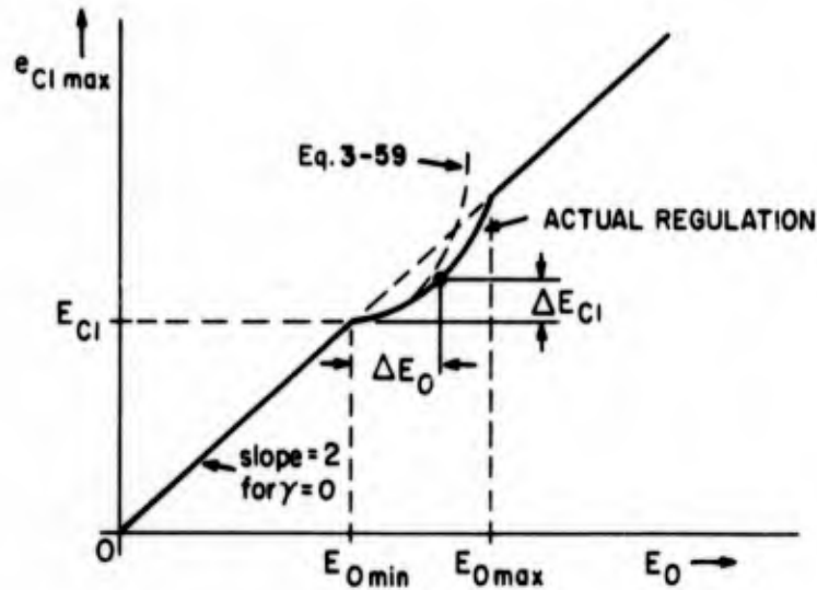
Fig. 3.9 Regulation Characteristic Showing Effect of L_{l1}
