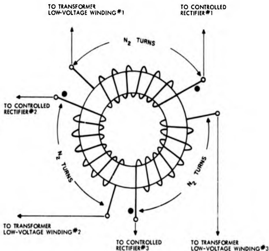
Fig. 4.3 Hold-Off Inductor Winding Configuration for 3 Parallel Discharge Paths
