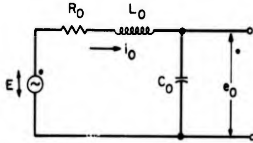
Fig. 3.10 Power-Supply Equivalent Circuit
