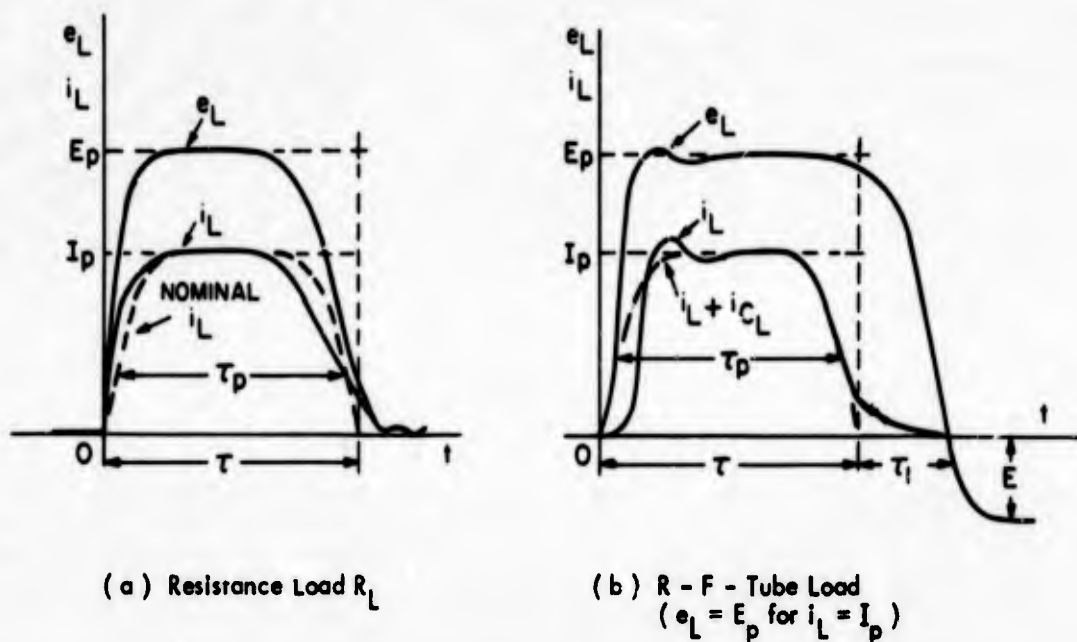
Fig. 3.3 Typical Output-Pulse Shapes
