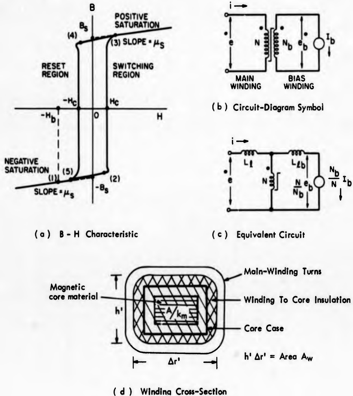
Fig. 2.1 The Saturable Inductor
