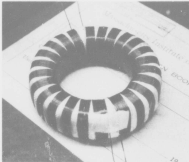
Fig. 5.12 Diode Inductor L_3 High-Voltage Winding Construction
