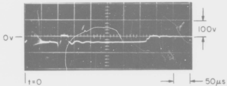
c) Resetting Voltages
