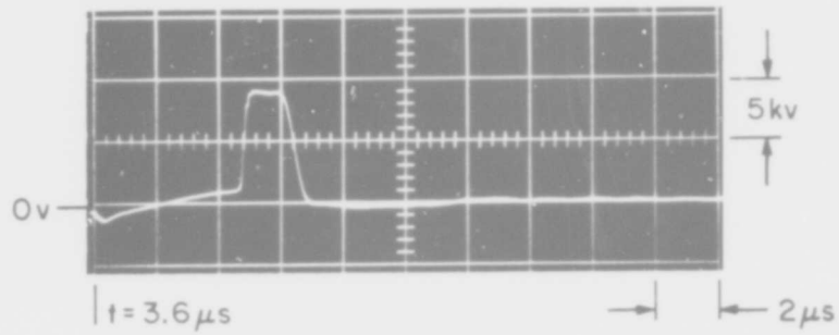
a) Output Pulse, Showing E_L
