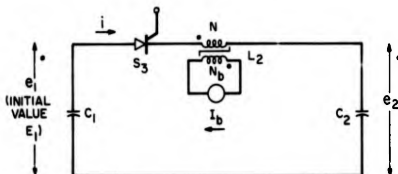
Fig. 2.4 Controlled Rectifier with Hold-Off Inductor
