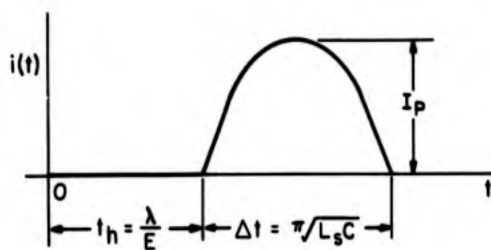
Fig. B.2 Current i(t) in Fig. B.1
