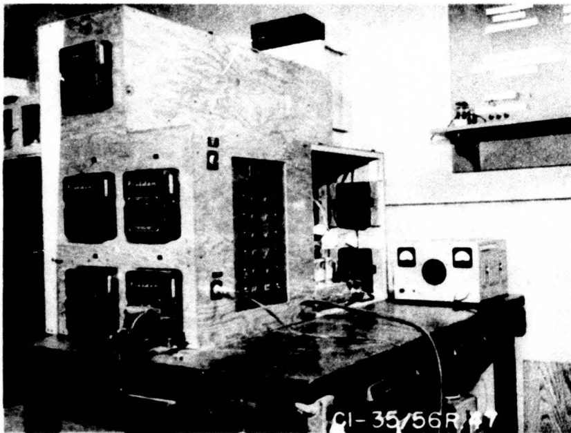
Rear View of Instrument Panel for Recording Strains and Deflections
