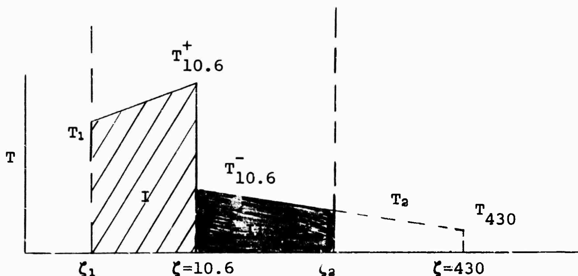
FIG. 3. QUADRATURE DIAGRAM AT \zeta = 10.6
