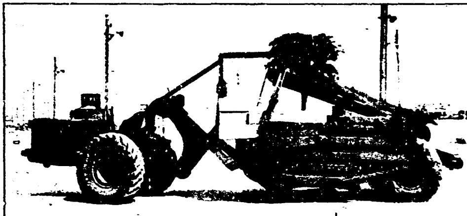
SUPER C TOURNAPULL WITH MODEL LP SGRAFER LOADED WITH 1 TON CONCRETE BLOCKS SPEED OF TRAFFIC FROM 5 TO 10 MILES PER HOUR
