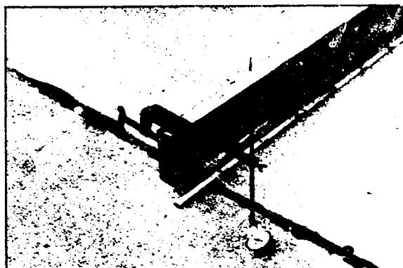
(B) DETAIL OF EXTENSOMETER AND SUPPORT.
