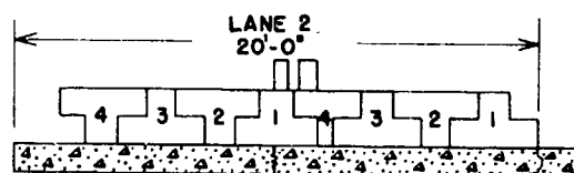
DIAGRAM OF TRAFFIC DISTRIBUTION THE 4 TRIPS INDICATED ON THE DIAGRAM ARE ASSUMED TO MAKE 2 COVERAGES
