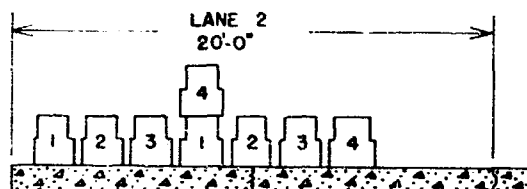
DIAGRAM OF TRAFFIC DISTRIBUTION THE 4 TRIPS INDICATED ON THE DIAGRAM ARE ASSUMED TO MAKE 2 COVERAGES
