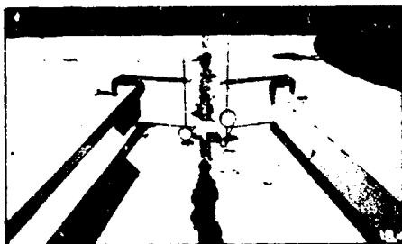
(C) ARRANGEMENT FOR DEFLECTION MEASUREMENT AT A JOINT.
