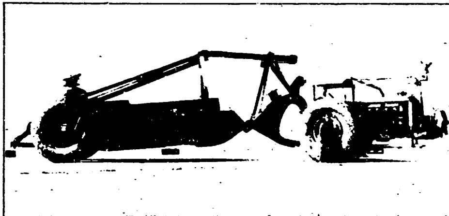
A-3 TOURNAPULL WITH MODEL NU SCRAPER LOADED WITH 1 TON CONCRETE BLOCKS SPEED OF TRAFFIC FROM 4 TO 5 MILES PER HOUR
