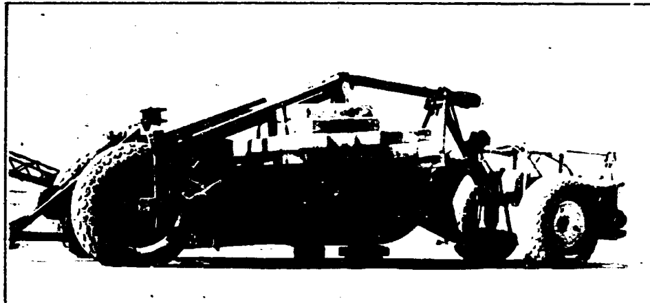
A-3 TOURNAPULL WITH MODEL NU SCRAPER LOADED WITH 1 TON CONCRETE BLOCKS SPEED OF TRAFFIC FROM 3.0 TO 3.5 MILES PER HOUR
