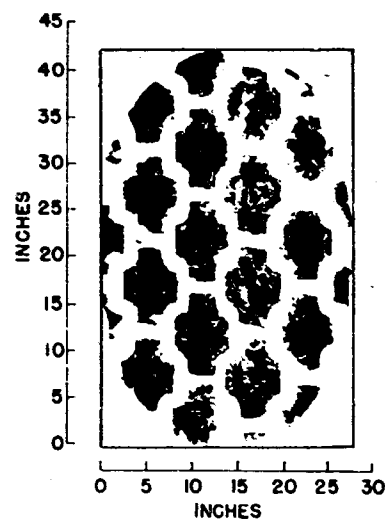
TYPICAL TIRE PRINT INFLATION PRESSURE 52 LBS. PER SQUARE INCH AREA 1051 SQUARE INCHES
