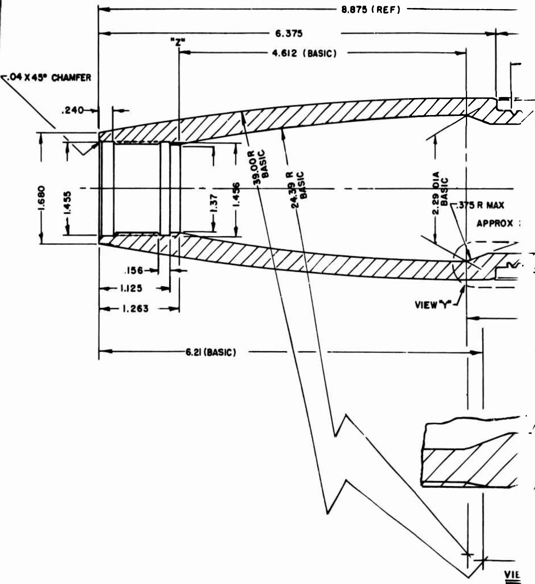
Fig 1 Head detail from dwg No. 660853 Mk 1, mod 1, 2.75 inch rocket
