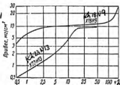
Fig. 31. Kinetics of oxidation of chromium-nickel steels Kh18N9 and Kh23N13 in air at 1100^{\circ} [66]:
