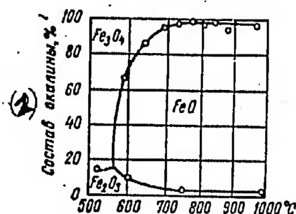
Fig. 4. Change in composition of scale on iron versus heating temperature in a medium of air [38]: (1) scale composition, %.
