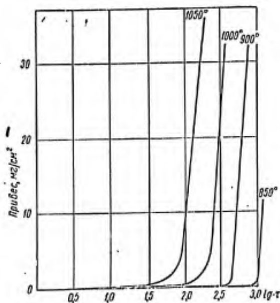
Fig. 26. Induction period versus temperature in oxidation of 1Kh13 steel in air [40]: 1 - weight gain, mg/cm 2 .
