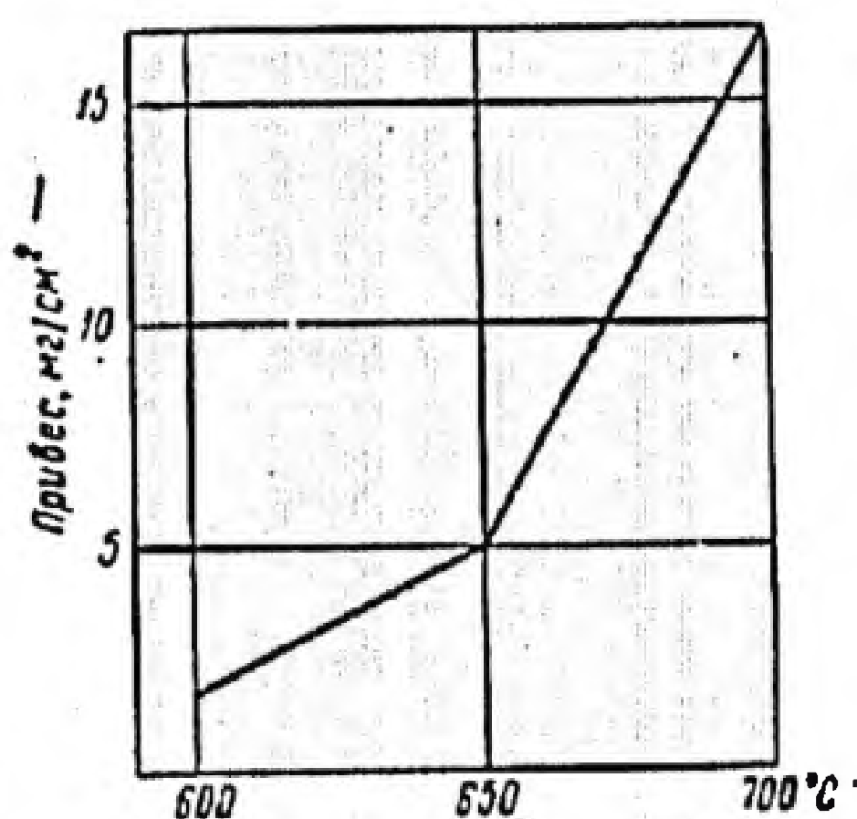
Fig. 46. Oxidation of steel 15Kh1M1F in air versus temperature in the 600-700°C range [27]: 1 - weight gain, mg/cm 2 .
