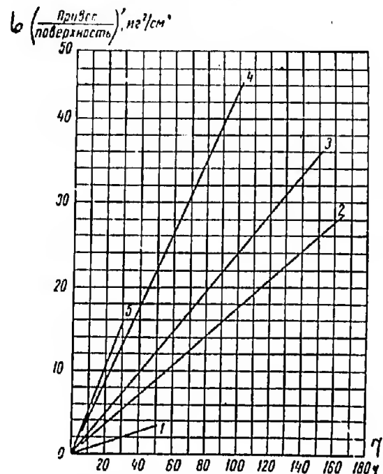
Fig. 22. Kinetics of oxidation of chromium steel containing 31.3% Cr in water vapor [39]:
