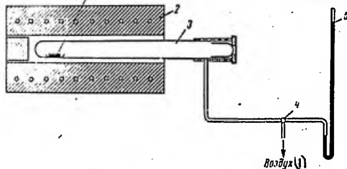
Fig. 8. Diagram of device for determination of oxygen by manometric method. [43]. (1) Air.
