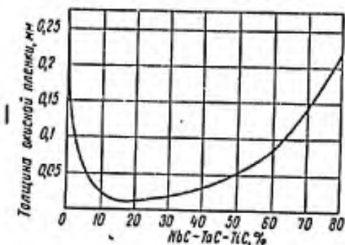
Fig. 62. Influence of a solid solution of carbides NbC-TaC-TiC on the scale resistance of metal-ceramic TiC-Co alloys at 980°; test period 64 hours [13]:
