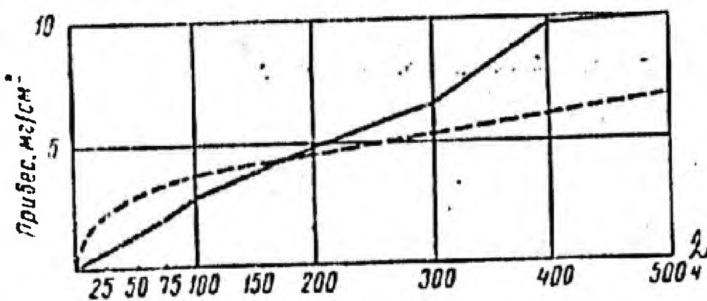
Fig. 45. Kinetics of oxidation of steel 15Kh1M1F in air and in superheated steam at 600° [27]: - - - in superheated steam; - - - in air; 1 - weight gain, mg/cm²;
