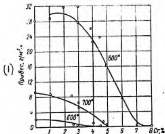
Fig. 9. Influence of chromium on scale formation on steel (0.15% C, 0.7 to 0.9% Si) in air at temperatures up to 800° [22]: (1) Weight gain, \text{g/m}^2 \cdot \text{h} .
