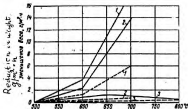
Fig. 1. Scale resistance of chromium-silicon steel in water vapor and in air. Test period 120 hours [227]. water vapor; air: 1 - 0.5% Mo, 1.0% Cr, 0.4% Si; 2 - 0.5% Mo, 2.5% Cr, 1.5% Si; 3 - 0.5% Mo, 6.0% Cr, 2.3% Si.
