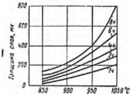
Fig. 69. Thickness of diffusion layer of chromium versus chromizing temperature [19]: l - Layer thickness, \mu
