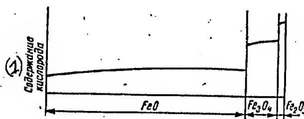
Fig. 3. Structure of scale on iron [22]: (1) oxygen content.
