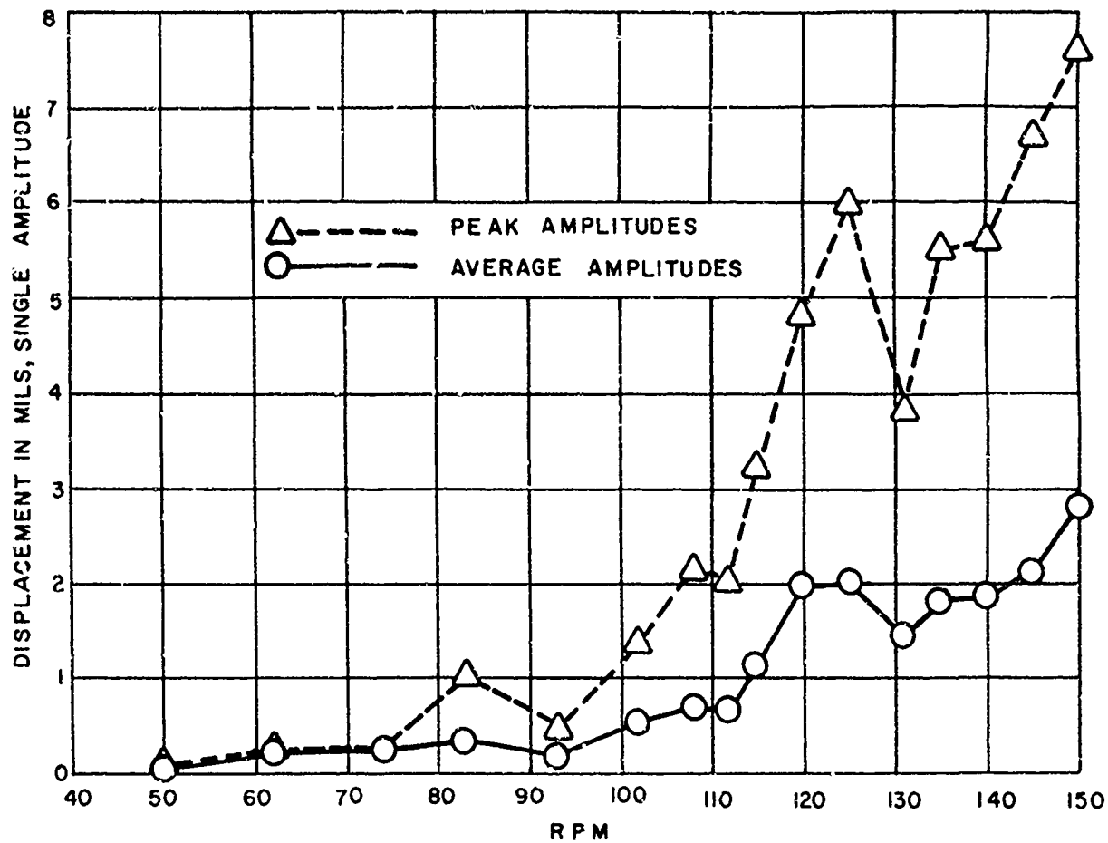
Figure 9 - Longitudinal Blade Frequency Displacement of Thrust Bearing Housing versus RPM
