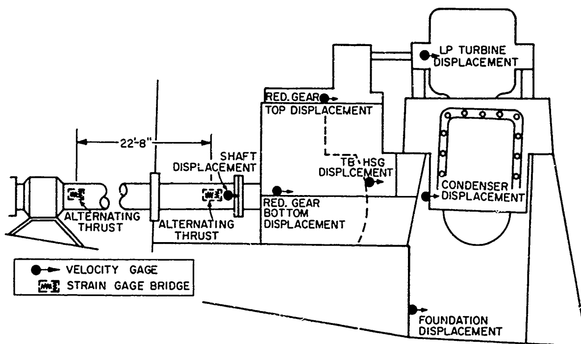
Figure 2 - Main Propulsion Plant of SIMON LAKE Showing Location and Orientation of Gages
