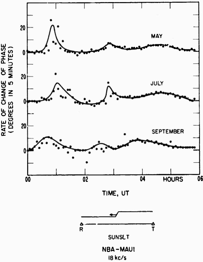
FIGURE 3. Rate of change of phase observed at Maui on the 18-kc/s signals from NBA at sunset.
