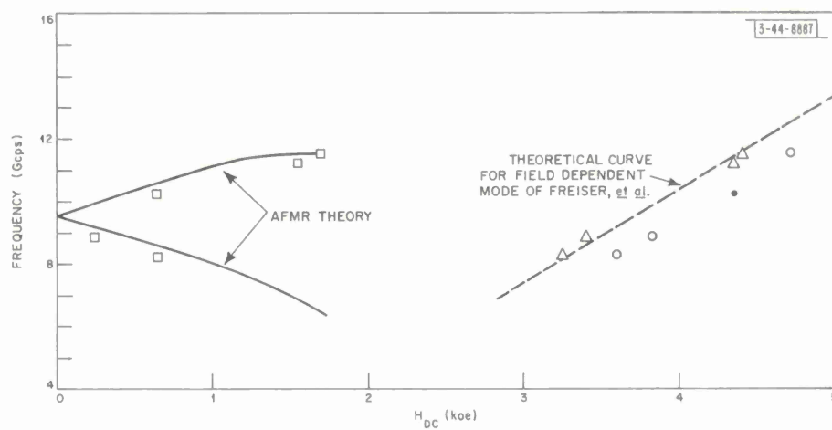
Fig. 16. Observed resonances for H_{DC} parallel to [100] axis.
