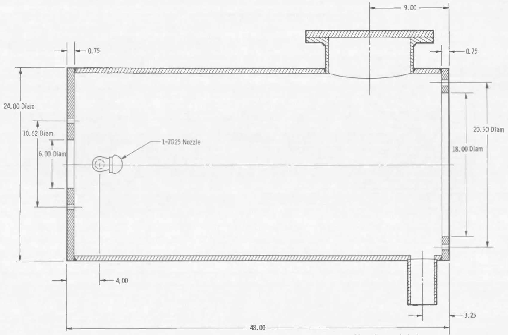
Fig. 3 Condenser Assembly
