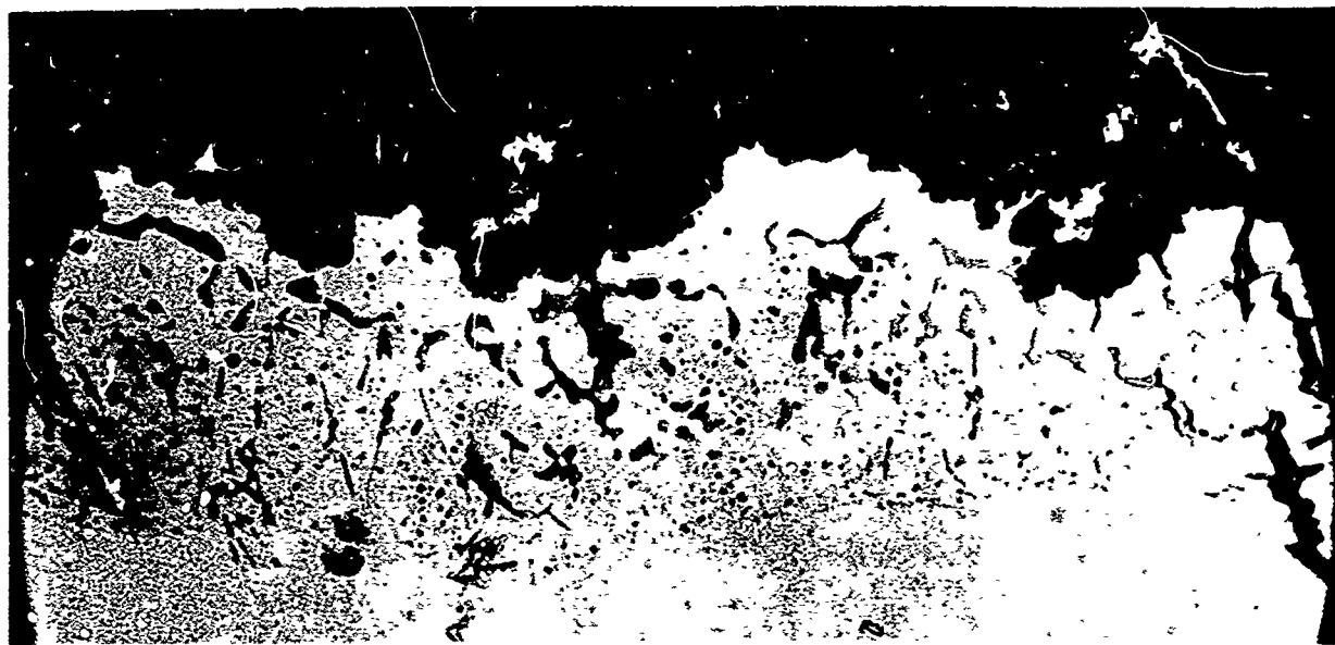
Fig. 37 Commercial alloy 713 coated with sodium sulfate and exposed to dry oxygen at 300°C for 33 hours (713-2). 500X
