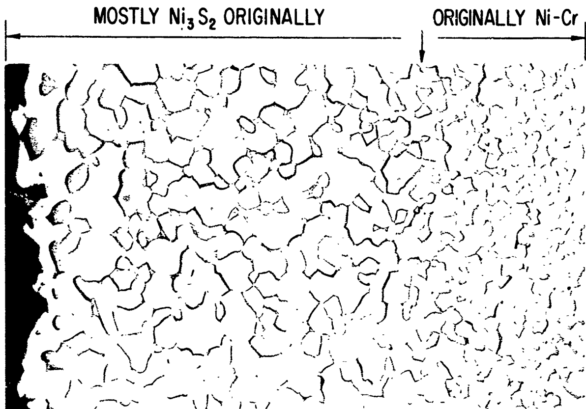
Fig. 15 Ni + 20% Cr alloy heated 2 hours at 850°C in contact with Ni 3 S 2 + H 2 . 250X
