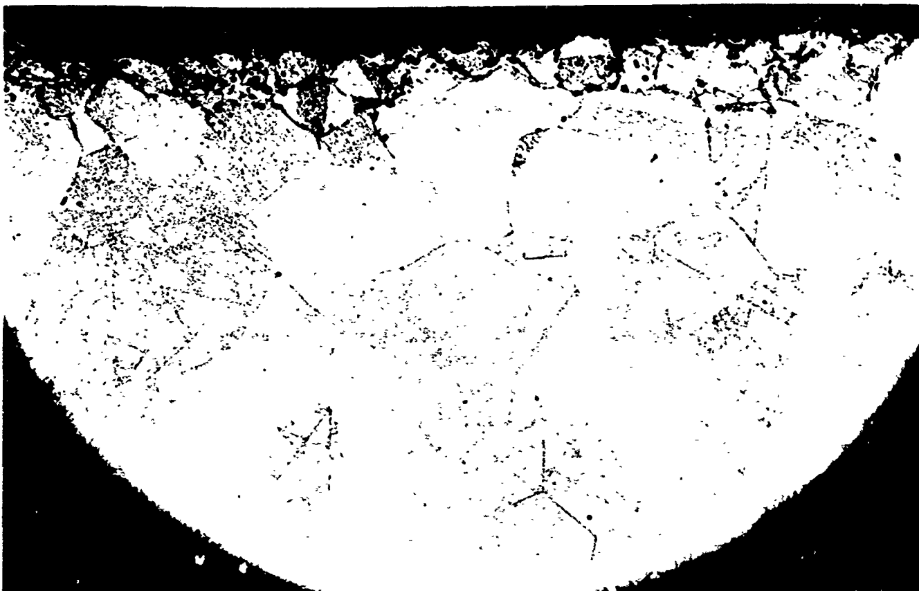
Fig. 28 Nickel-10% chromium alloy coated with sodium sulfate pretreated in wet argon and exposed to wet oxygen at 900°C for 4 hours (NC1-3). 500X
