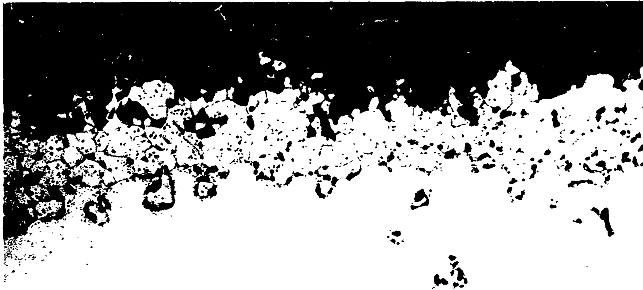
Fig. 38 Commercial alloy SEL coated with sodium sulfate and exposed to dry oxygen at 900°C for 70 hours (SEL-1). 500X
