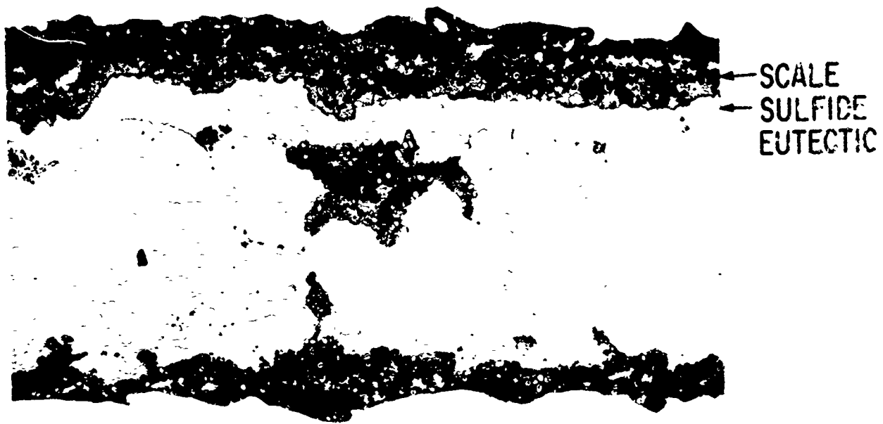
Fig. 1 "A" nickel heated 48 hours at 950°C in Na 2 SO 4 , evacuated capsule. 100X
