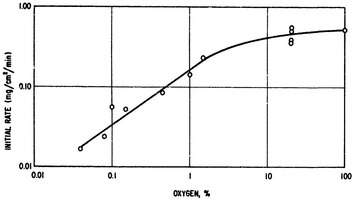
Fig. 7 The dependence of initial corrosion rate on oxygen partial pressure.
