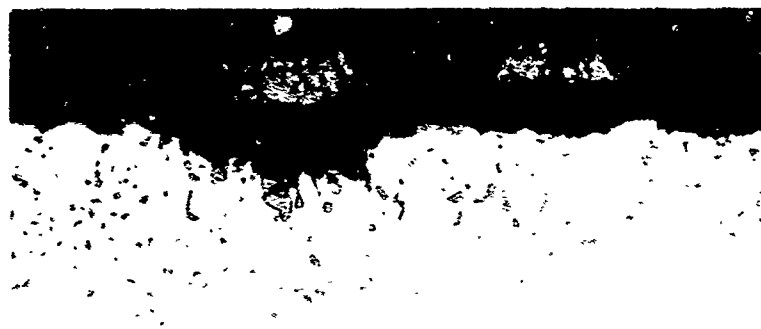
Fig. 18 99.99% Nickel, heated 2 hours at 850°C in SO 2 gas; complete conversion to sulfide eutectic. 150X
