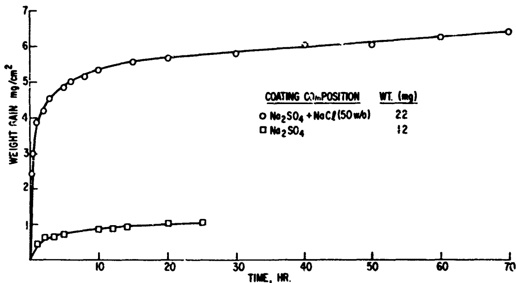
Fig. 39 Weight gain of coated 509 in dry oxygen at 900°C.
