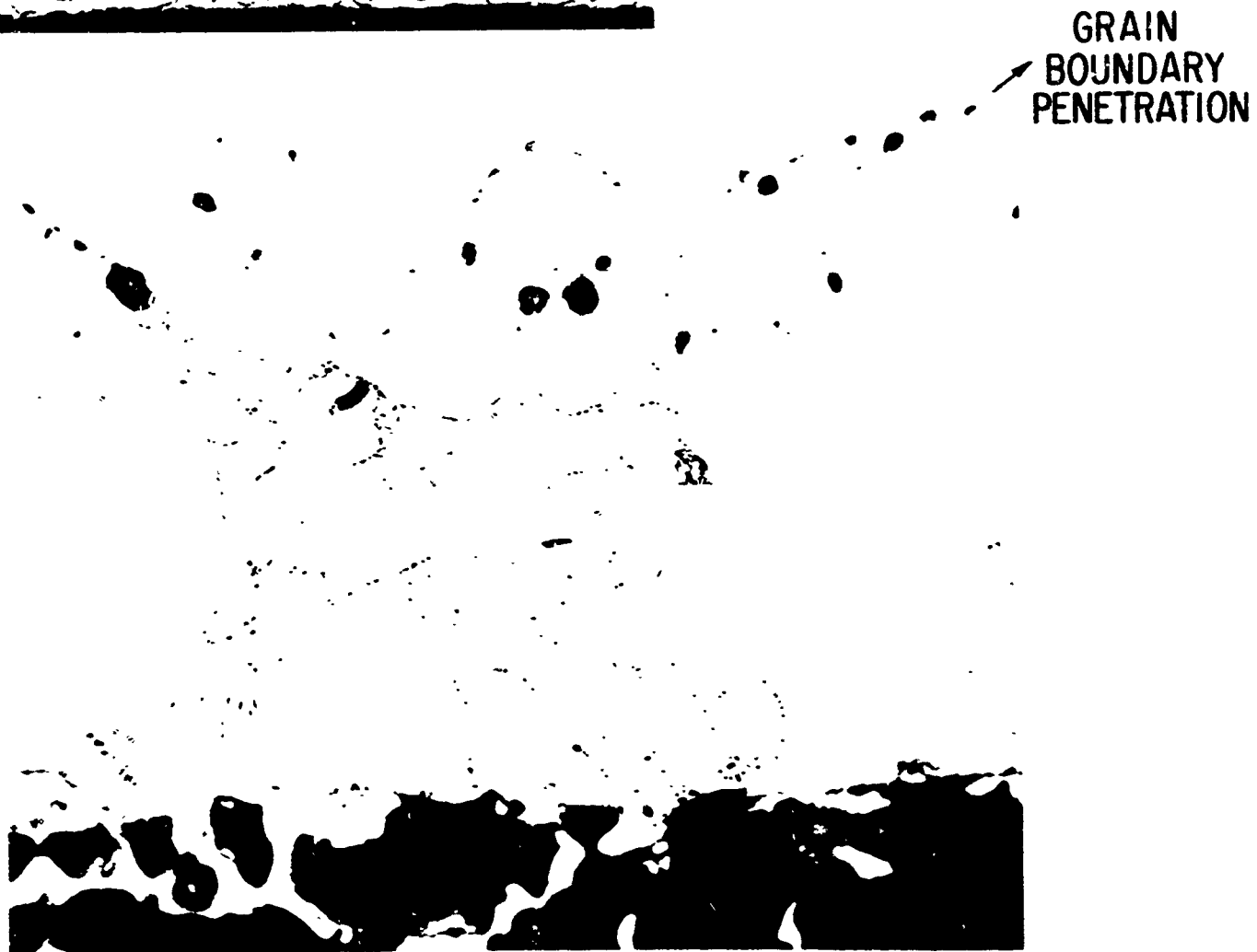
Fig. 7 "A" nickel heated 4 hours at 950^\circ\text{C} in \text{Na}_2\text{SO}_4 , \text{H}_2 bubbled through melt. 500X
