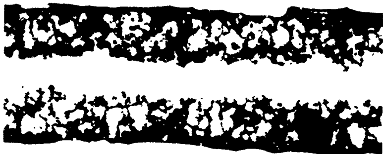
Fig. 10 "A" nickel heated 1 hour at 900^\circ\text{C} in \text{Na}_2\text{SO}_4 , in air. 100X
