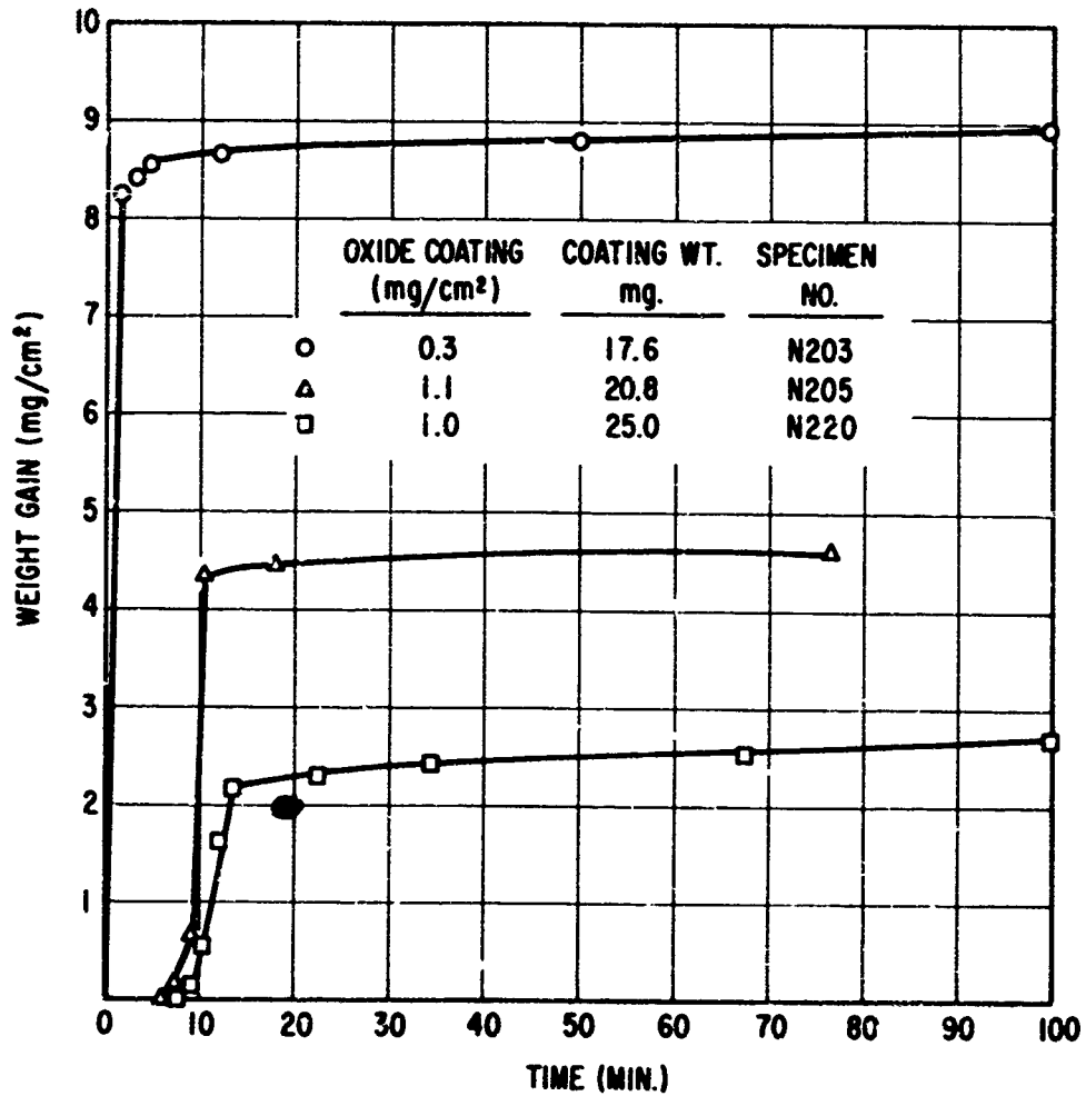
Fig. 8 The effects of preoxidizing nickel on corrosion in dry oxygen at 850^\circ\text{C} .
