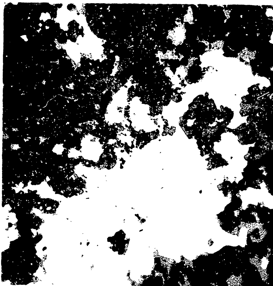
Fig. 5 Co-30 w/o Cr heated 48 hours at 950°C in Na 2 SO 4 , in air. 750X
