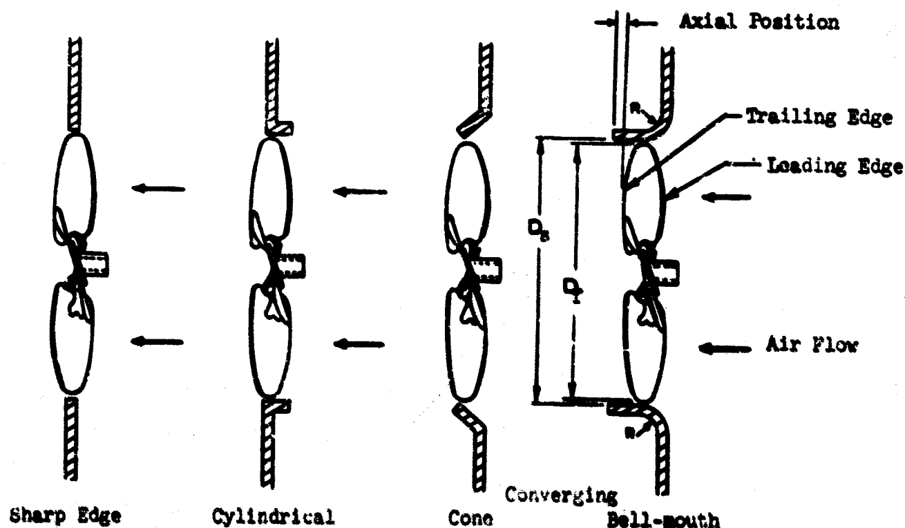
Figure 19 Orifice Types
