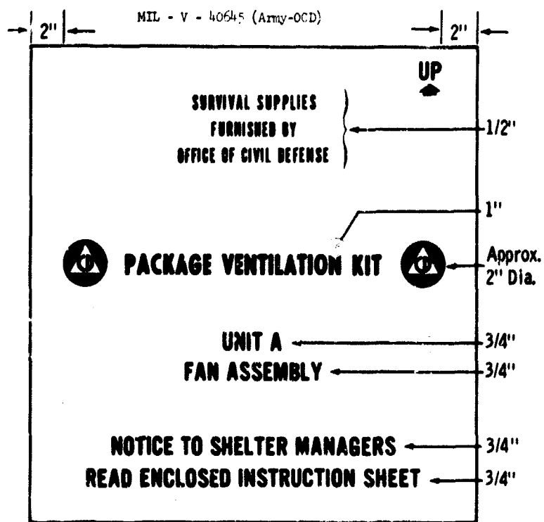
FRONT PANEL
