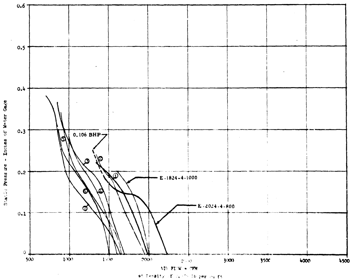
Figure 17 Fan Characteristics for One-man PVK
