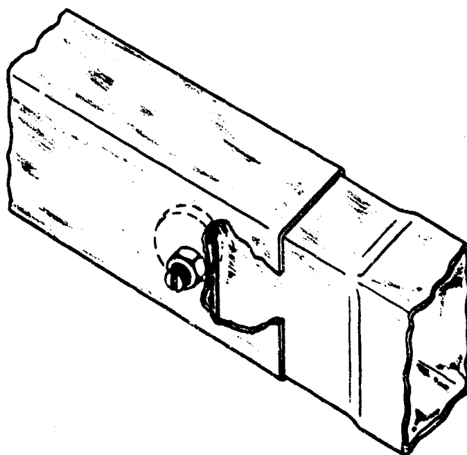
Eccentric-Cam
