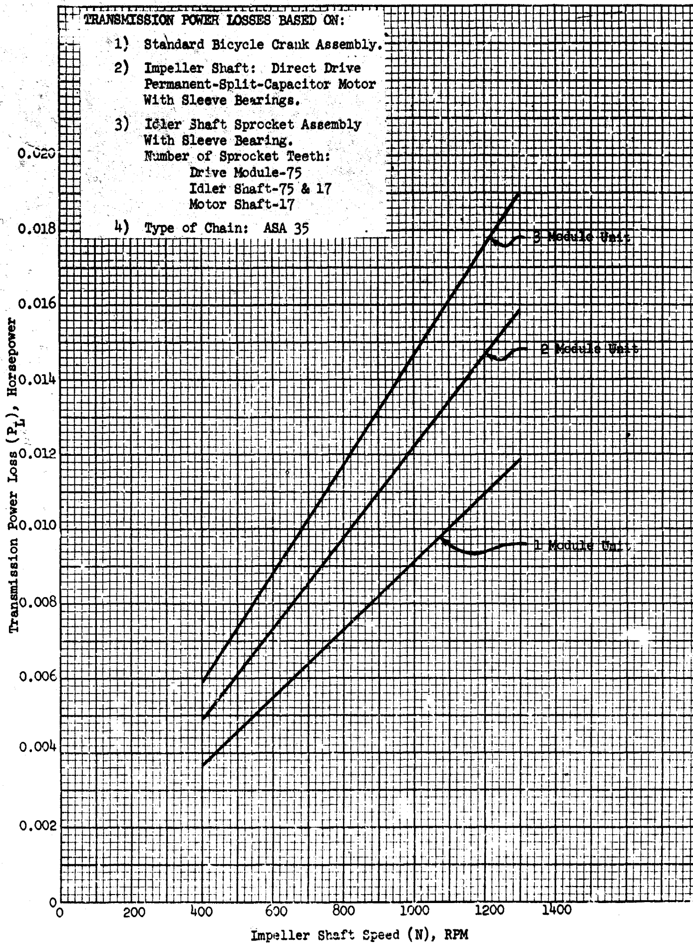
Figure 34 FVK Transmission Power Losses
