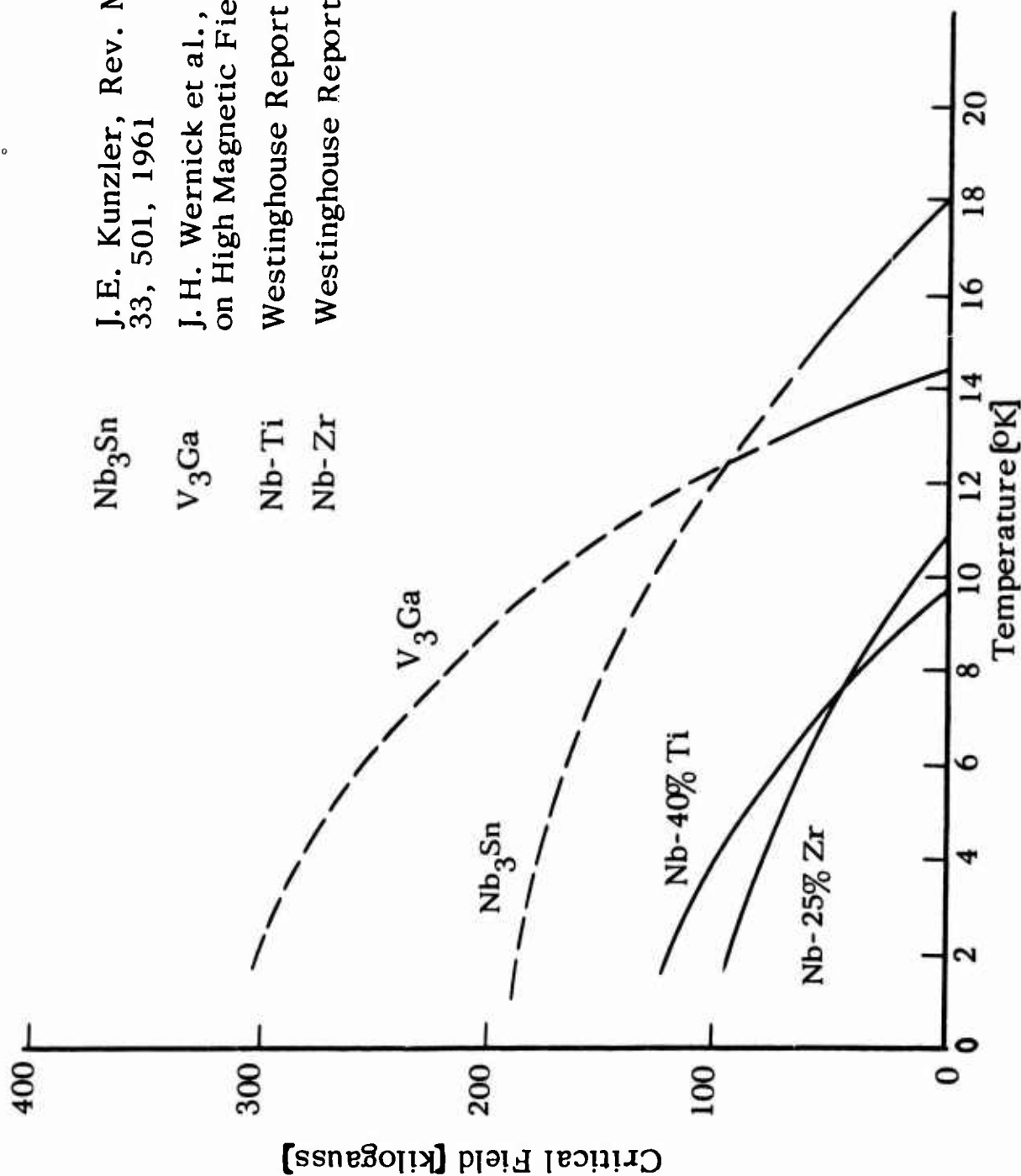
Figure 2. Critical Fields for Various Superconductors
