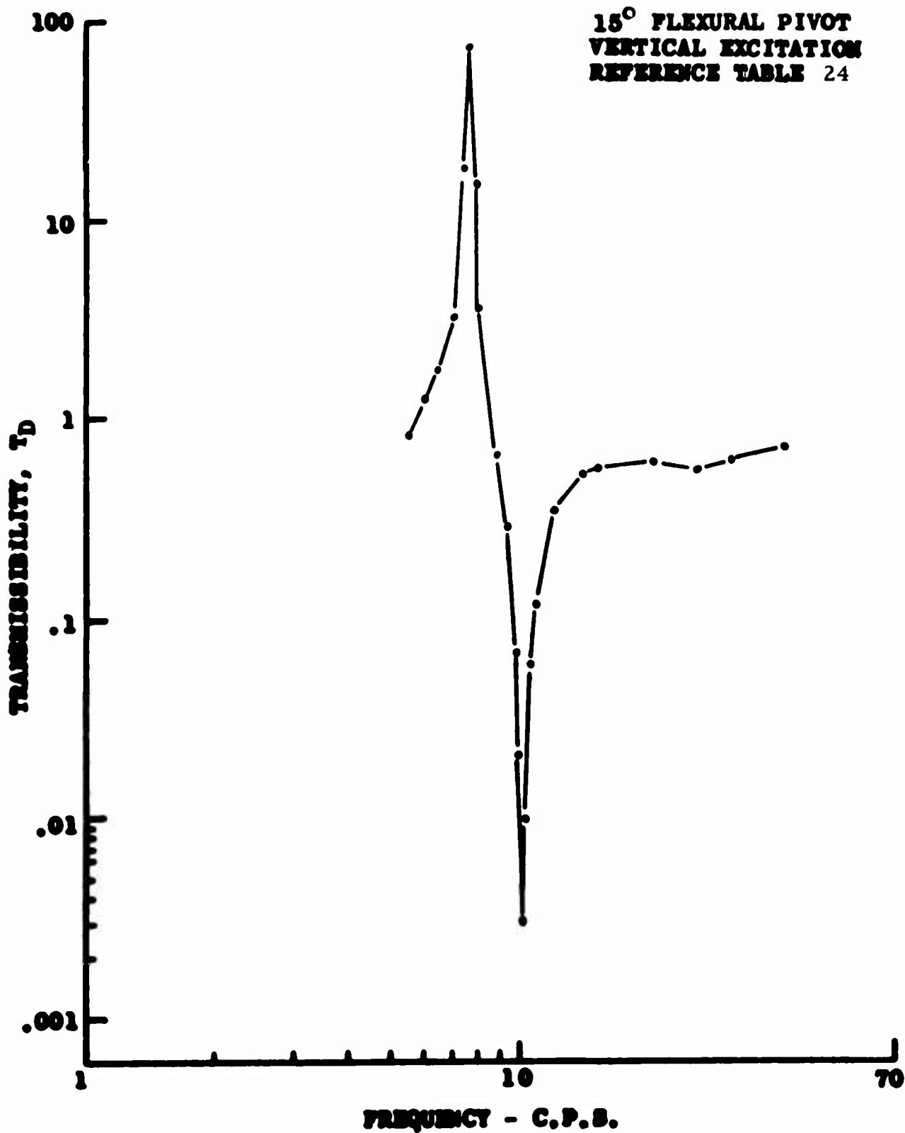
Figure 41. Response Curve for Two-Dimensional DAVI
