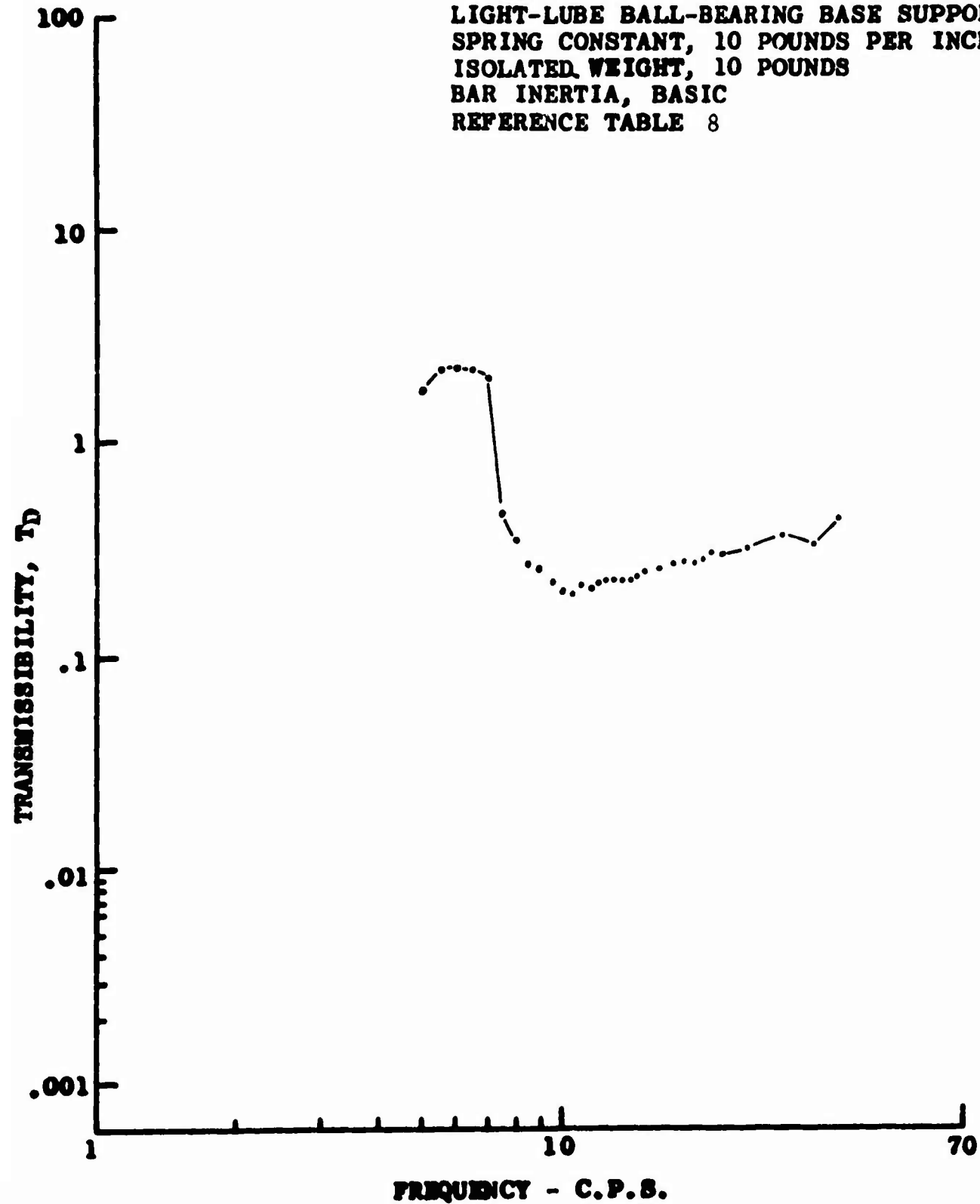
Figure 21. Sliding Pivot Configuration Response Curve
