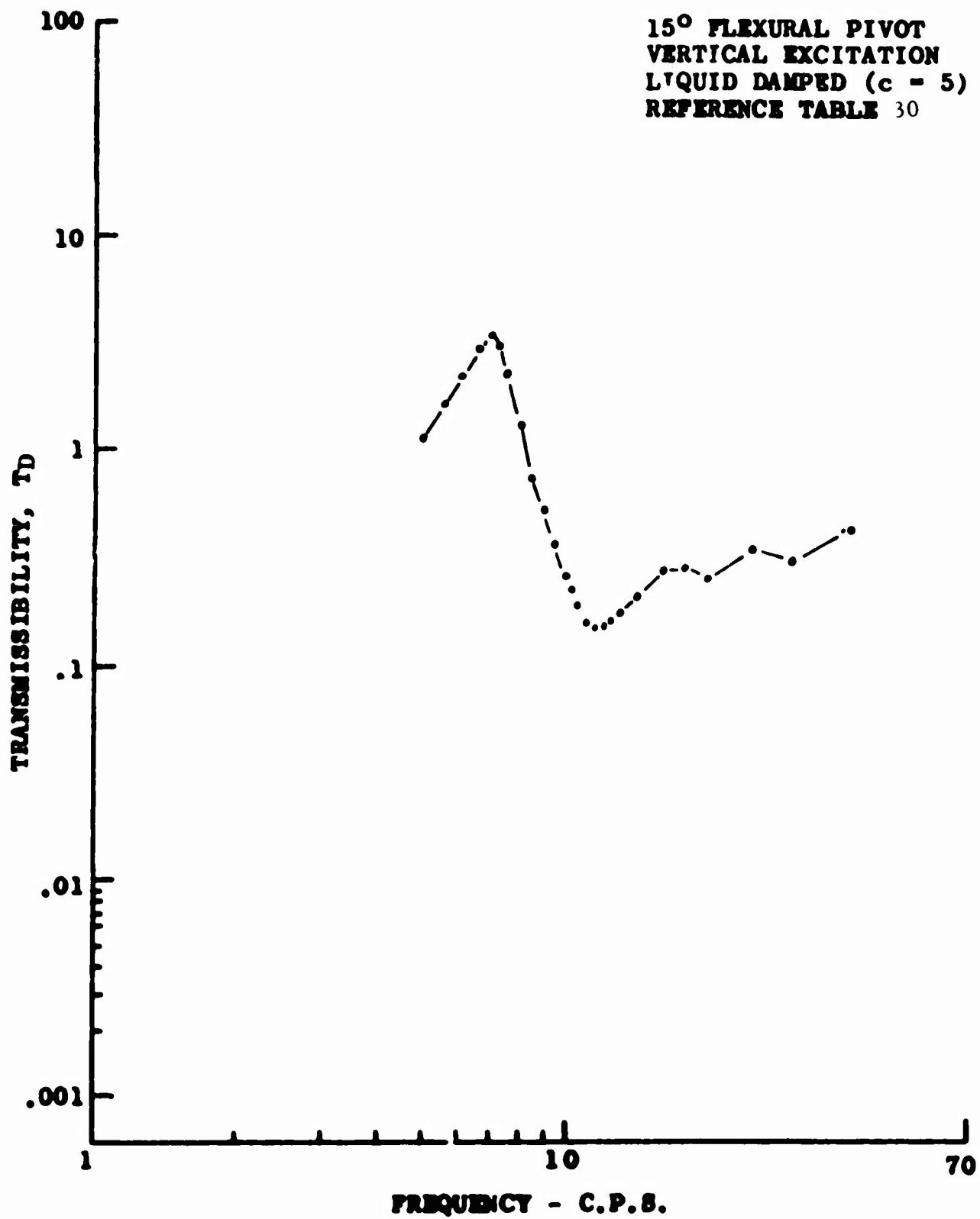
Figure 64. Response Curve for Two-Dimensional DAVI
