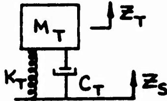
Figure 11. Conventional Isolator
