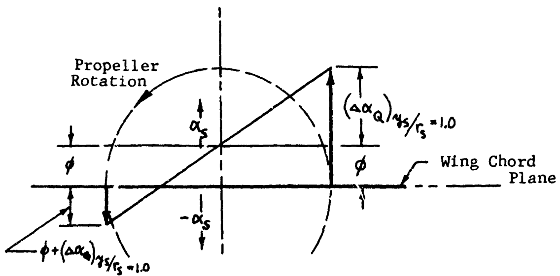
FIGURE 1. Velocity and Angle-of-Attack Distribution of Assumed Slipstream at the Wing.
