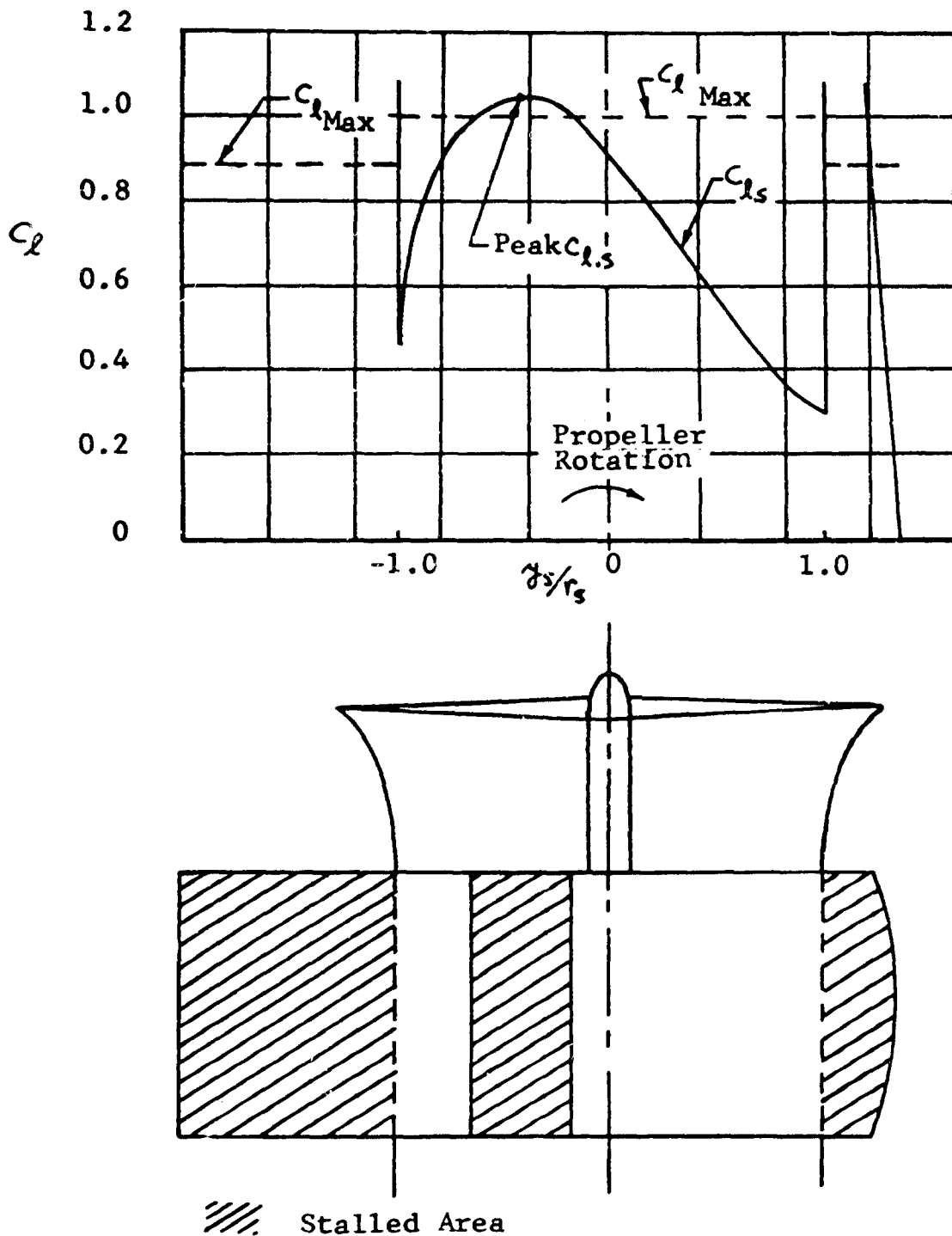
FIGURE 4. Estimated Spanwise Lift Coefficient Distribution and Extent of Wing Stall (Propeller Rotating down at Wing Tip, \alpha_w = 50 Degrees, C_{Ts} = 0.88 , R = 5.0 , NACA 0015 Airfoil Section).
