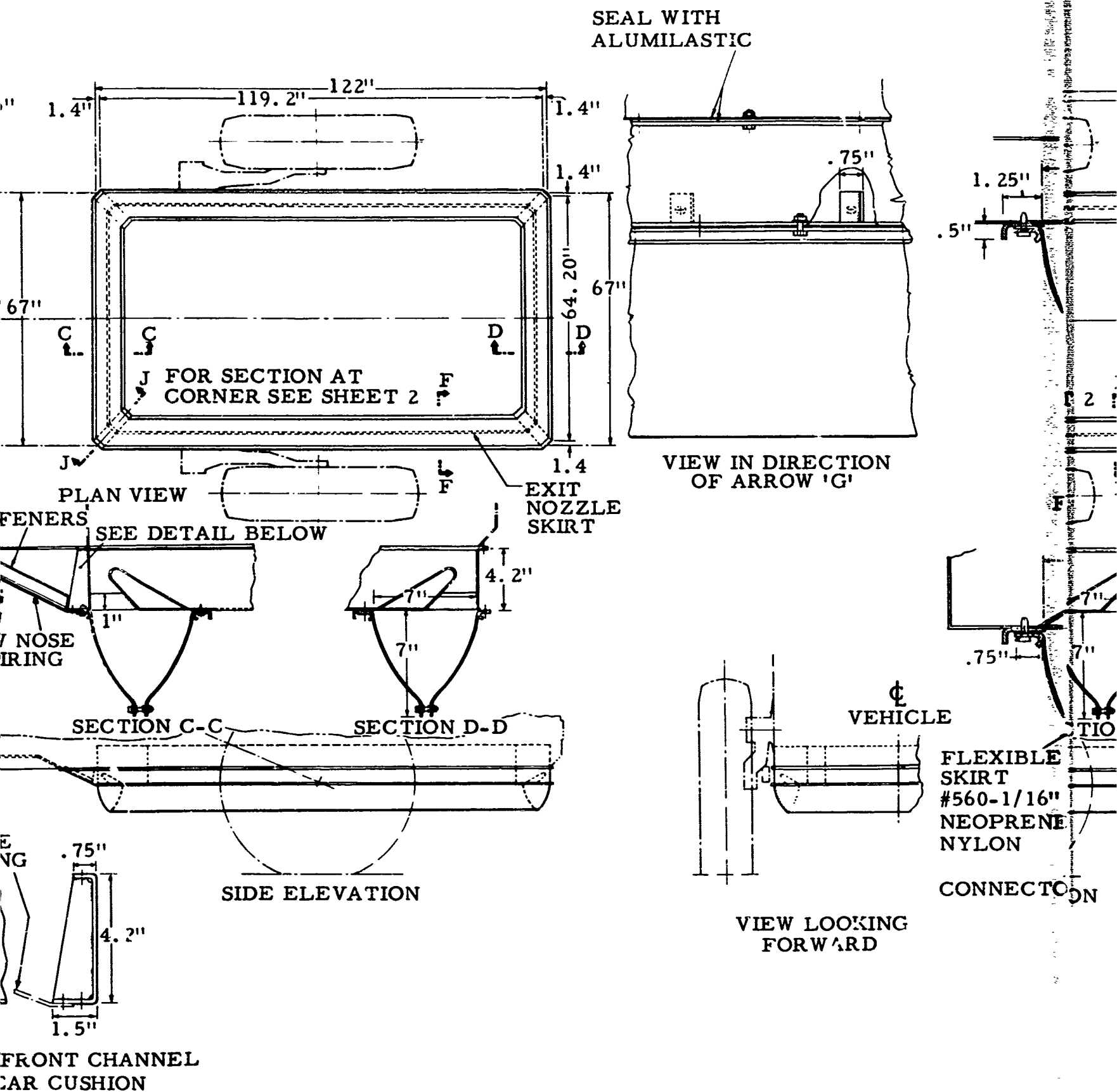
Figure 6. Skirt Type 6D and Attachment to Vehicle (Sheet 1).
