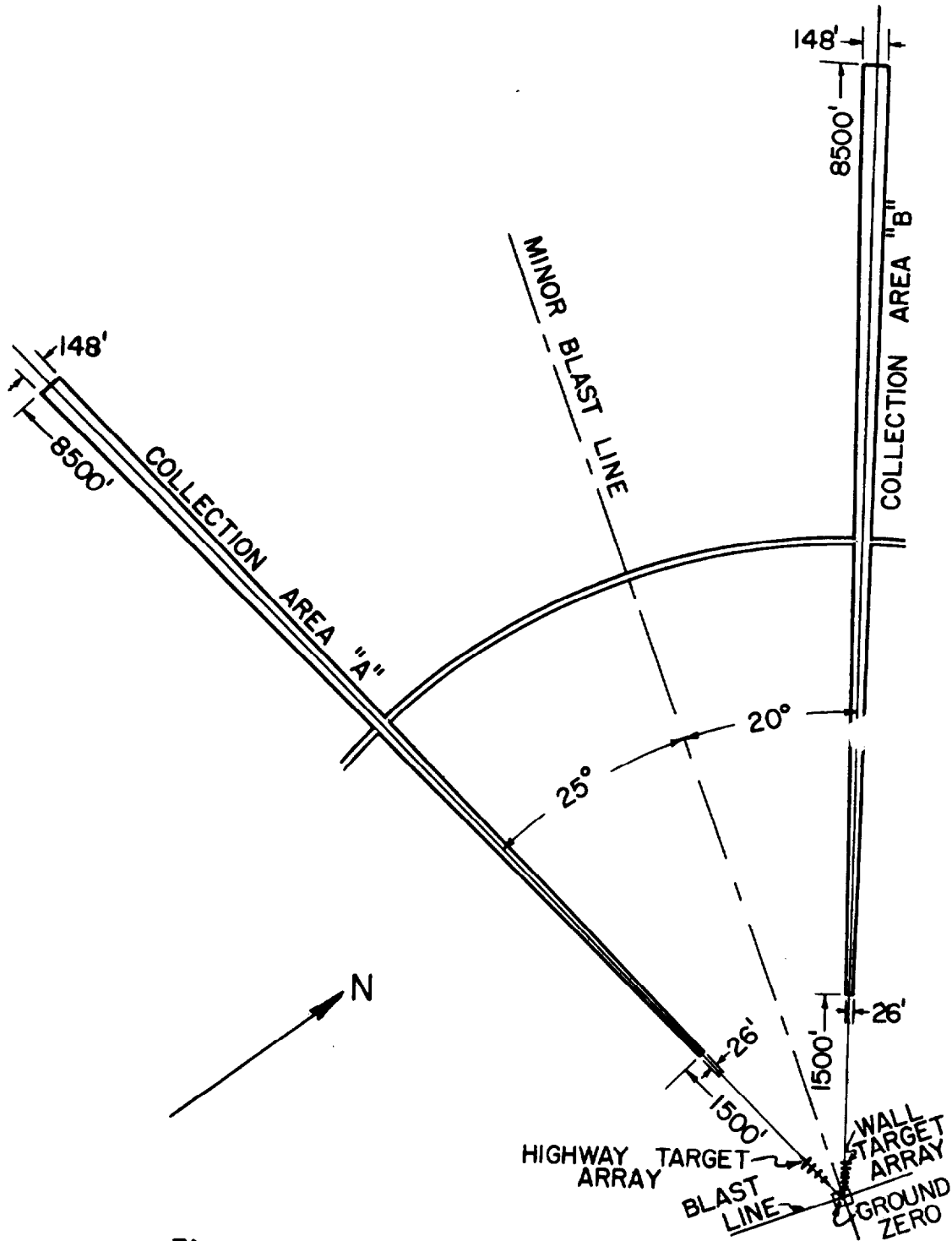
Figure 3.2 Collection Strip Layout
