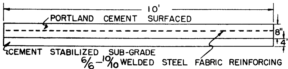
Figure 3.6 Specifications for Wall and Highway Target Construction
