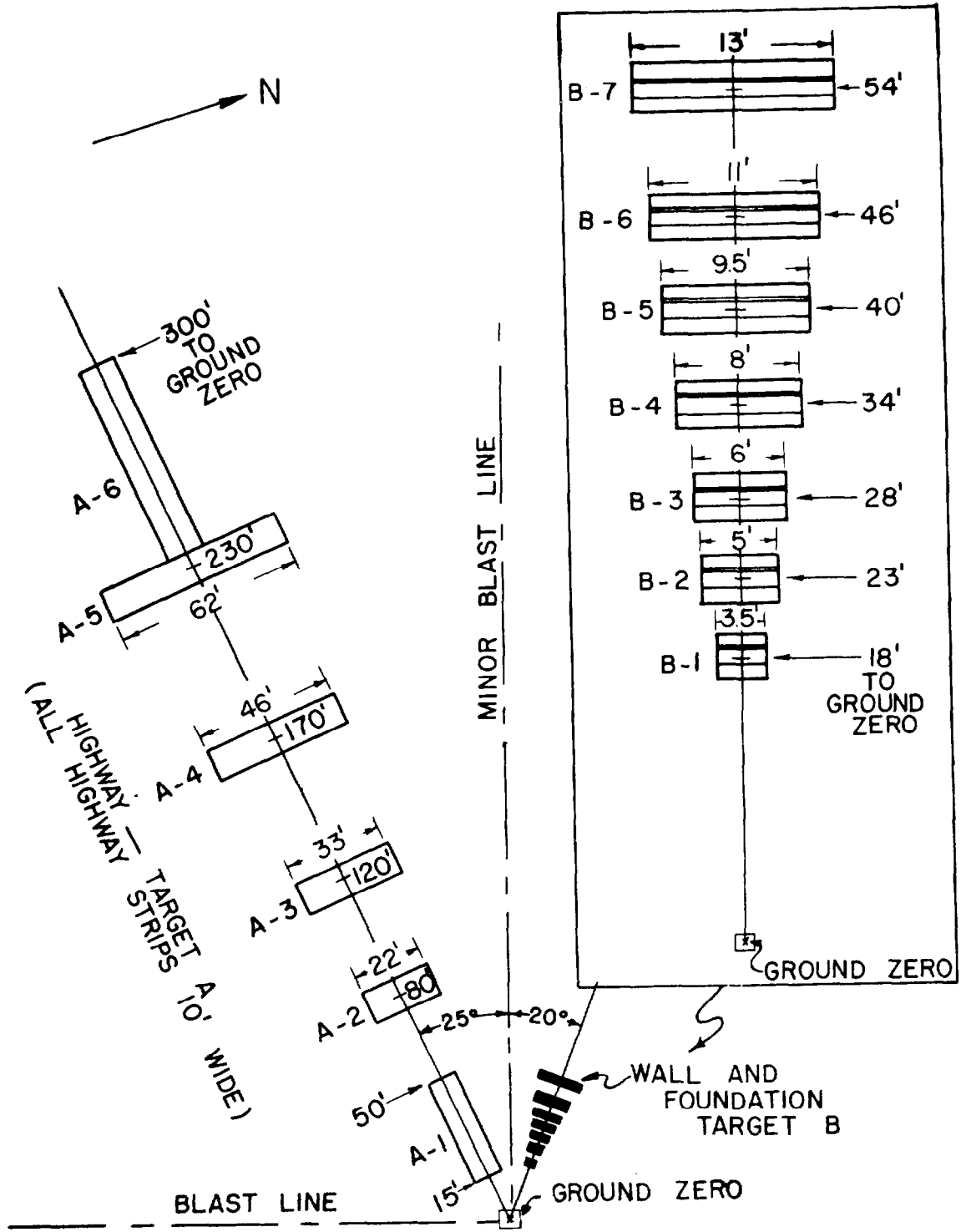
Figure 3.1 Target (Missile Source) Layout
