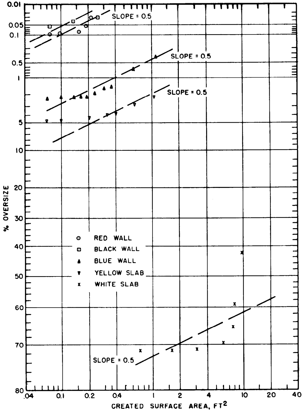
Figure 5.1 Size Distribution of Missiles. Theoretical Slope = 0.5
