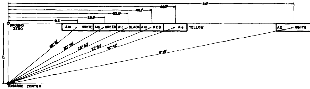
Figure 5.2 Elevation of Highway Slab Targets A-1 and A-2
