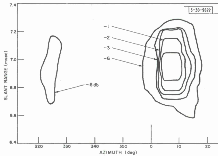
Fig. V-16. Distribution of L-band auroral echo intensity at 2.0° elevation, showing 1-, 2-, 3-, and 6-db contours.
