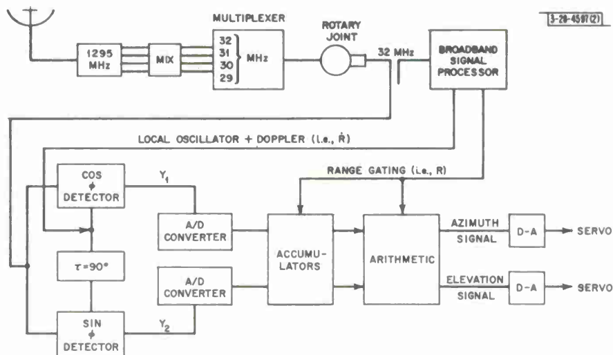
Fig. II-6. Digital monopulse tracking system.
