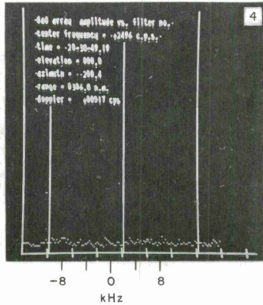
Fig. II-4. Calliscope displays of Trailblazer spectra obtained during re-entry phase. Frames 1 and 2 show (a) Doppler-spread echo and (b) higher velocity, hard-target type echo. In Frame 3 only the Doppler-spread echo remains. No echoes can be seen in Frame 4.
