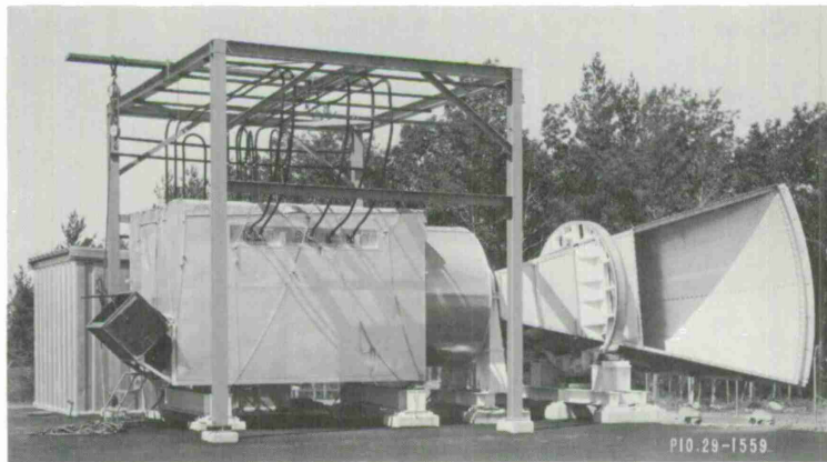
Fig. III-2. Radiometer box installed on cornucopia standard-gain antenna.
