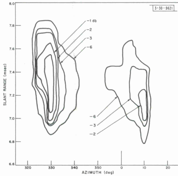
Fig. V-15. Distribution of L-band auroral echo intensity at 1.5° elevation, showing 1-, 2-, 3-, and 6-db contours.
