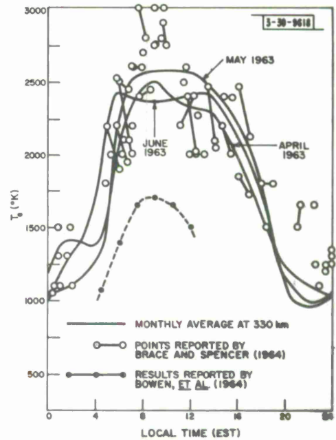
Fig. V-12. Comparison of radar and satellite determinations of electron temperature. Points reported by Brace and Spencer 24 were for altitudes in 260- to 400-km range, hence a curve corresponding to 330 km has been drawn to represent radar results.
