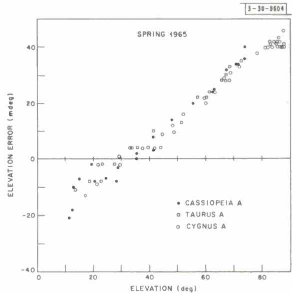
Fig. III-14. Haystack pointing calibration.
