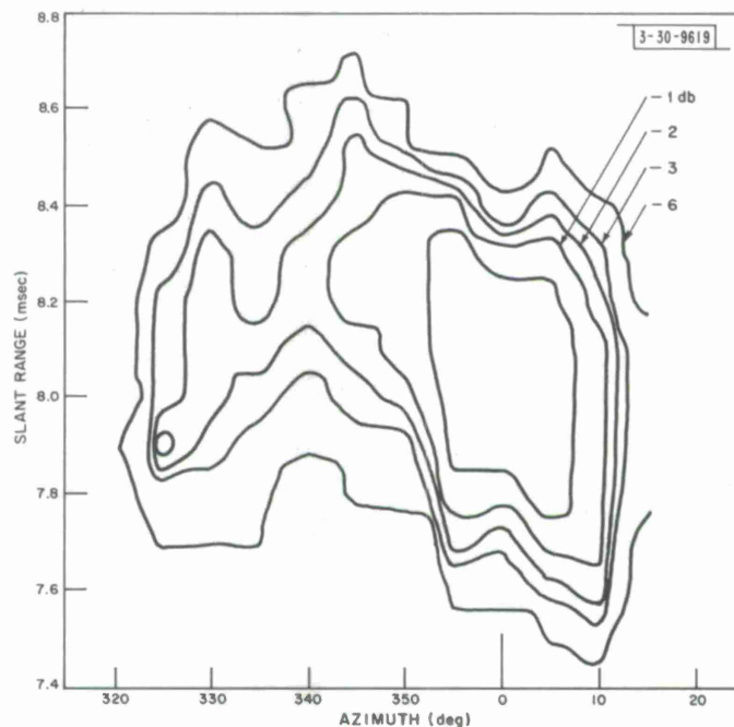
Fig. V-13. Distribution of L-band auroral echo intensity at 0.5° elevation, showing 1-, 2-, 3-, and 6-db contours.
