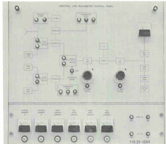
Fig. III-9. Spectral line radiometer control panel.
