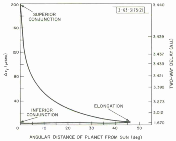
Fig. IV-15. Relativistic effect on Earth-Venus time delays.
