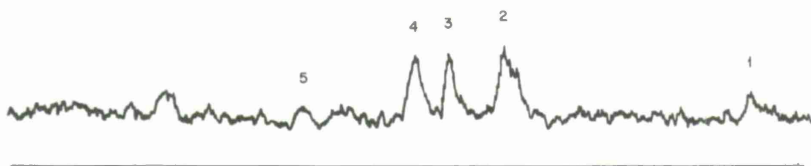
Fig. II-8. Weak targets in the orbit of the first West Ford launch detected in February 1962 with the Millstone UHF radar, using incoherent integration. (Integration period: 5 seconds.)
