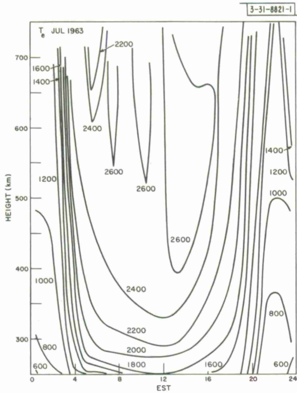
Fig. V-11. Variation of electron temperature as a function of height and time obtained by averaging all results for July 1963.
