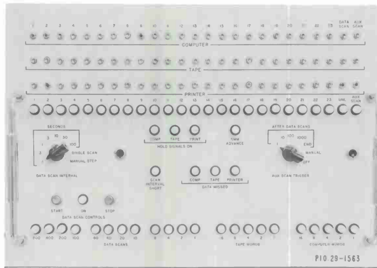
Fig. III-8. Radiometer system, data control panel.
