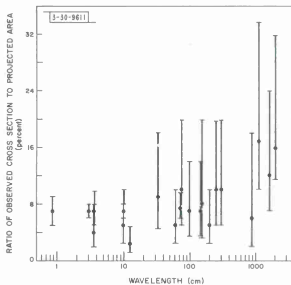
Fig. IV-7. Various experimental determinations of lunar cross section.
