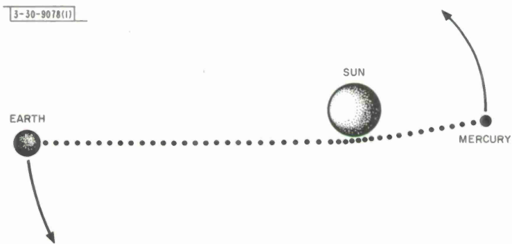
Fig. IV-13. Relativistic effect on electromagnetic wave propagation.
