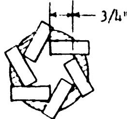
f) Inlet Bushing Positions for e); 2 Rows of 6 Inlets Each
