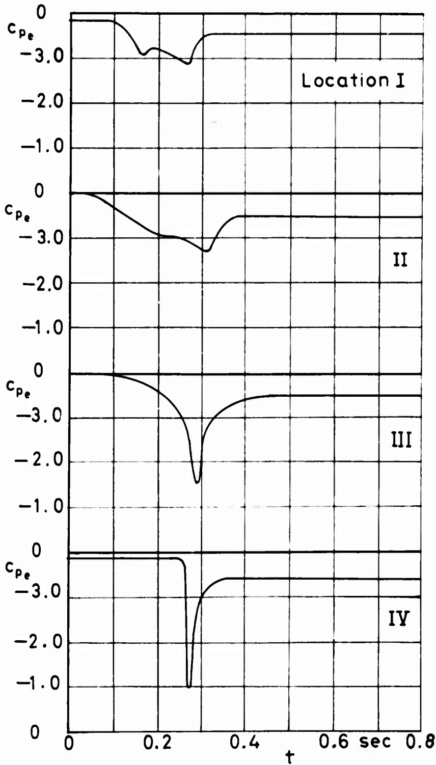
Figure 22 c_{pe} and filling versus time v_0 = 100 ft/sec Run No 226
