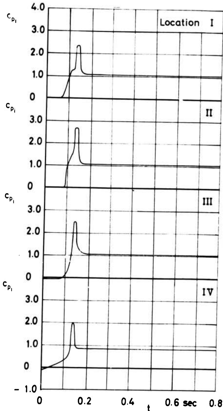
Figure 14 c_{pi} and filling versus time
