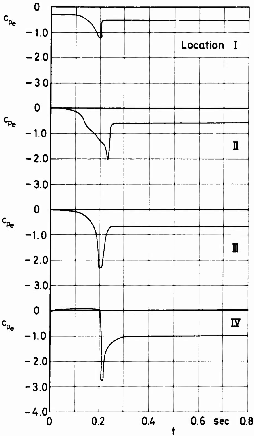
Figure 12 c_{pe} and filling versus time
