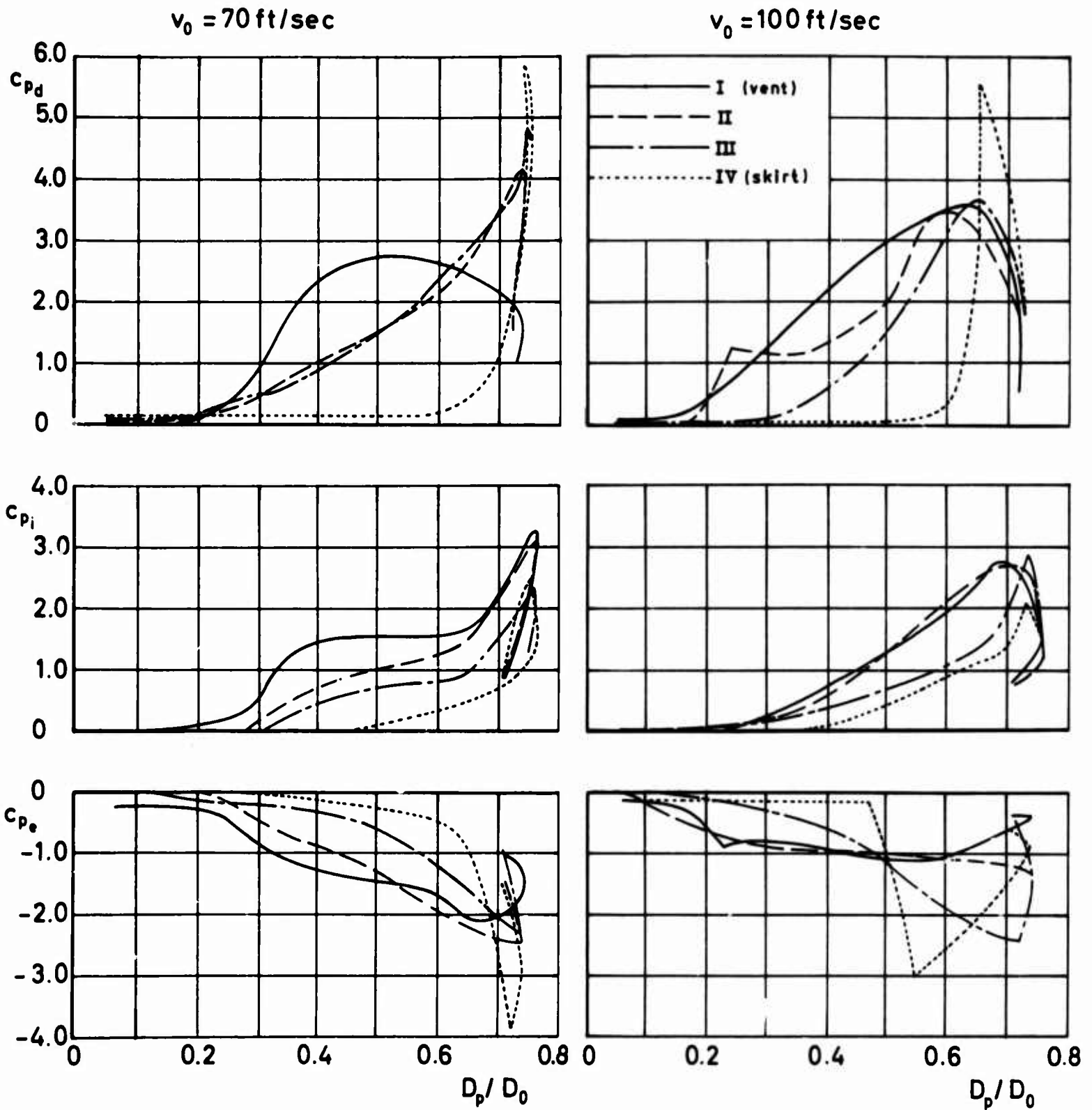
Figure 55 c_p versus D_p/D_0 for Extended Skirt
