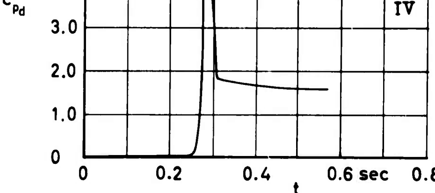
Figure 20 c_{pD} and filling versus time
