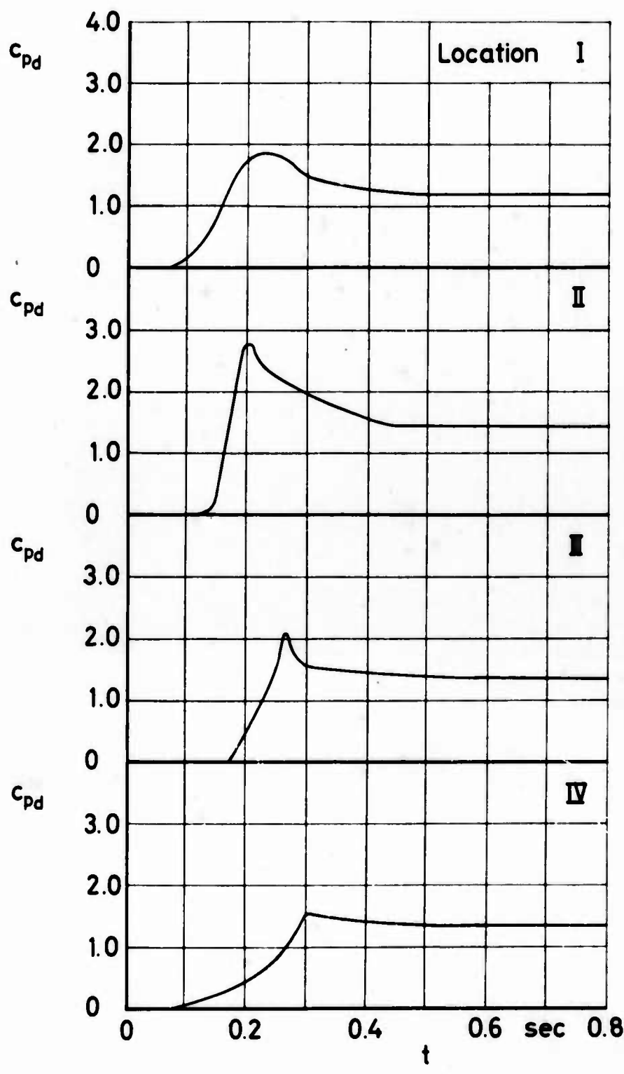
Figure 104 c_{pd} and filling versus time
