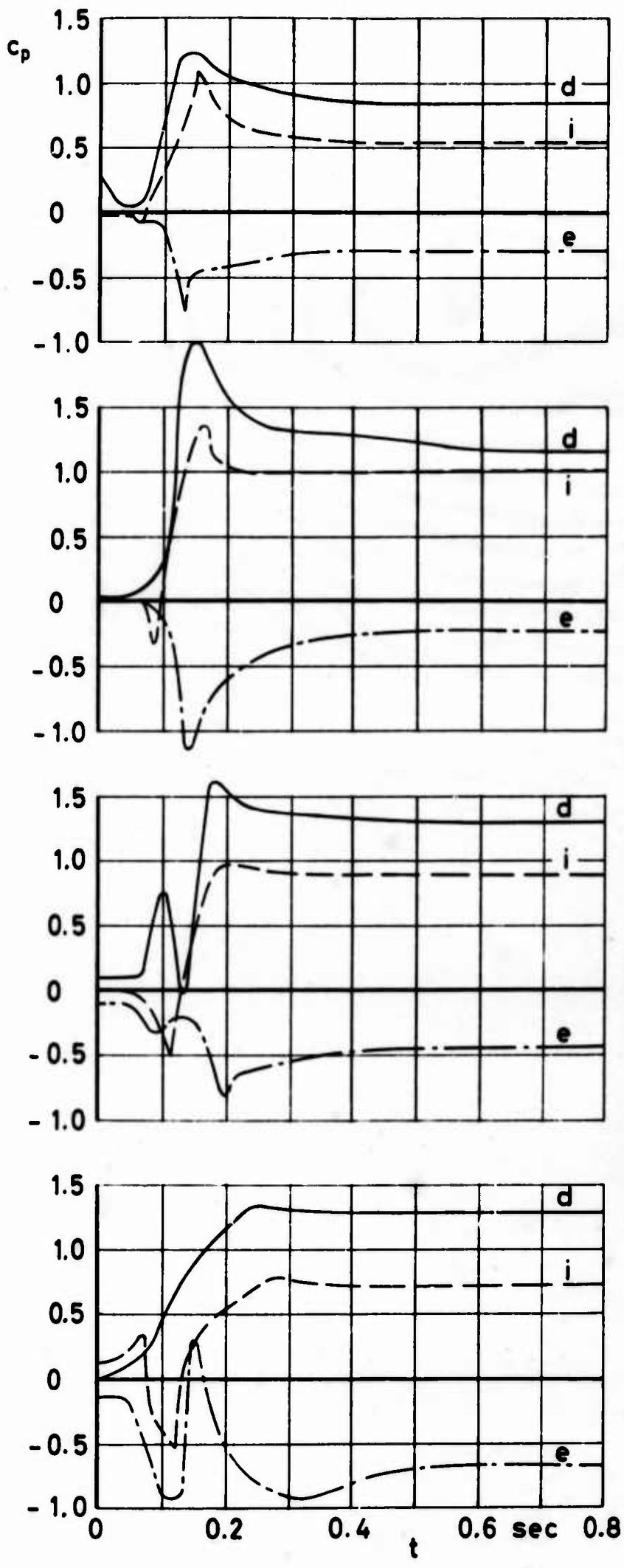
Figure 101 C_p versus time for differential, internal and external pressure
