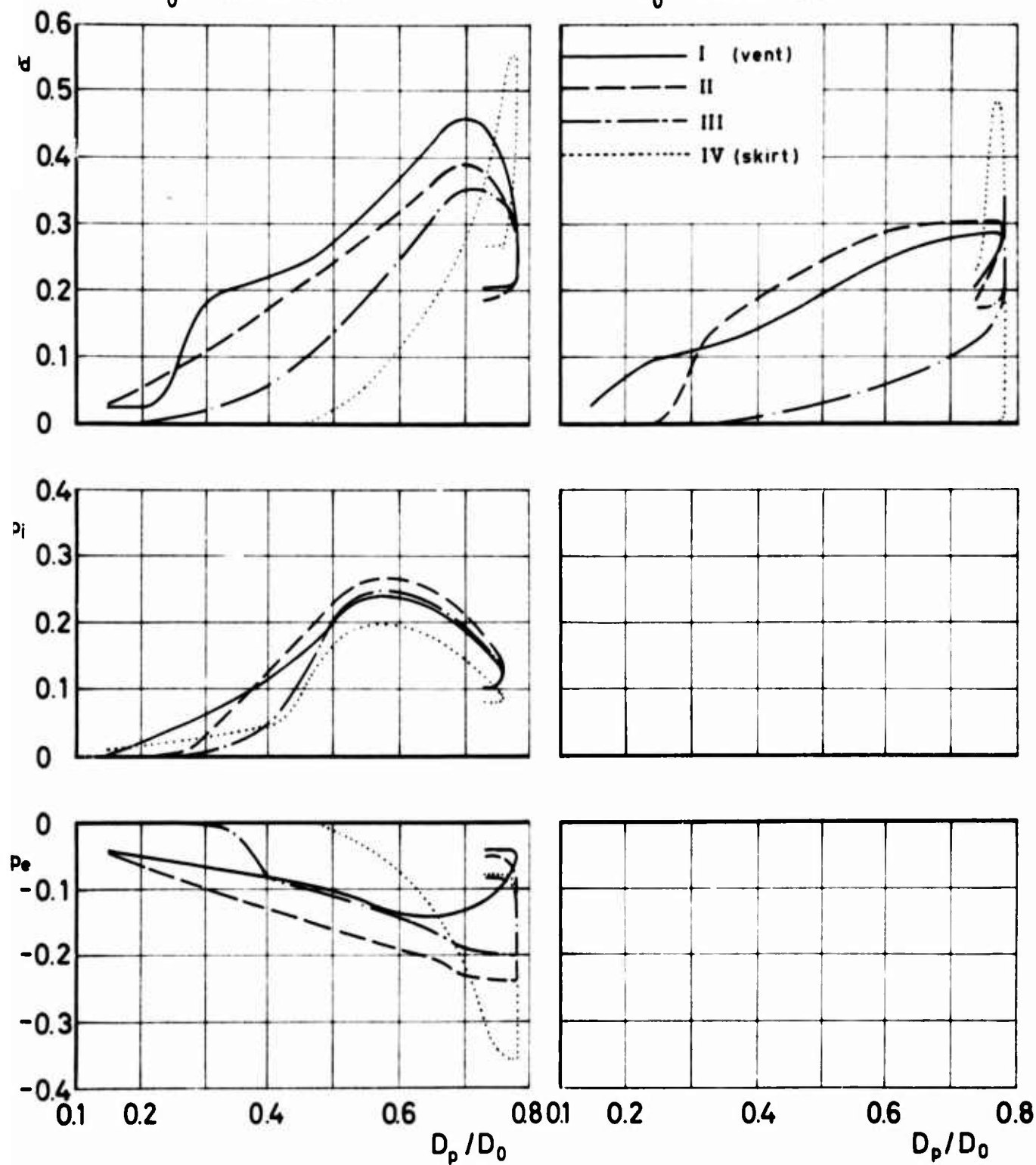
Figure 54 c_p versus D_p/D_0 for Circular Flat
