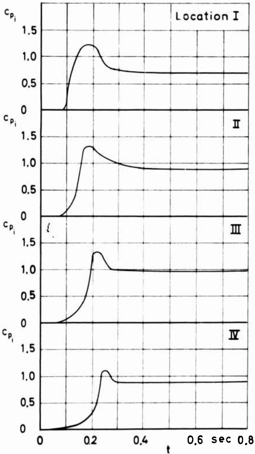
Figure 36 c_{p_i} and filling versus time v_0 = 130 ft/sec Run No 92
