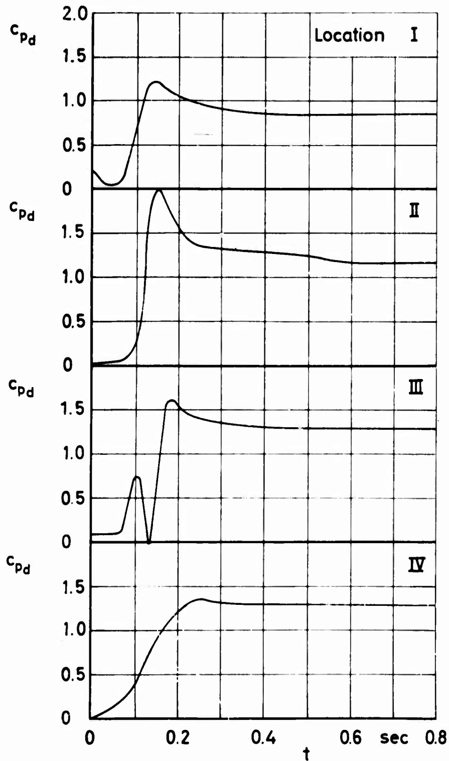
Figure 47 c_{pd} and filling versus time
