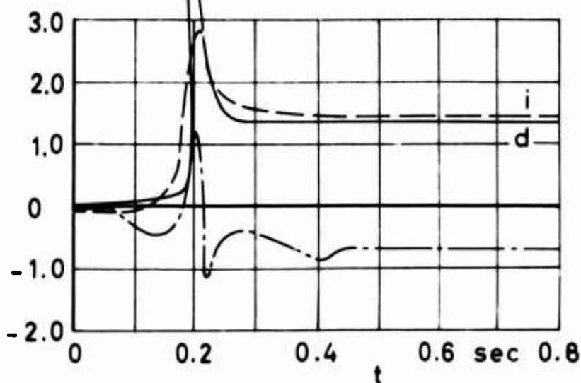
Figure 94 c_p versus time for differential, internal and external pressure
