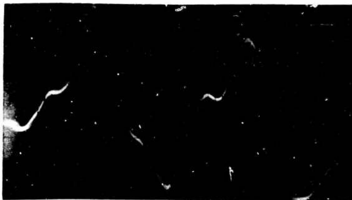
Figure 77. Current Waveform Change Due to Removing One Probe from Measuring Circuit, Horizontal Sweep Speed - 10 nsec/cm, Vertical Sensitivity - 200 v/cm
