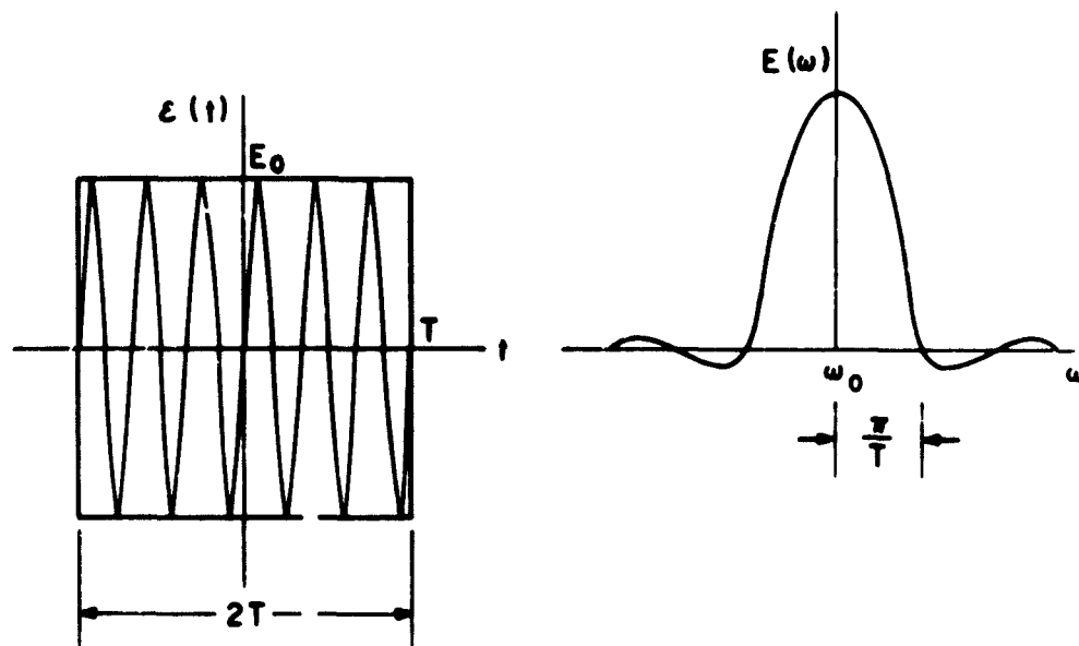
FIG. 1b RECTANGULAR ENVELOPE CARRIER PULSE
