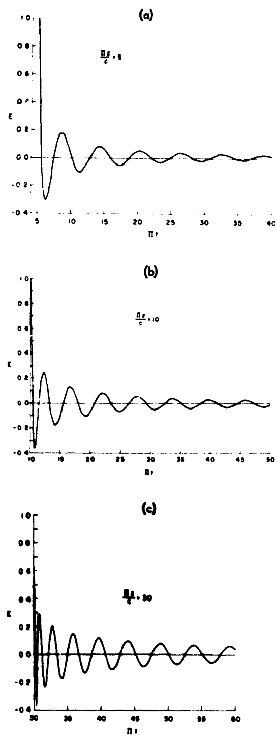
Figure 8. Propagation of a Step Function Electric Field in a Plasma
