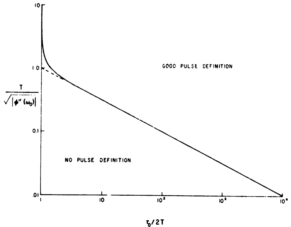
Figure 5. Regions of Good Pulse Definition and No Pulse Definition
