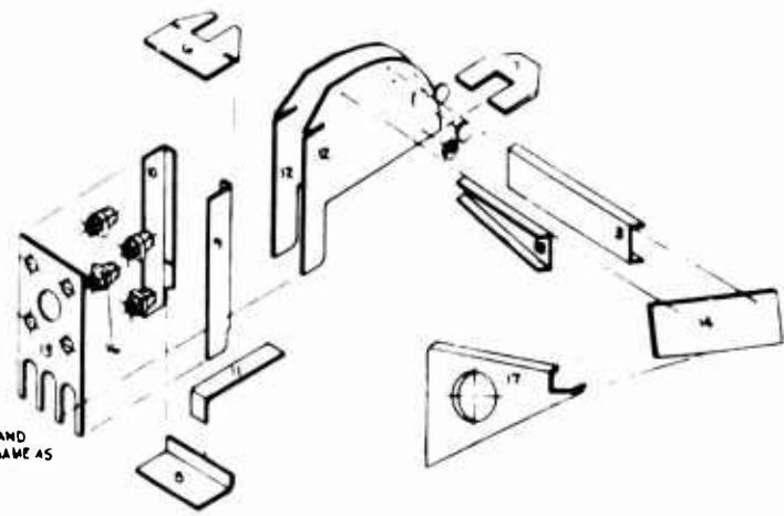
SCHEMATIC EXPLODED VIEW OF GROUP 2
