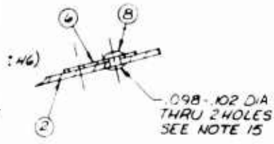
VIEW D (ZONE H-7) SCALE 2/1
