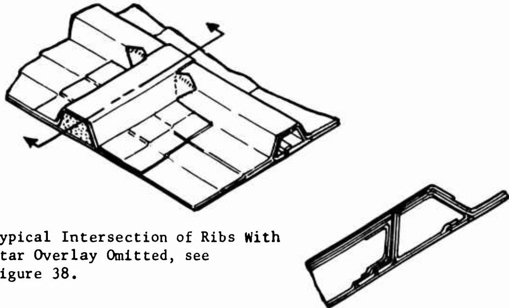
Figure 37. Showing Typical Joint Construction Used in the Manufacturing of the Dome.
