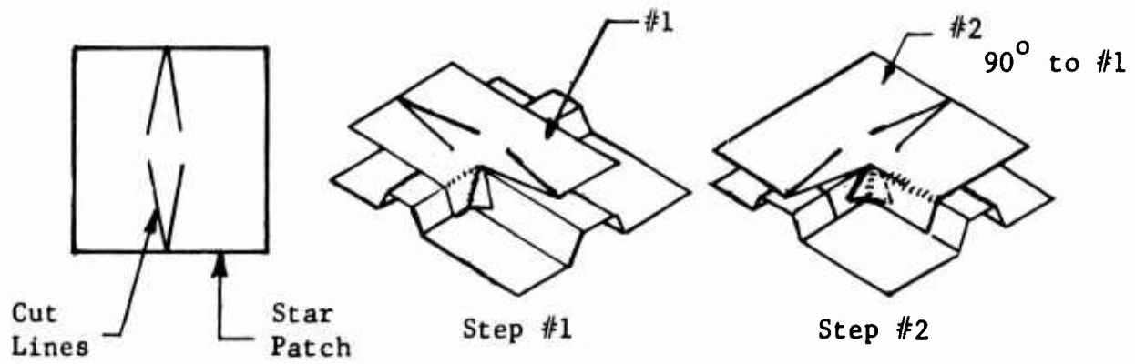
Figure 38. Showing Typical Star Lay-up Over Rib Junctions Reinforcing the Joint.
