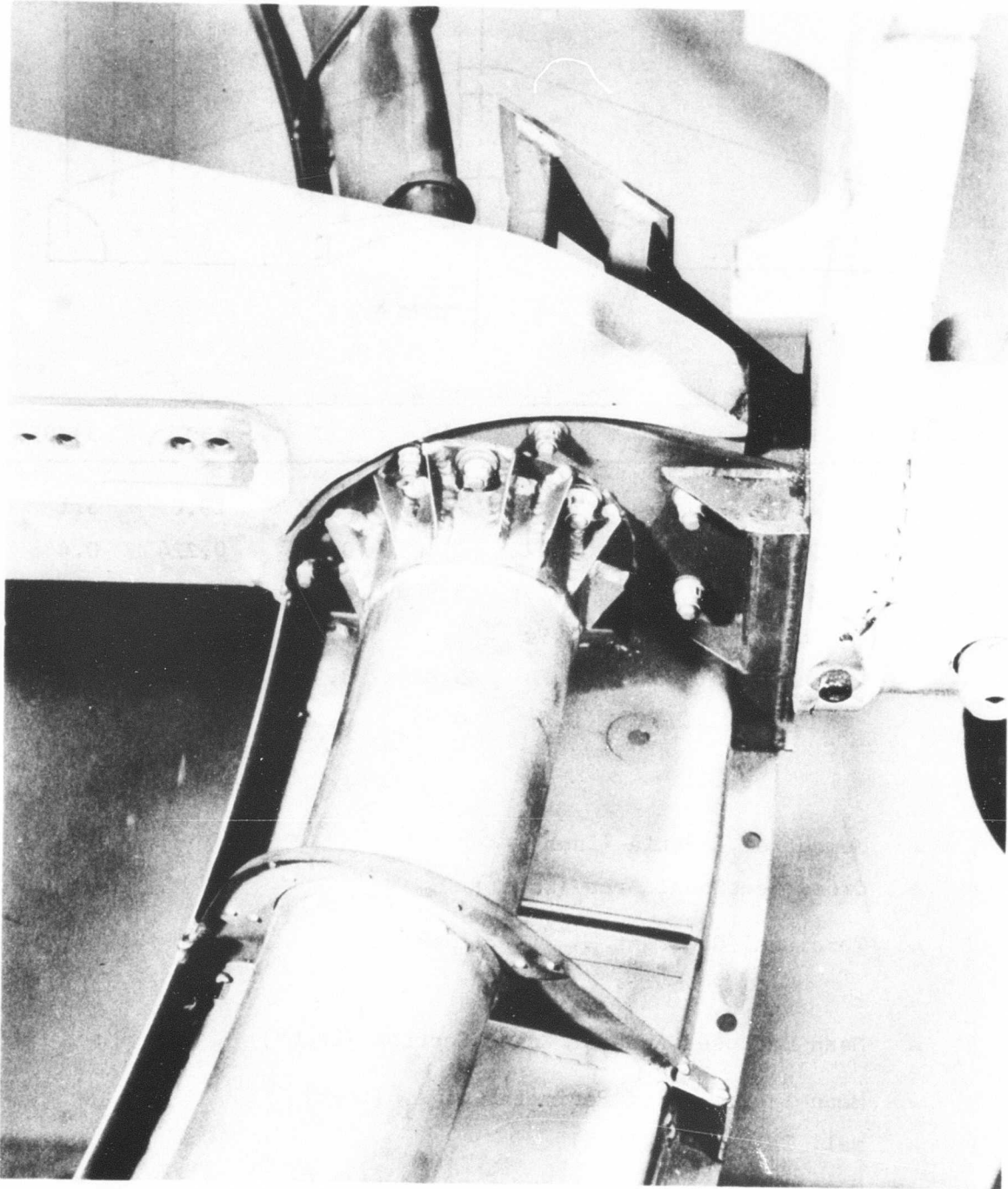
Figure 21. LF-2 Front Frame View Showing Attachment of the Al10AT Titanium Cold-Side Sector and 17-4 PH End Cap to the 12 to 6 O'clock Cast A356T1 Aluminum Strut.
