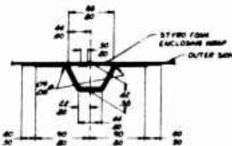
SECTION K-K (ENL. 1/2) SCALE 1/2 STYRO FOAM CONSTRUCTION NOTE: ALL LINES TO BE COVERED, SEE EXAMPLE U-U, POINT TO CORNER WITH ENCLOSING MESH
