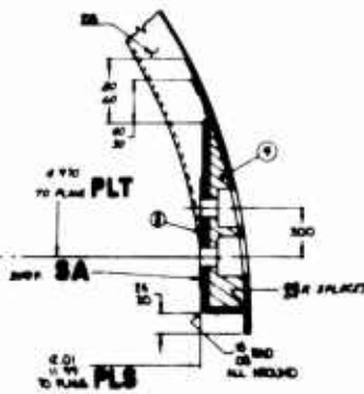
SECTION A-A (EDGE B1) SCALE 1/2" TYPICAL 8 PLACES SEE ILLUSTRATION, EXAMPLE P-10
