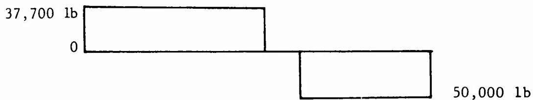
c) Shear Diagram
