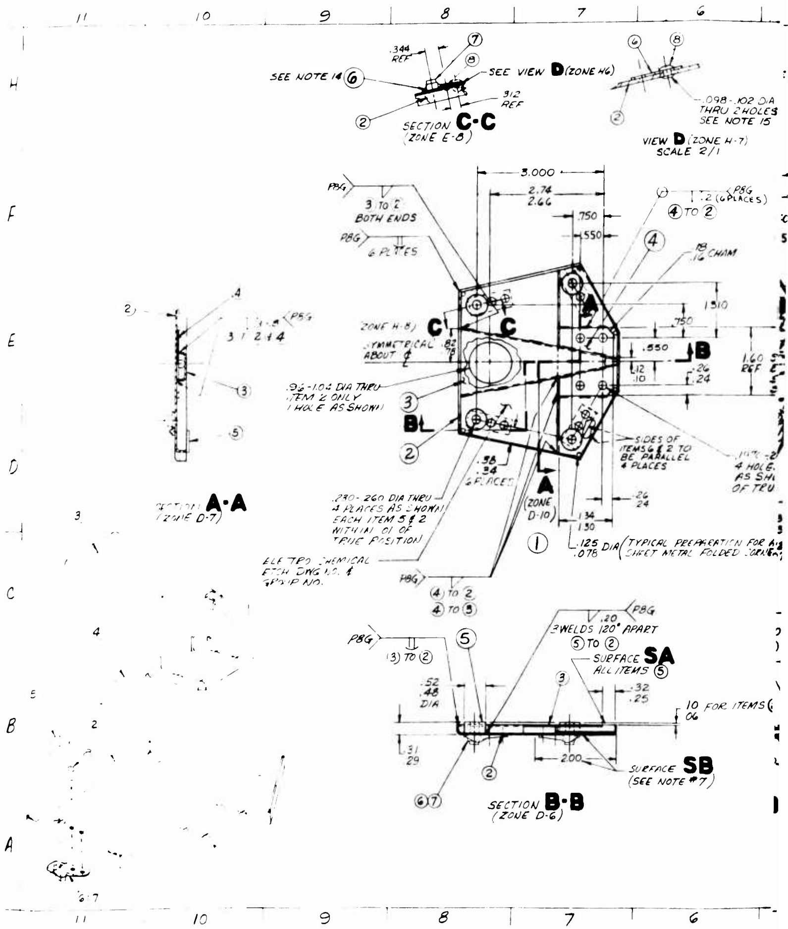
Figure 13. Drawing 4012001-3873
