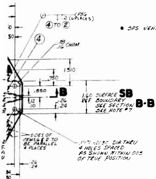
VIEW D (ZONE H-7) SCALE 2/1
