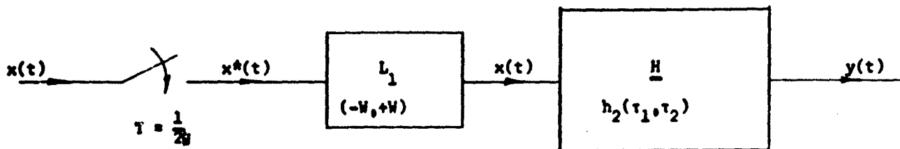
Fig. 27. Bandlimited system with bandlimited input.
