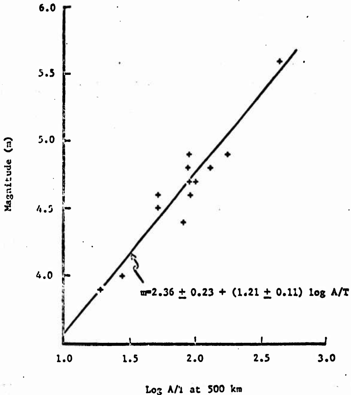
Magnitude from teleseismic stations (dist. \geq 16^\circ ) versus logarithm of amplitude divided by period (A/T) at 500 km, based on nuclear explosions at the Nevada Test Site and SHOAL (Fallon, Nevada).
