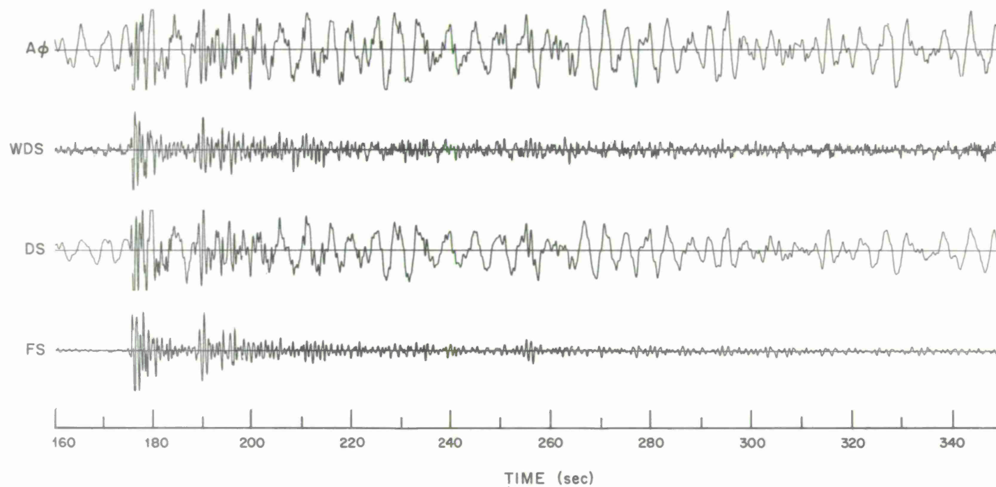
Figure 6. Processed traces obtained by time-domain synthesis procedure, 11/11/65 Rat Island event, subarray Aφ, NIM = 2, NFP = 21, 3 minute fitting interval.
