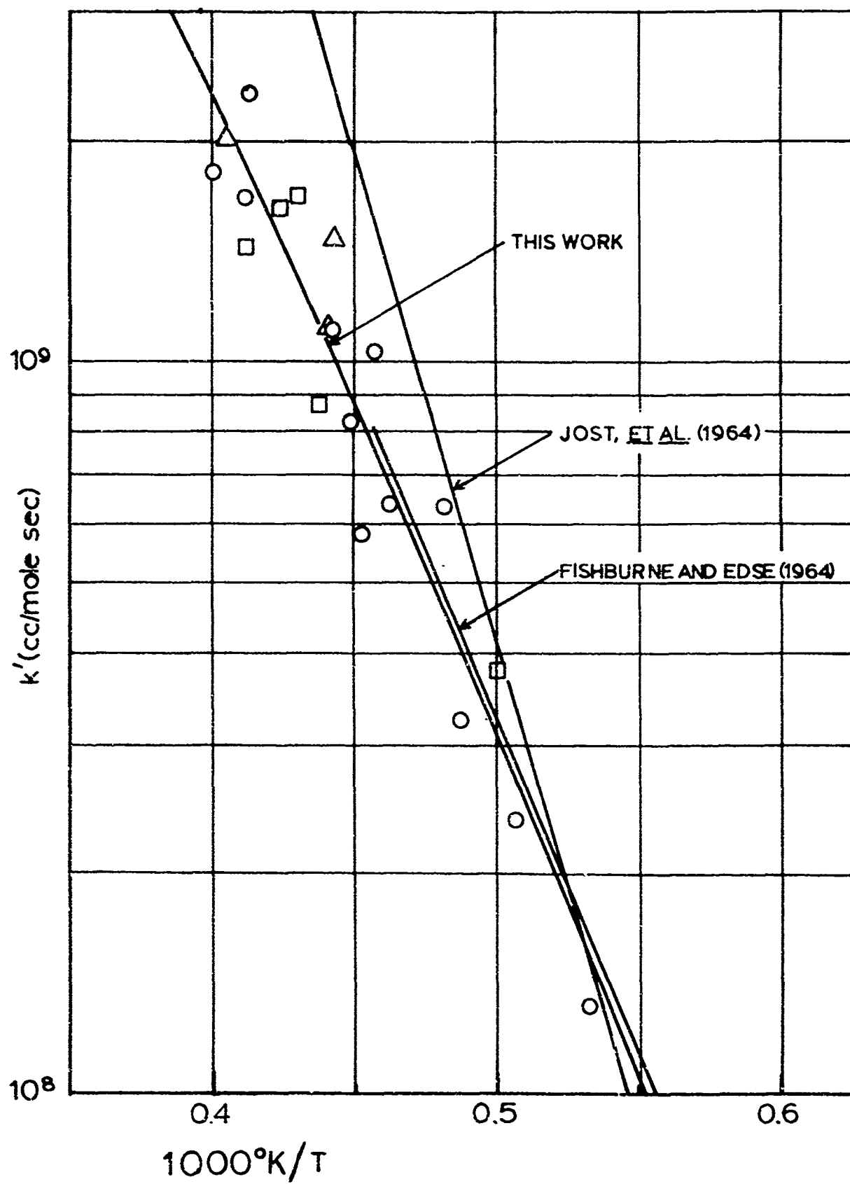
FIG. 5.5 THERMAL DECOMPOSITION RATE OF \text{H}_2\text{O} (AND EXTENDED BELOW 1000°K)
