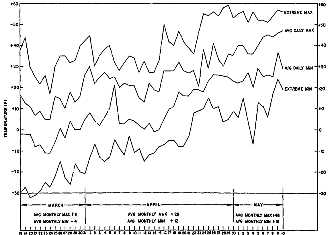
PAST TEMPERATURE MEANS FOR THE SIX YEAR PERIOD 1952-1957 AT SONDRESTROM AIR BASE
