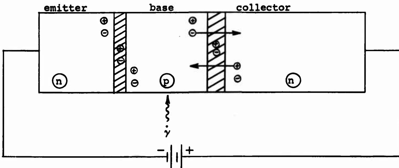
Figure 4. Open Base Transistor Under Irradiation
