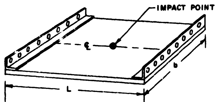
Figure 12. Bottom Panel Geometry (.30 and .50 Caliber).
