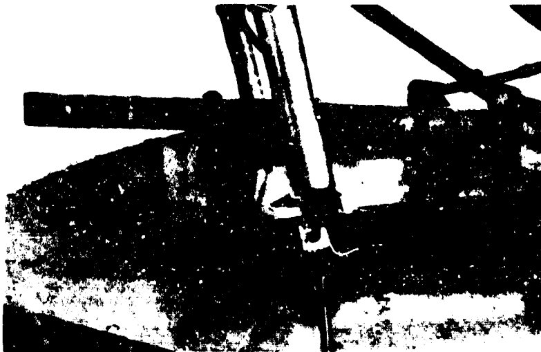
Figure 20. Result of Sideward-Load Application (Note Tear-Out at Track Rail; Failure Load, 4,800 Pounds).
