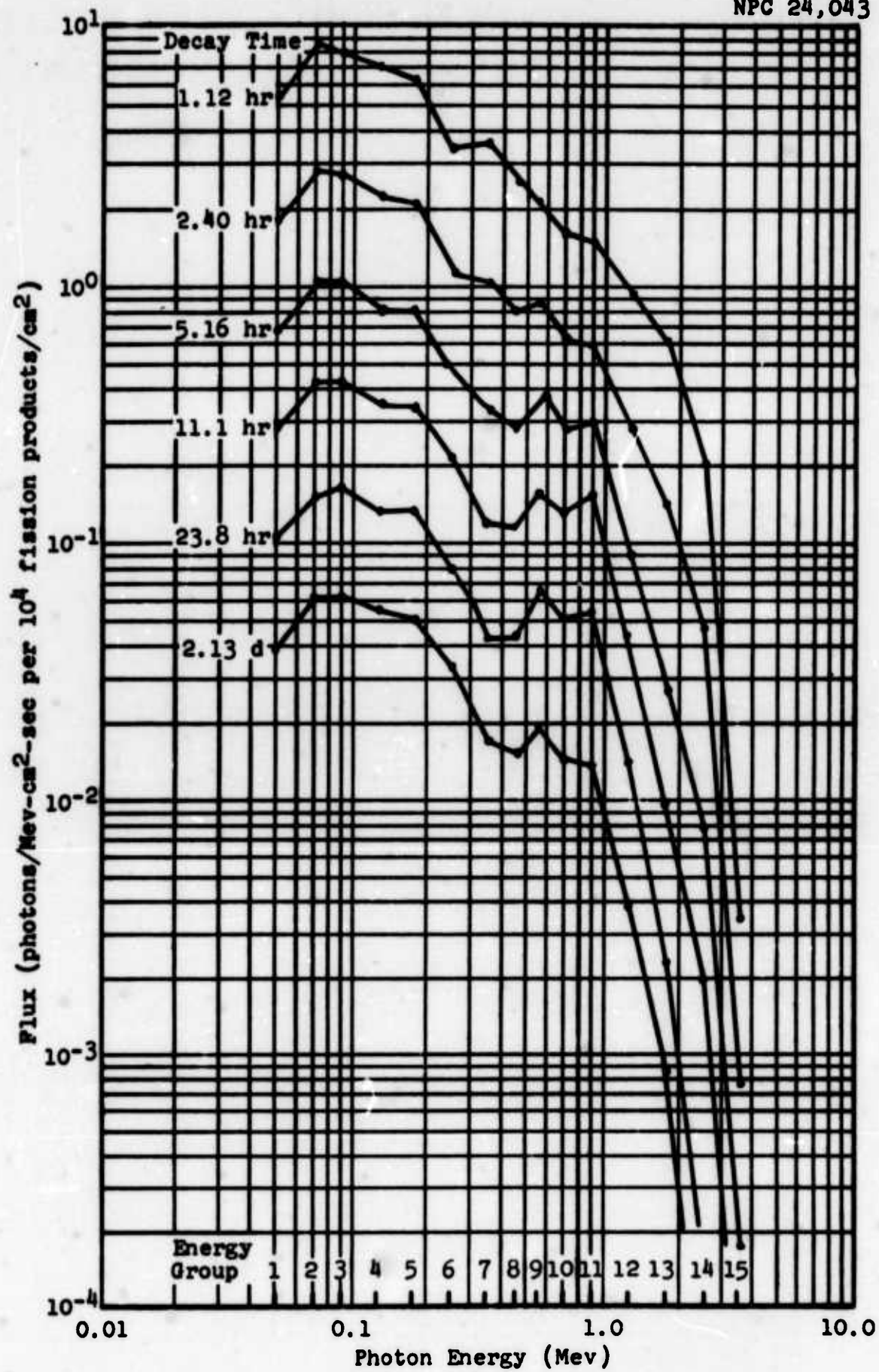
Figure 4.1 Number Spectra: Altitude, 3 Feet (figure continued on next page)
