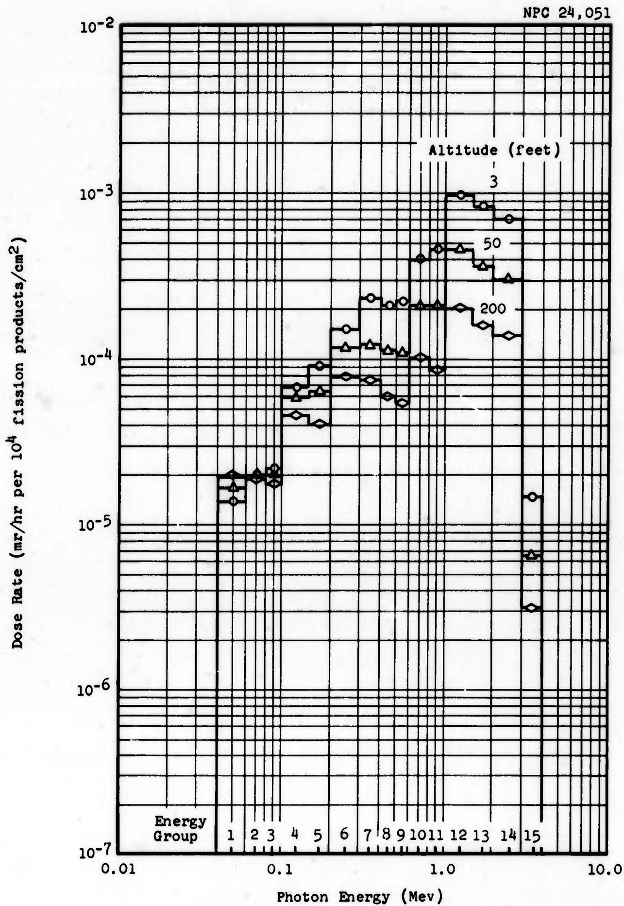
Figure 4.7 Multigroup Dose-Rate Spectra: Time, 1.12 Hours
