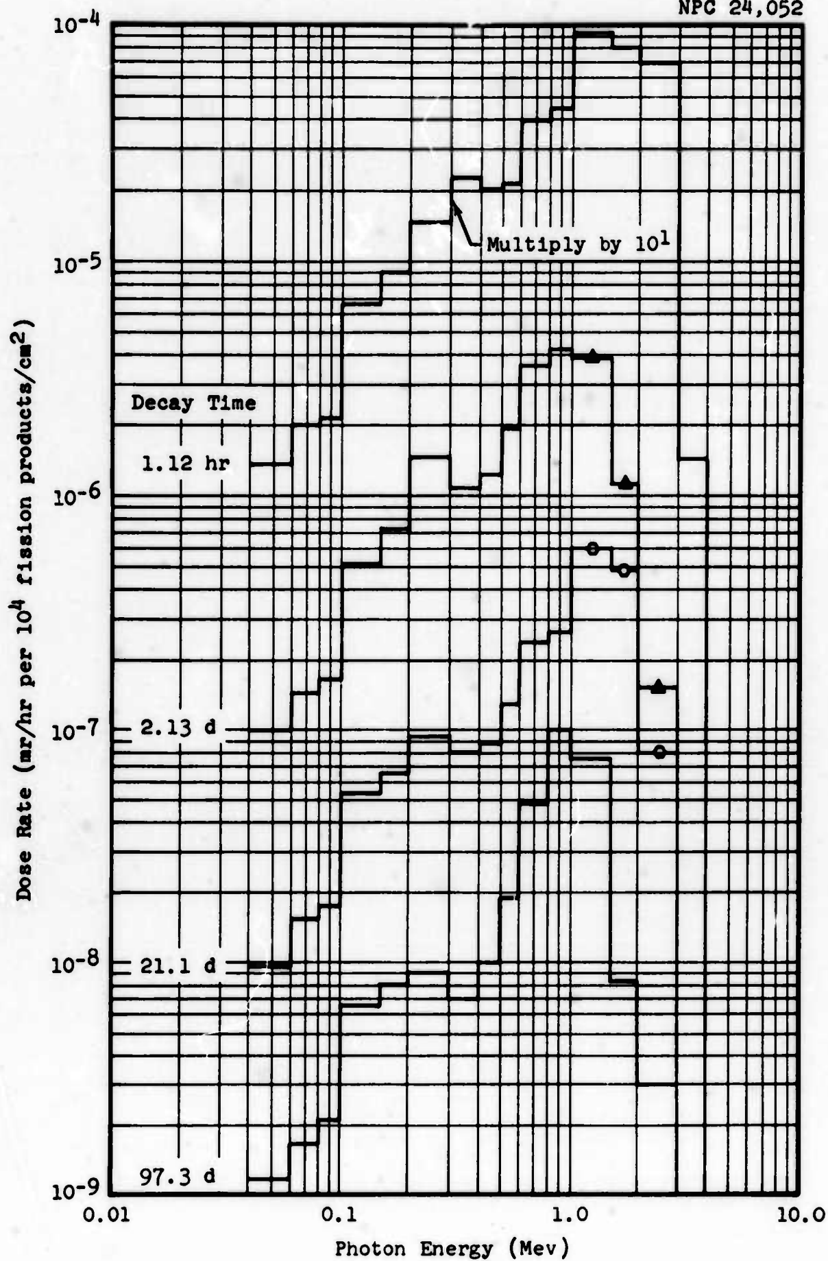
Figure 4.8 Multigroup Dose-Rate Spectra: Altitude, 3 Feet
