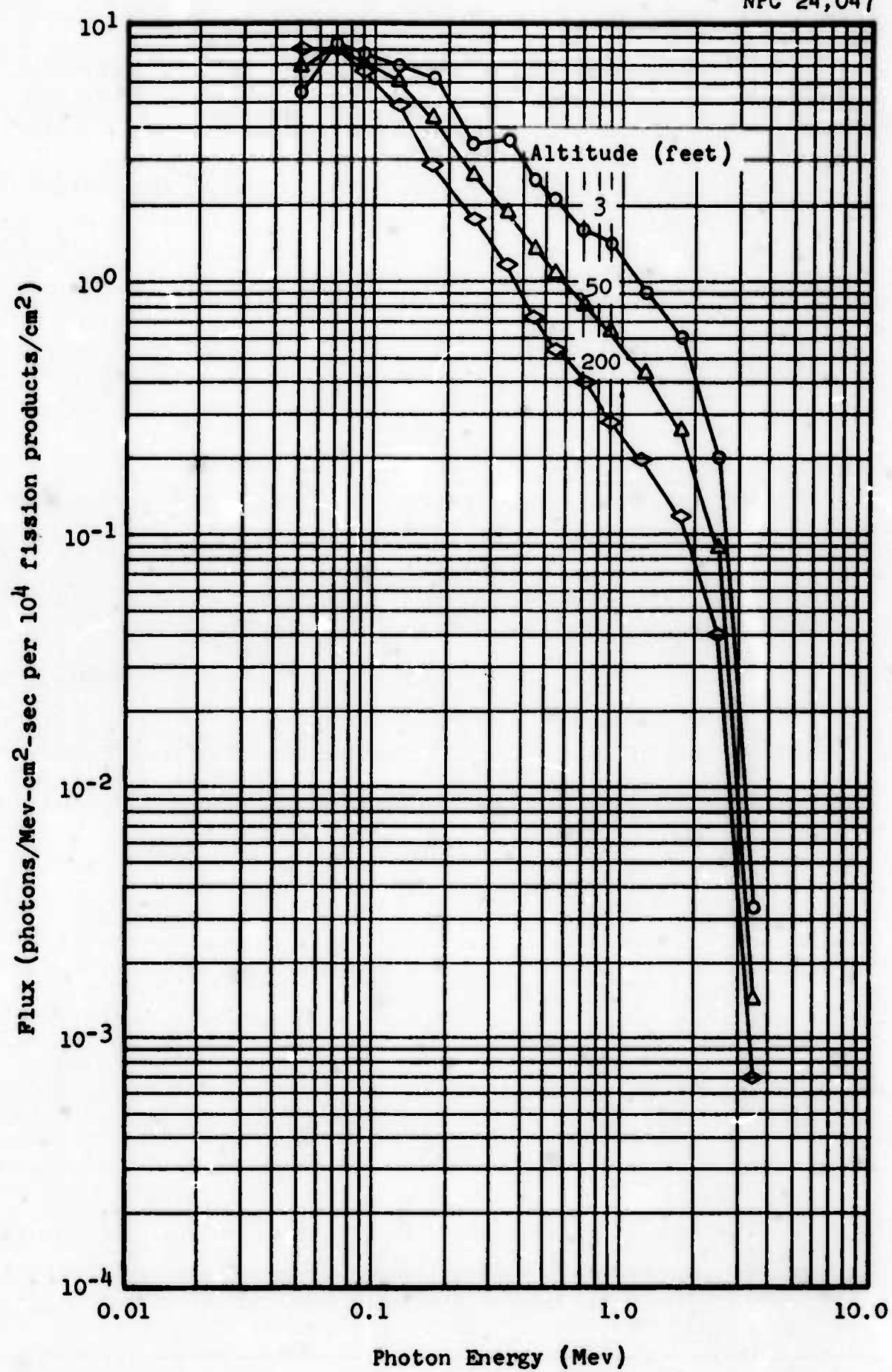
Figure 4.3 Number Spectra: Decay Time, 1.12 Hours
