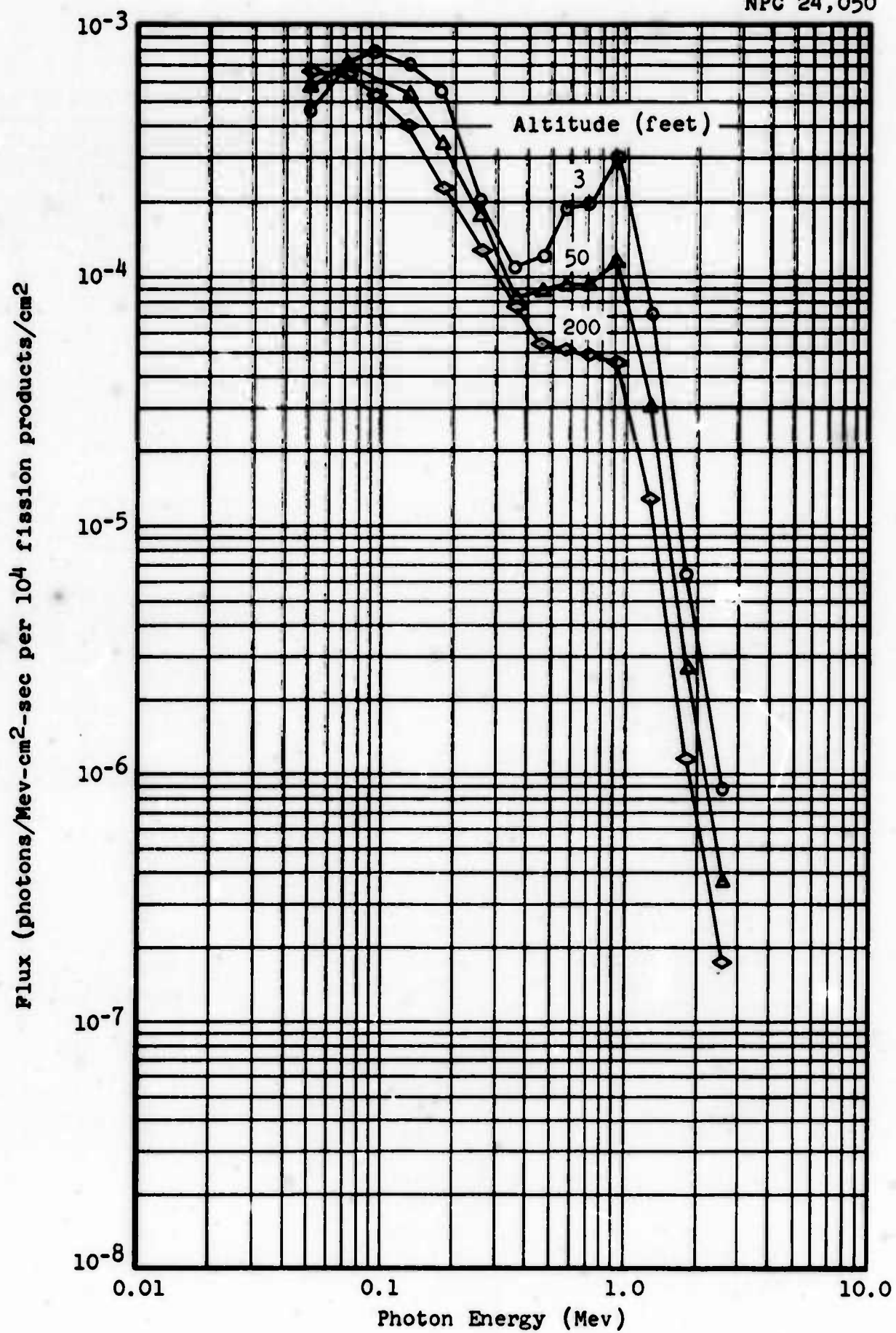
Figure 4.6 Number Spectra: Decay Time, 97.3 Days
