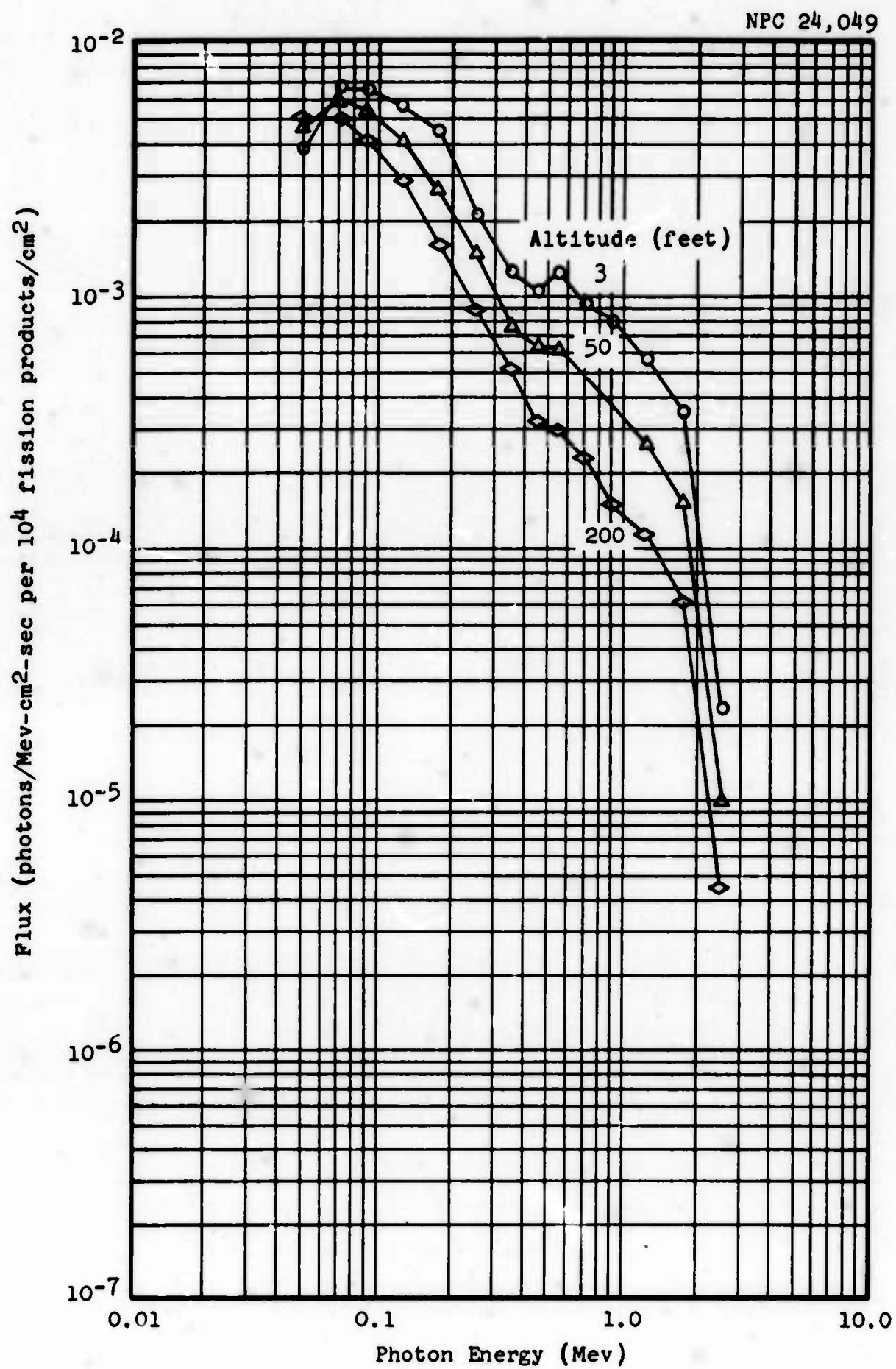
Figure 4.5 Number Spectra: Decay Time, 21.1 Days
