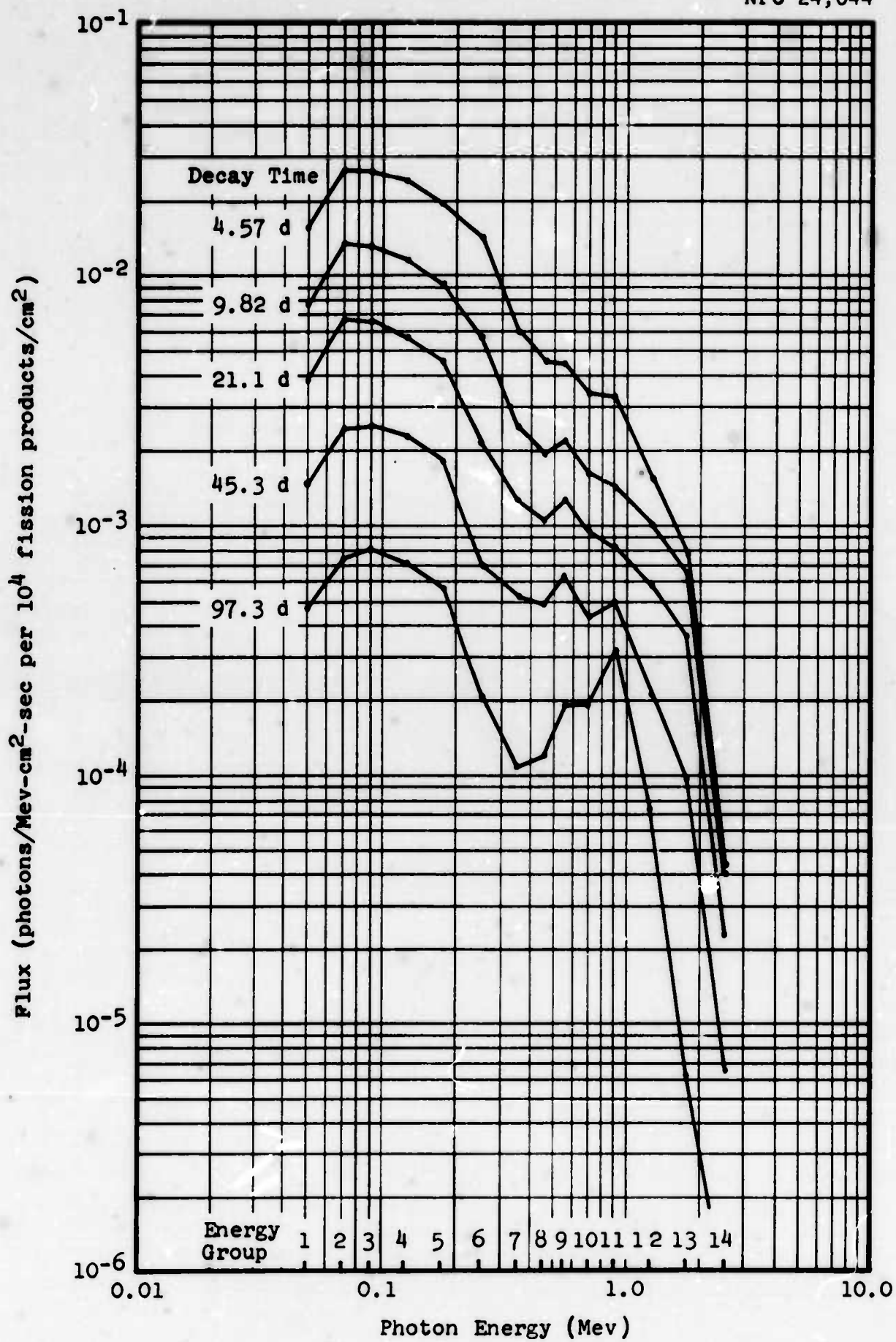
Figure 4.1 (cont'd) Number Spectra: Altitude, 3 Feet
