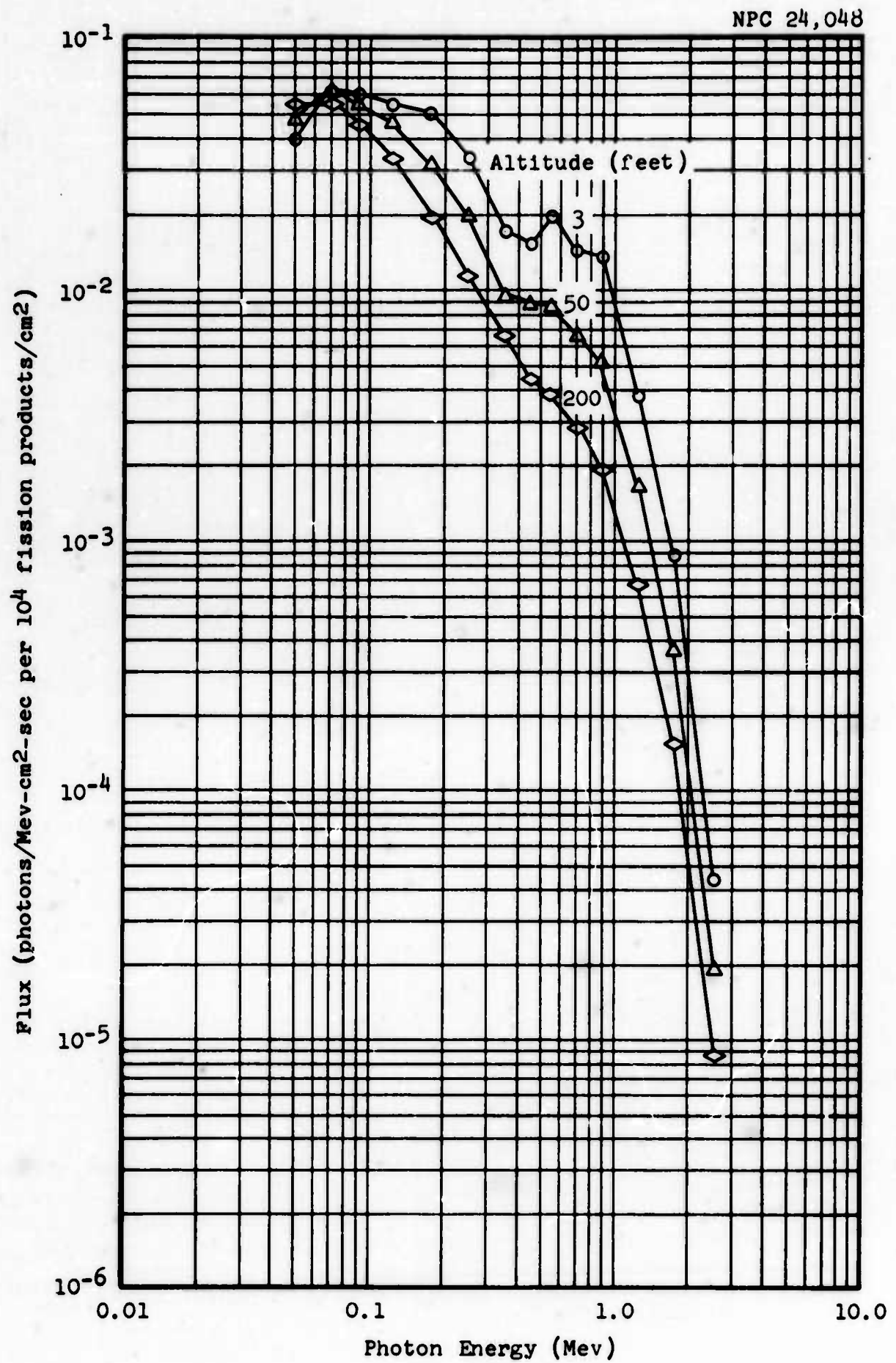
Figure 4.4 Number Spectra: Decay Time, 2.13 Days
