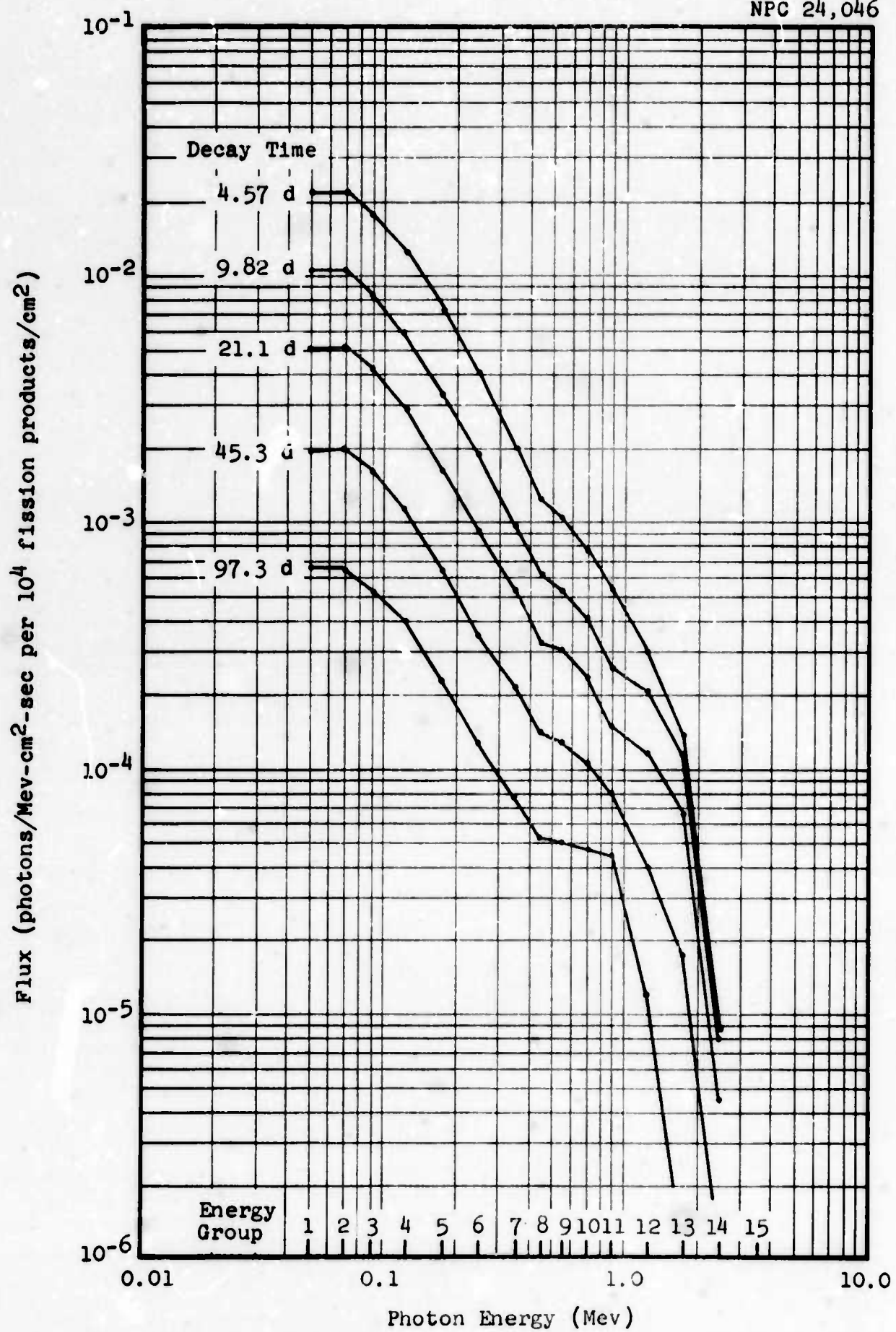
Figure 4.2 (cont'd) Number Spectra: Altitude, 200 Feet
