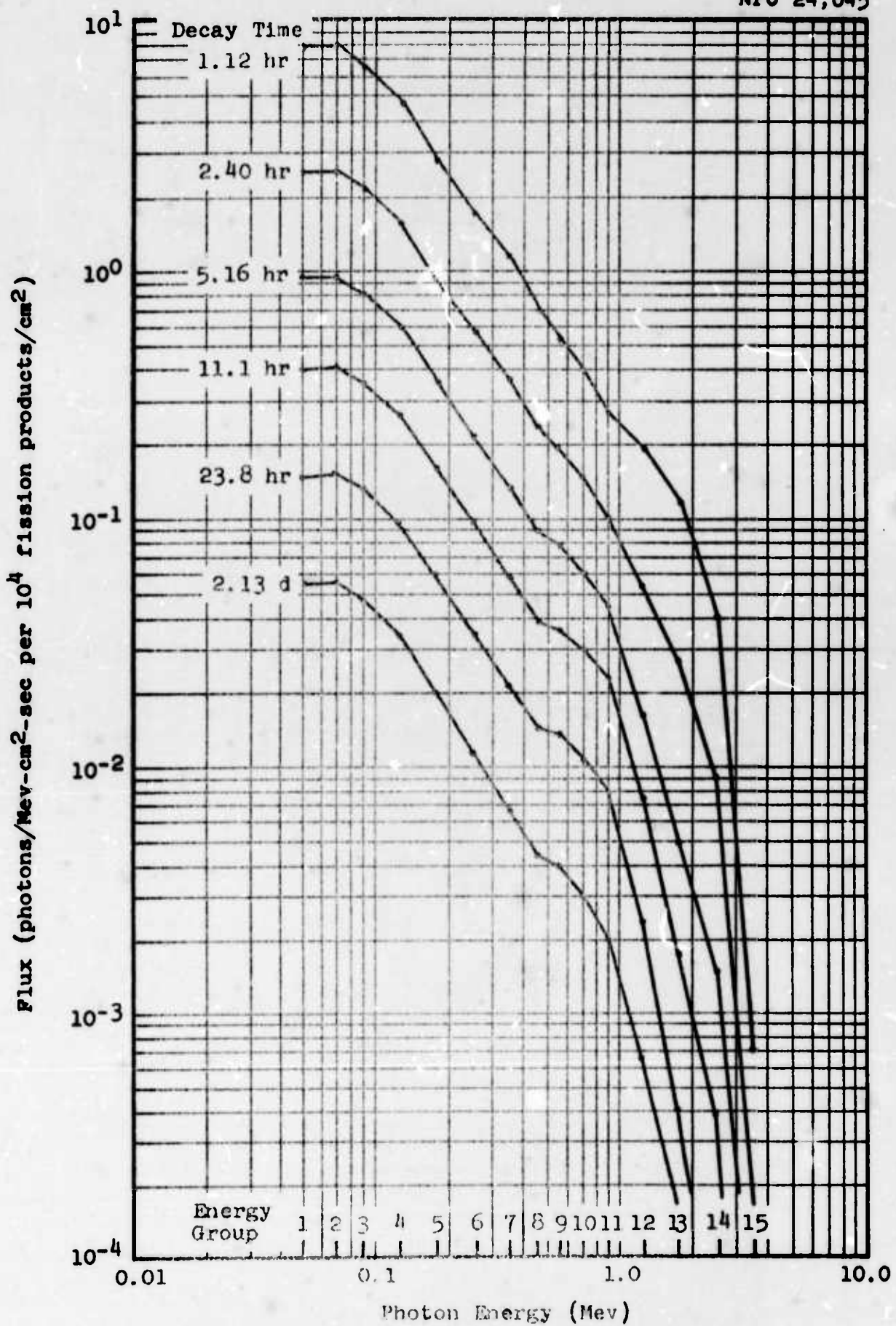
Figure 4.2 Number Spectra: Altitude, 200 Feet (figure continued on next page)
