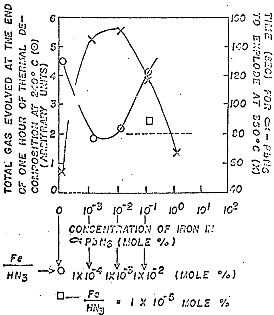
SENSITIVITY OF Cl-PbN 6 VS IRON DOPING
