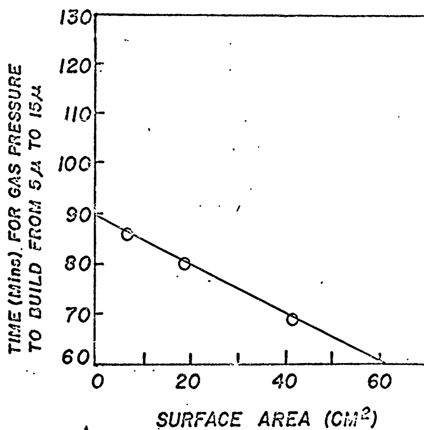
SENSITIVITY OF \text{Cr-PbN}_6 VS SURFACE AREA ( 240^\circ\text{C} )
