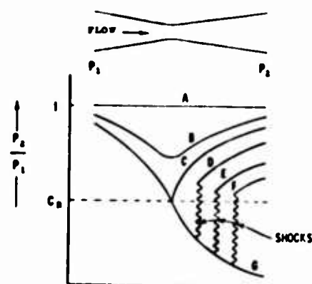
ONE-DIMENSIONAL COMPRESSIBLE FLOW IN A CONVERGENT-DIVERGENT PASSAGE
